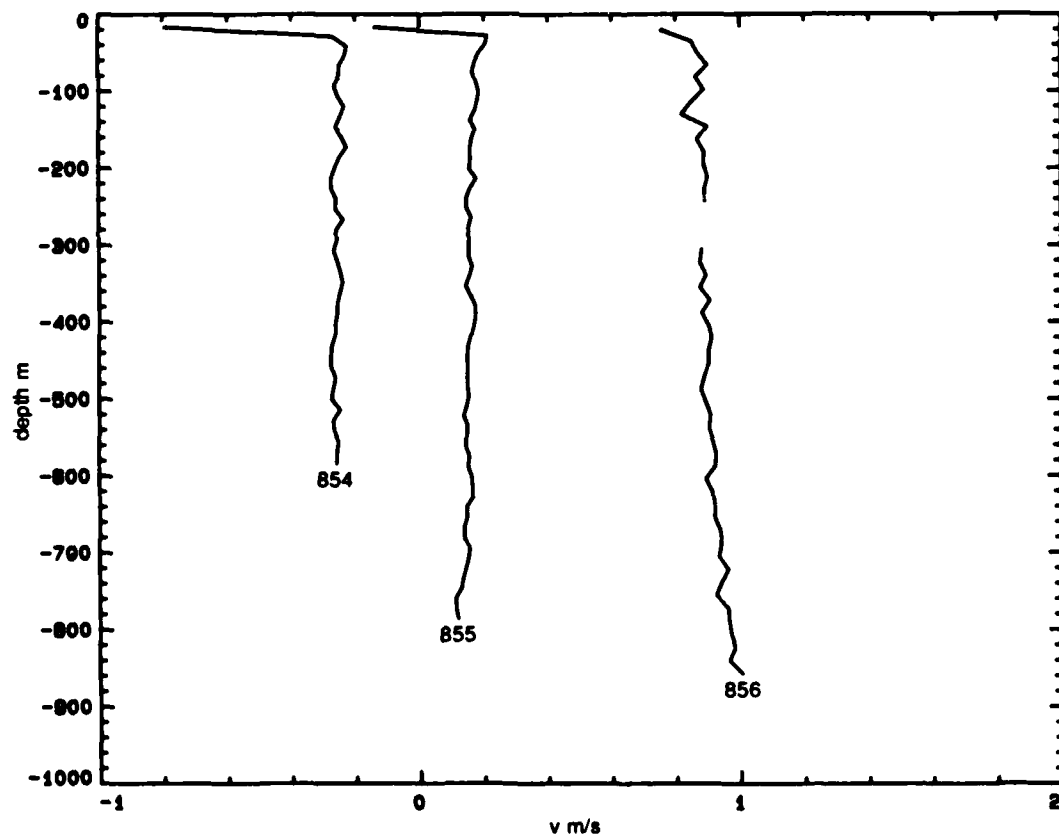
Figure 9. Shorted electrode probes' east (u) and north (v) velocities. These data are a measurement of the noise sensed by the probe.
