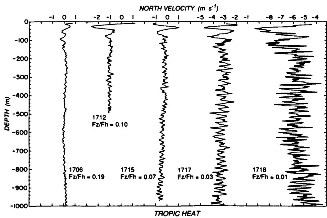
Figure 13b. Velocity comparisons at similar F_z/F_h ratios.
