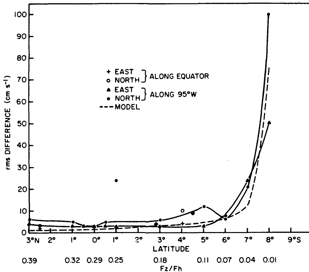
Figure 11. The rms differences between XCP and TOPS. The dashed line is the model prediction. The values of F_z/F_h for the drops in the 95°W section are shown below the corresponding latitude.
