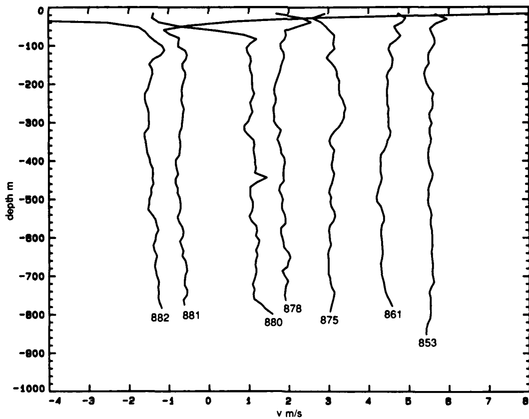
Figure 8b. XCP east ( u ) and north ( v ) velocity sections. Velocities are in magnetic components.
