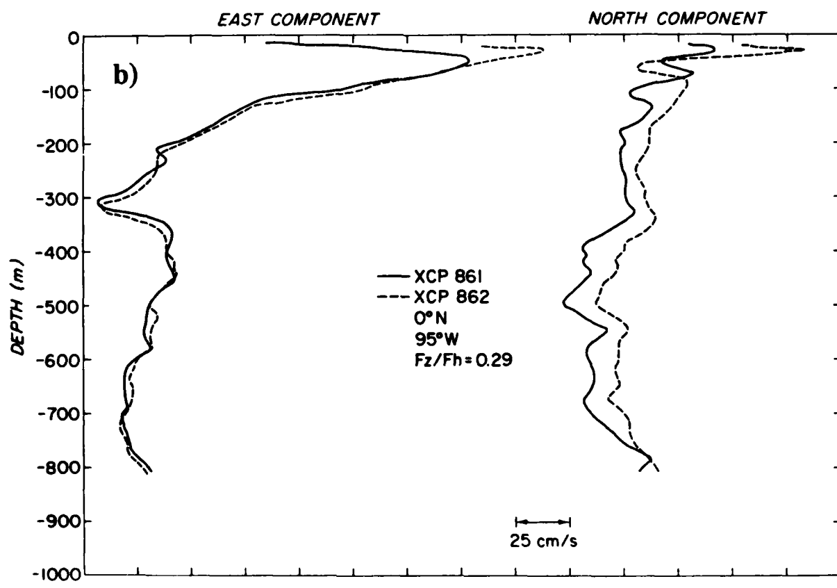
Figure 4a-c. XCP/XCP velocity comparisons. Velocities are in magnetic components.
