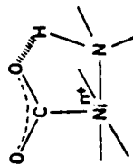
Figure 1. Proposed binding of CO 2 to nickelacyl 20 . 32
