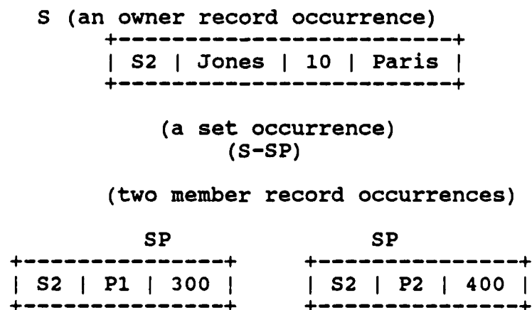
Figure 4. A CODASYL Set Occurrence
