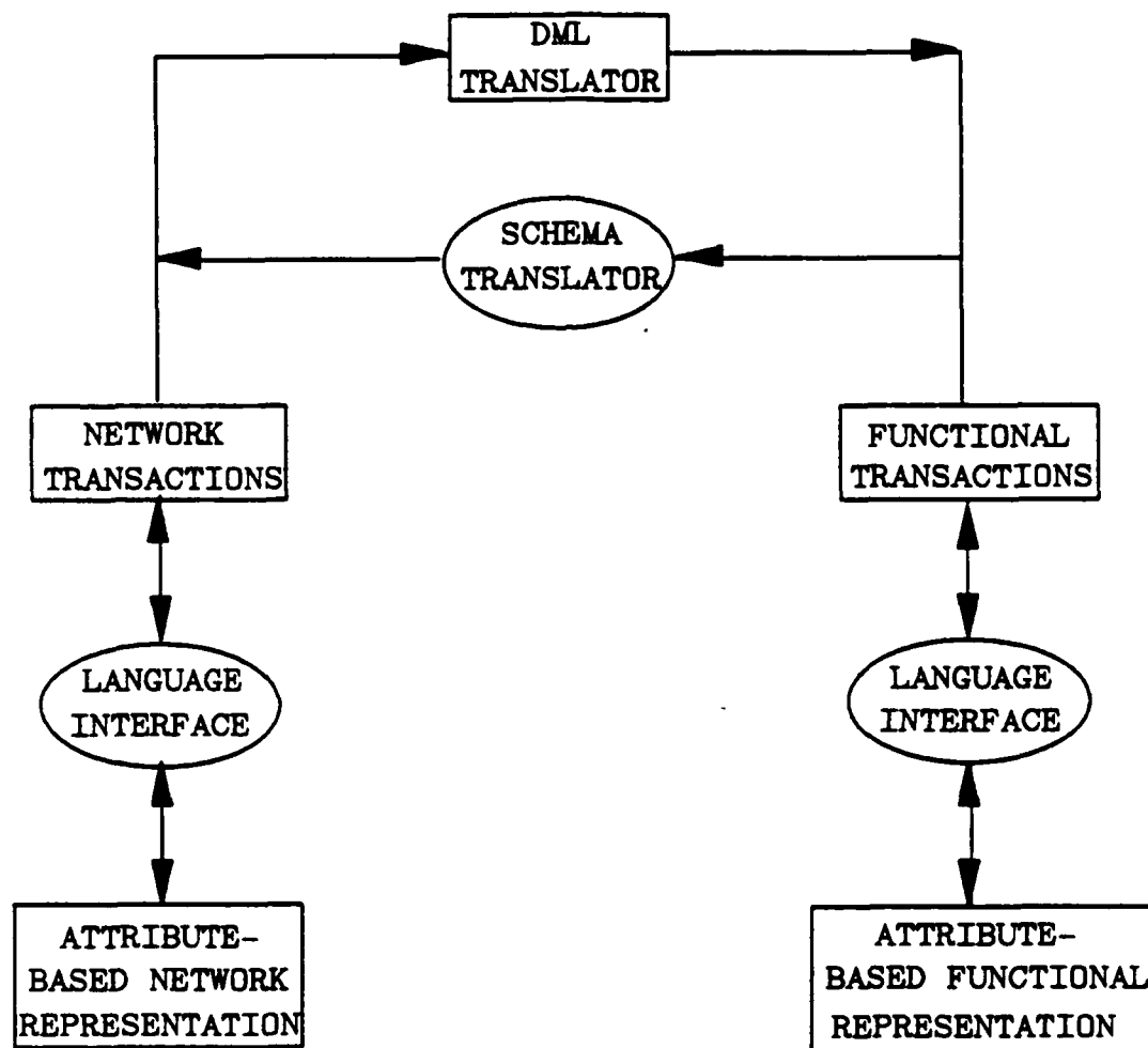
Figure 11. The High-Level Preprocessing Approach
