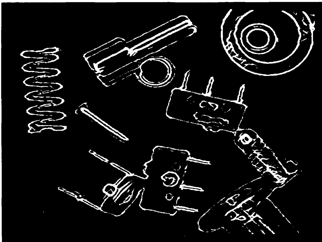
Fig. 15-b. Edgel Image - Our Detector ( \tanh, \sigma_{\text{blur}} = 0.6 )
