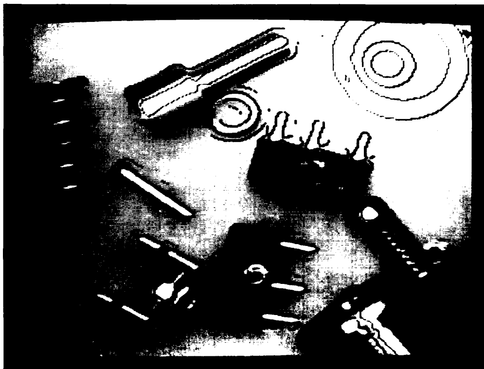
Fig. 15-g. Superimposed Image - Marr-Hildreth Operator
