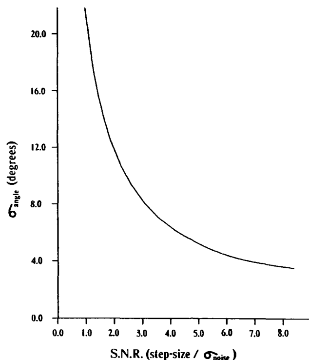
Fig. 10. Plot of the standard deviation of the angular error in the true positives detected with threshold = 0, vs the S.N.R..
