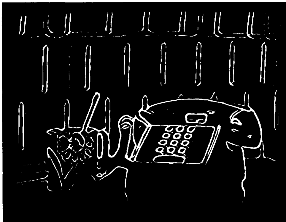
Fig. 14-b. Indoor Scene : Edgel Image (tanh)
