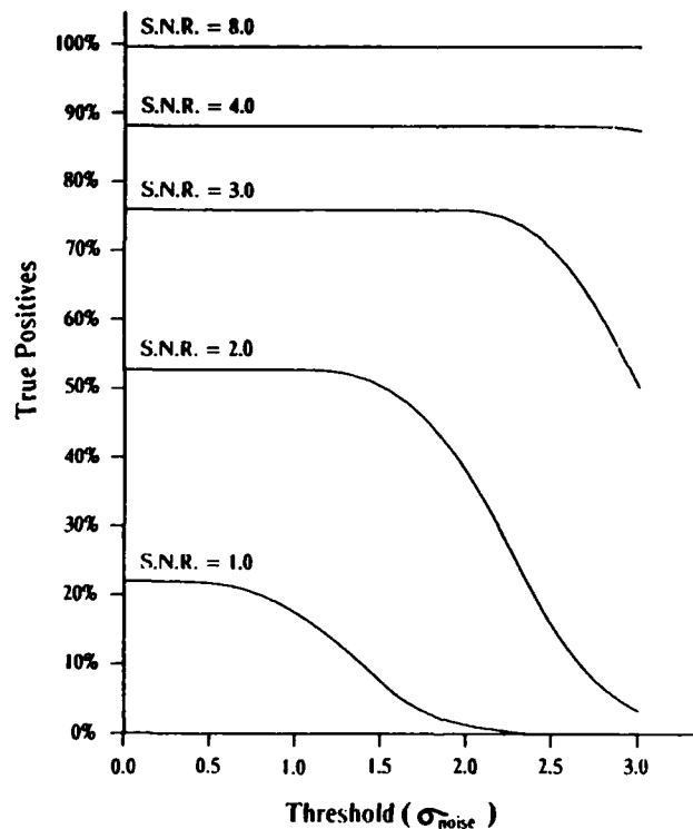
Fig. 9. Plot of true positives detected in windows with synthesized step-edges and additive white Gaussian noise, as a function of the threshold for different S.N.R.'s.
