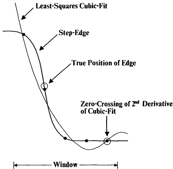
Fig. 2. Inadequacy of the cubic-fit for a step-edge cross-section which is positioned near the edge of a window.
