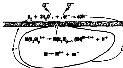
Figure 3. Schematic diagram of pitting initiation.
