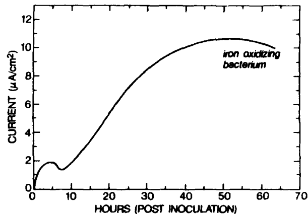
Figure 2. Corrosion current vs. time resulting from colonization of carbon steel.
