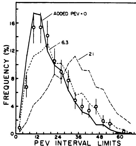
Fig. 5. The frequency distributions (in percent) of maximum PEV's resulting from correlations of the solar flux with real and fictitious winds. The real wind PEV distribution and its approximate 68% confidence limits are denoted by the circles and vertical lines, respectively. The fictitious wind series distributions are denoted by the solid and broken lines. The PEV of each ensemble of fictitious wind series, due to the addition of a fraction of the solar flux, is indicated.
