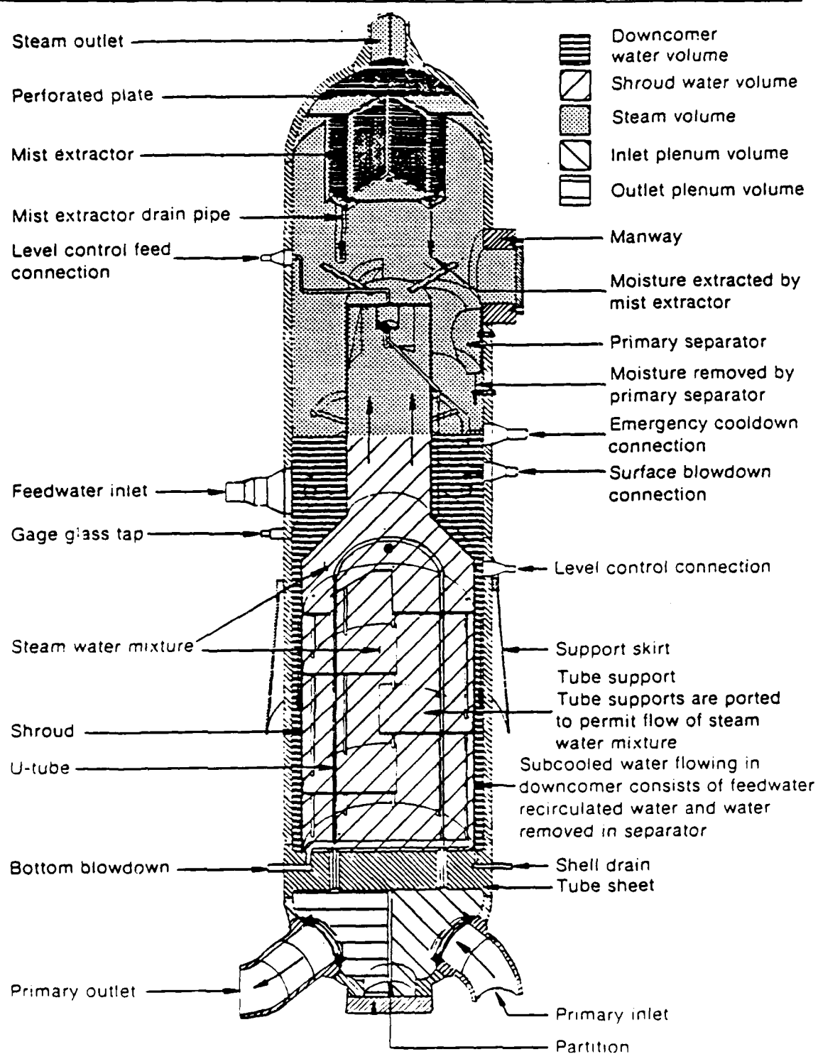
Figure 7: LOFT Facility Intact Loop Steam Generator
