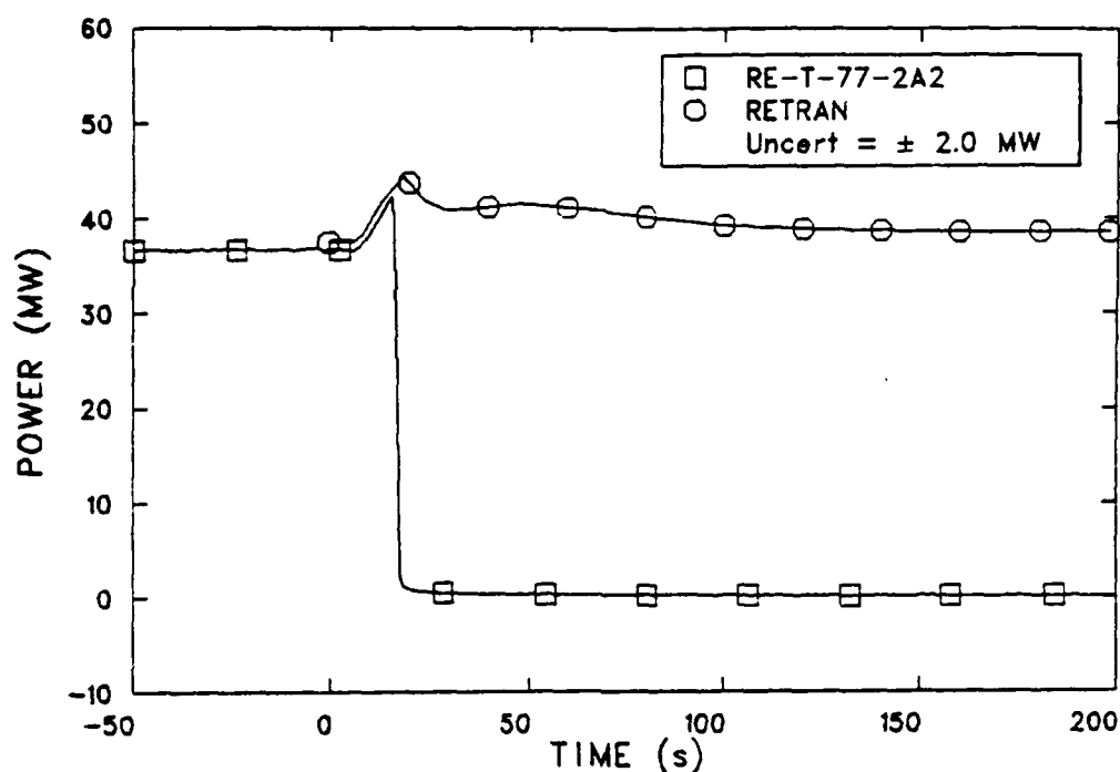
Figure 23: Experiment L6-3: Reactor Power
