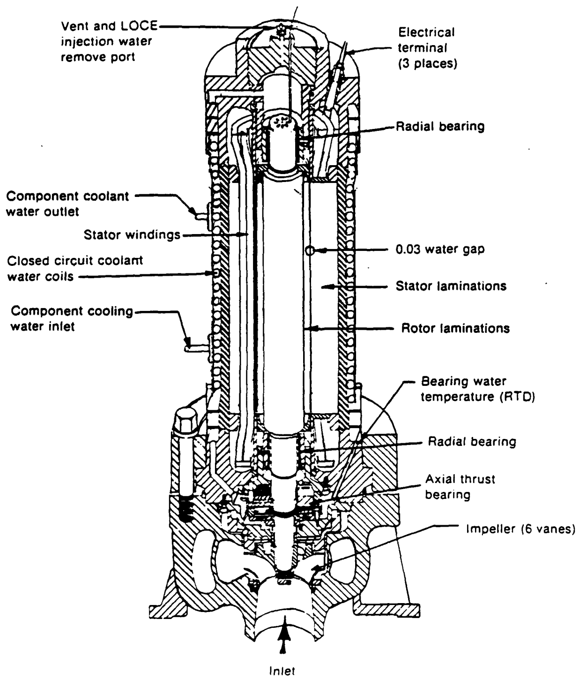
Figure 8: LOFT Facility Reactor Coolant Pump
