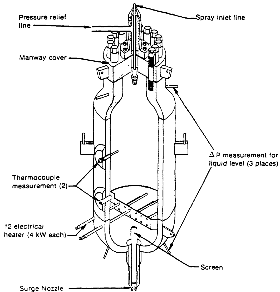
Figure 6: LOFT Facility Pressurizer
