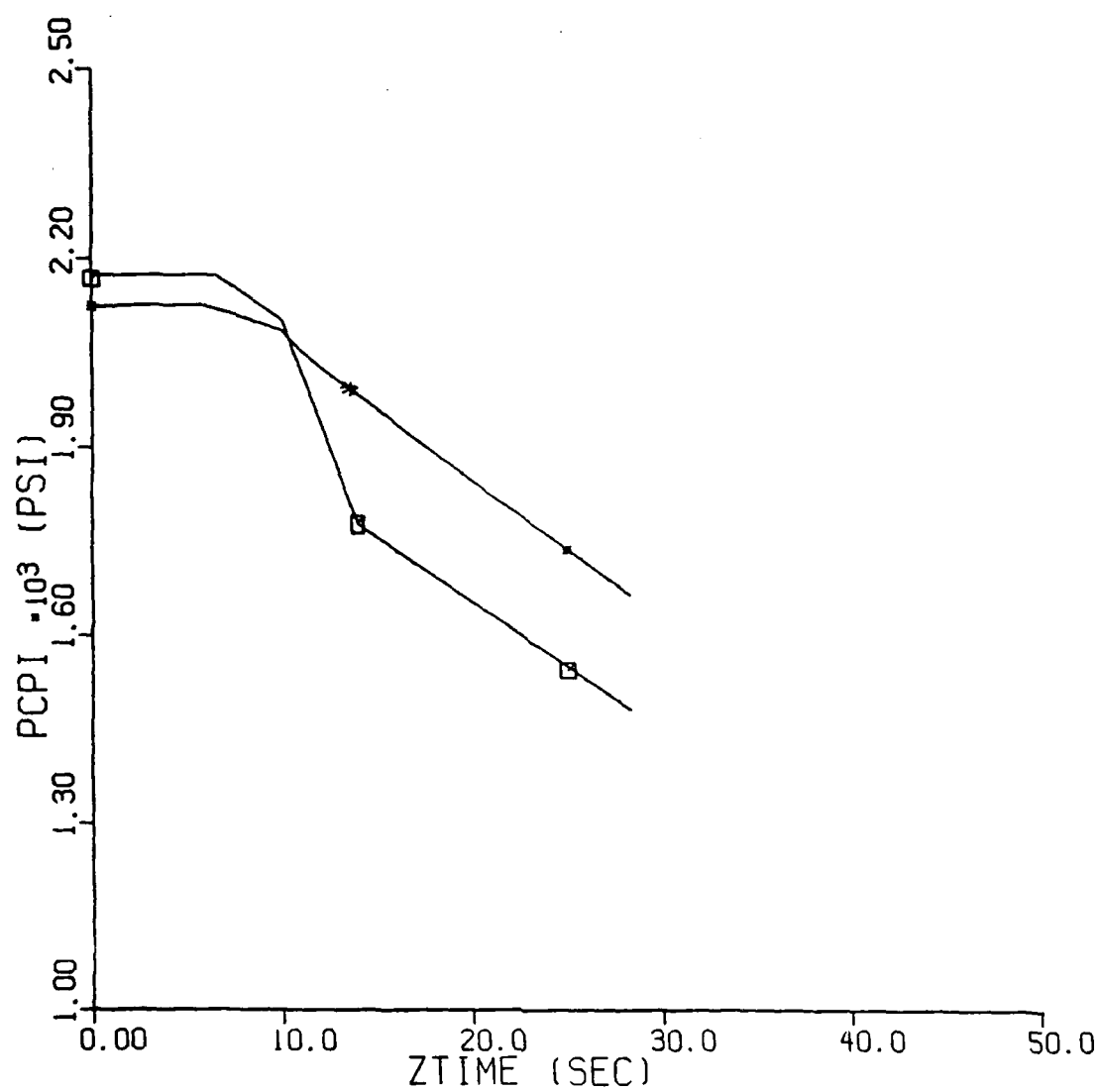
Figure 27: L3-5 Predicted Performance: Primary System Pressure
