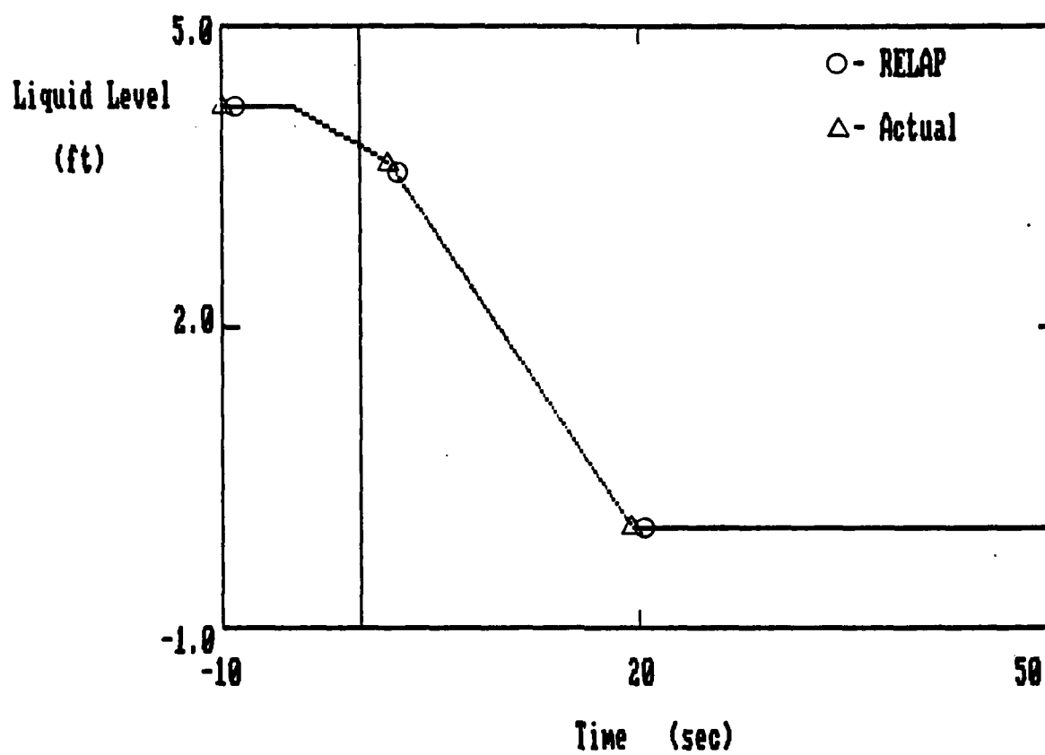
Figure 21: Experiment L3-5: Pressurizer Level
