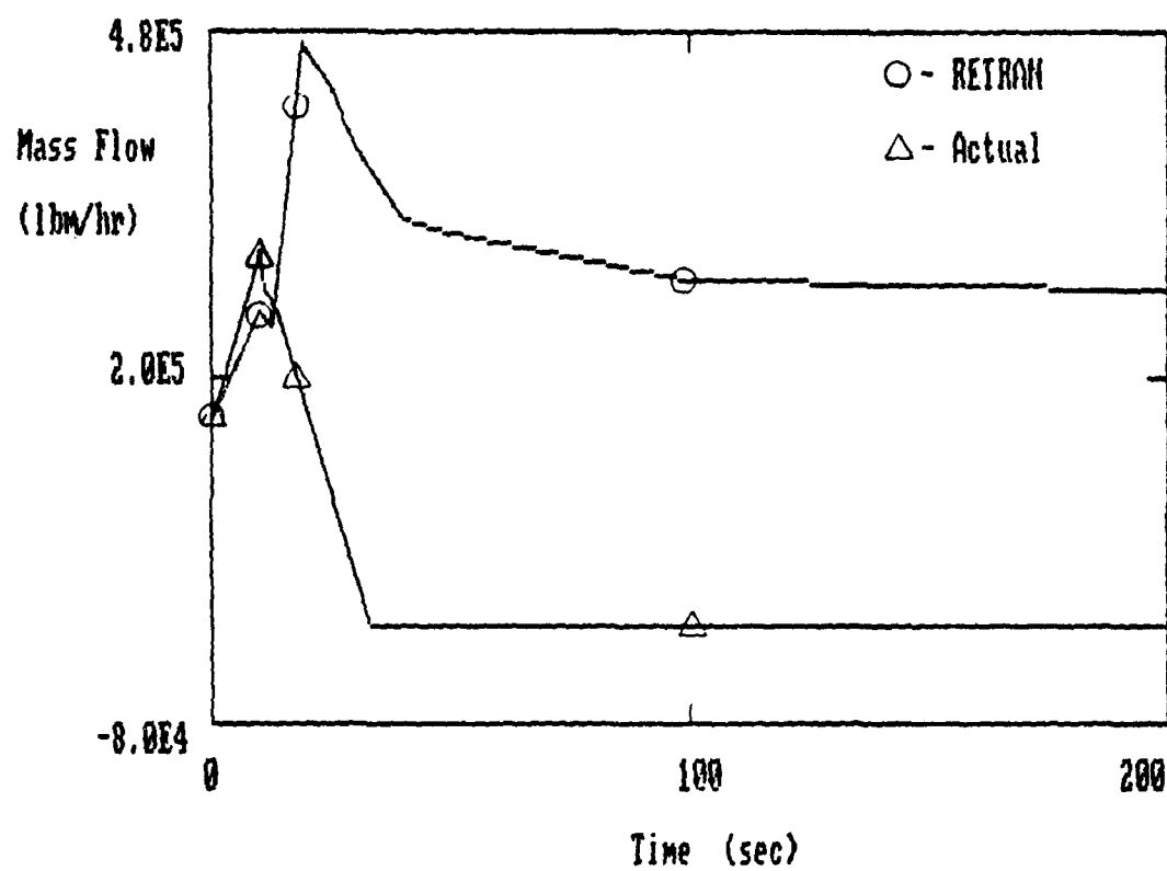
Figure 22: Experiment L6-3: Steam Demand
