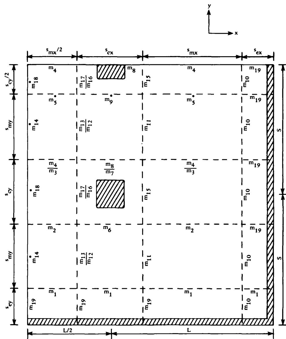
Figure A-9. Unit moment distribution for 3 x 4 flat slab.
