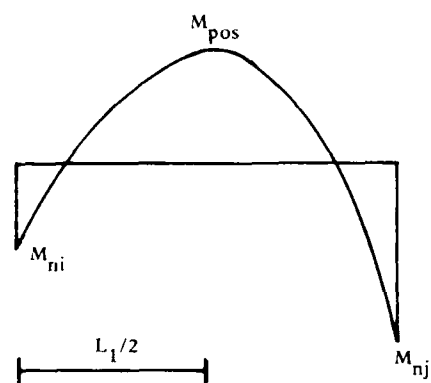
(a) Moment diagram referring to centerline of supports.
