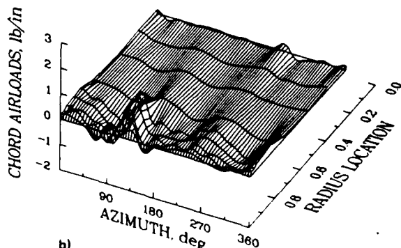
Figure 5. Chord airloads derived from measured normal force; drag on airfoil is a negative load. a) 0-10 harmonics. b) 3-10 harmonics.
