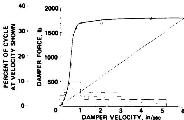
Figure 18. Calculated damper velocity histogram; linear damping rate of 300 lb-sec/in. shown as dashed line.
