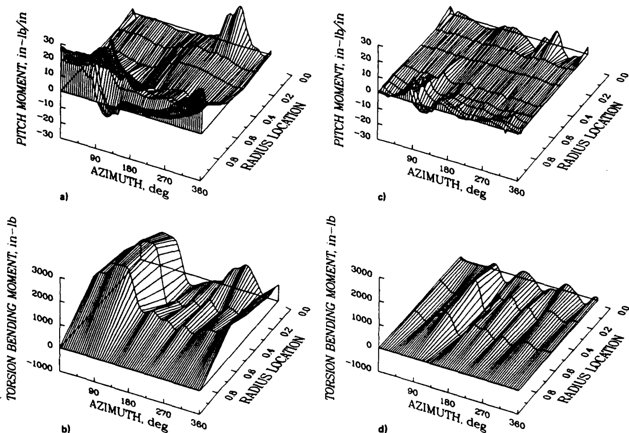
Figure 3. Cartesian plots of CH-34 wind tunnel pitching moment and torsional-moment data; V = 150 knots, shaft angle = -5^\circ . a) Pitching moment; 0-36 harmonics. b) Torsional moment; 0-10 harmonics. c) Pitching moment; 3-36 harmonics. d) Torsional moment; 3-10 harmonics.
