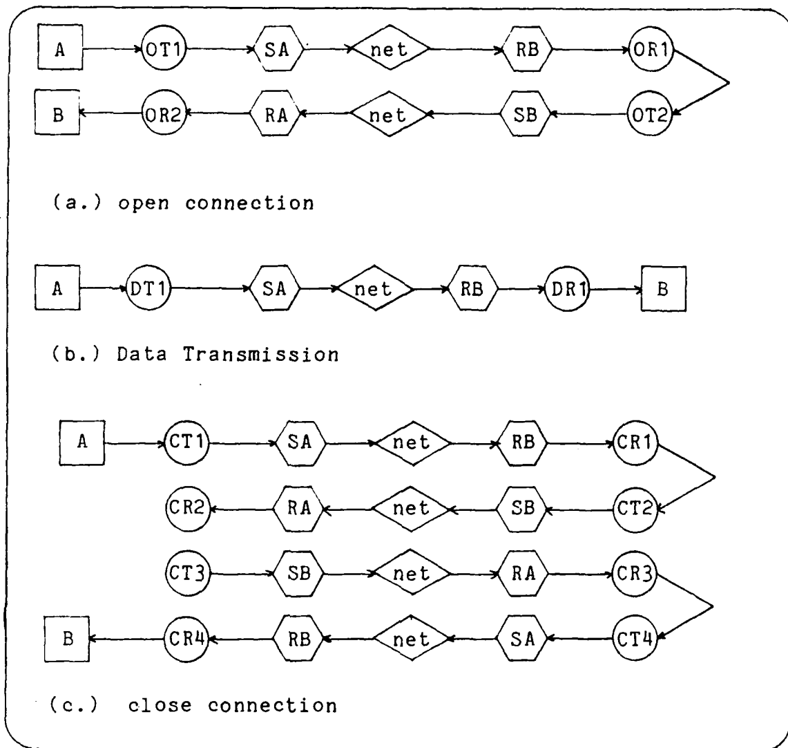
Figure 9. Queueing Chains
