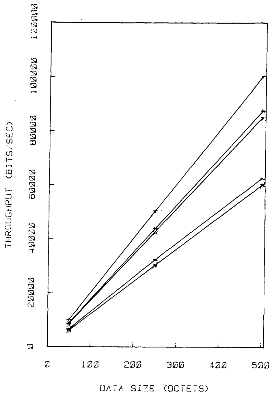
Figure 14. Throughput Summary
