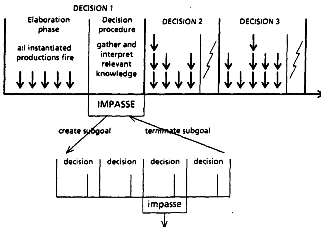
Figure 5-1: The SOAR Decision Cycle
