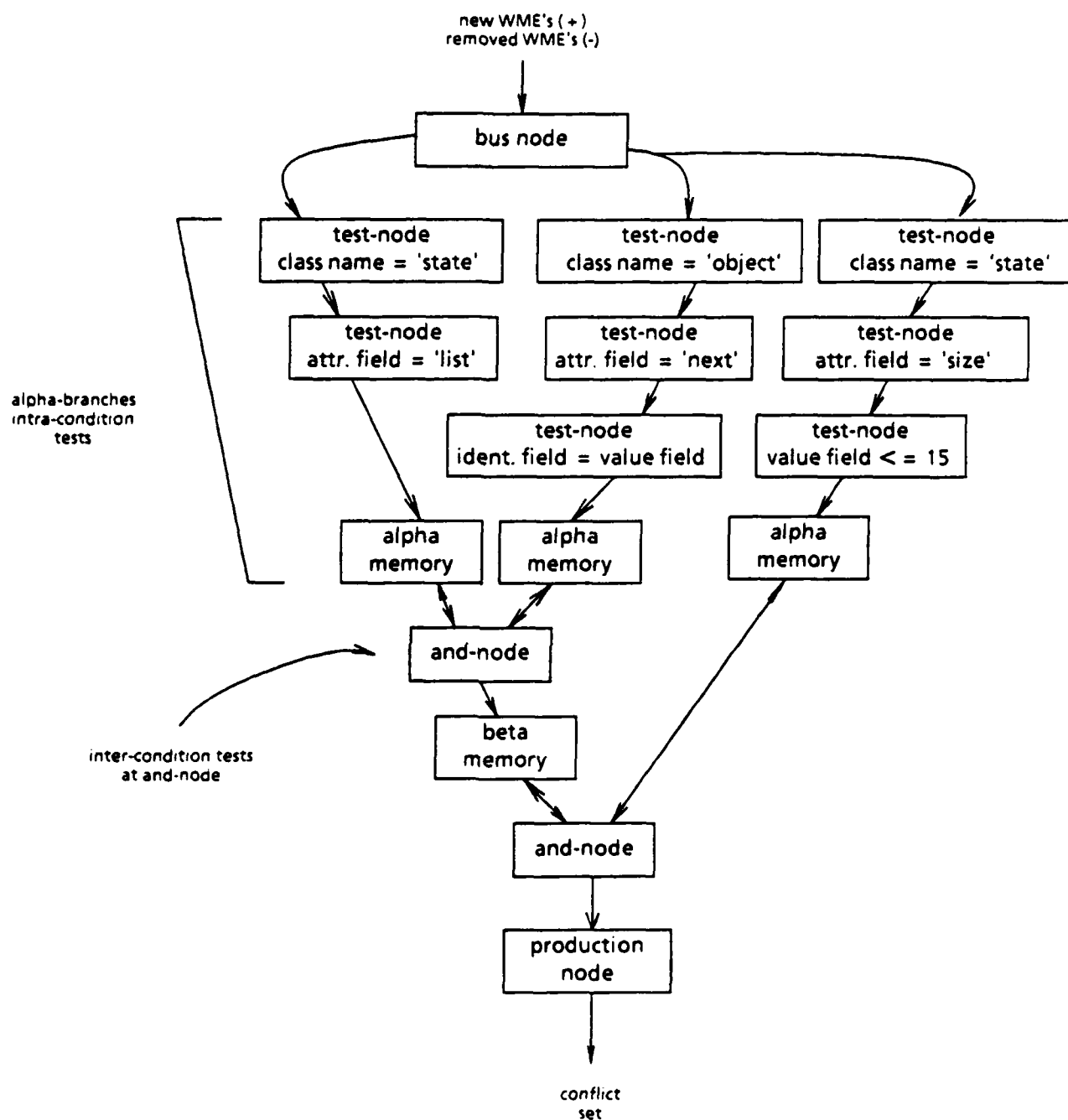
Figure 4-1: Structure of a Small Rete Network
