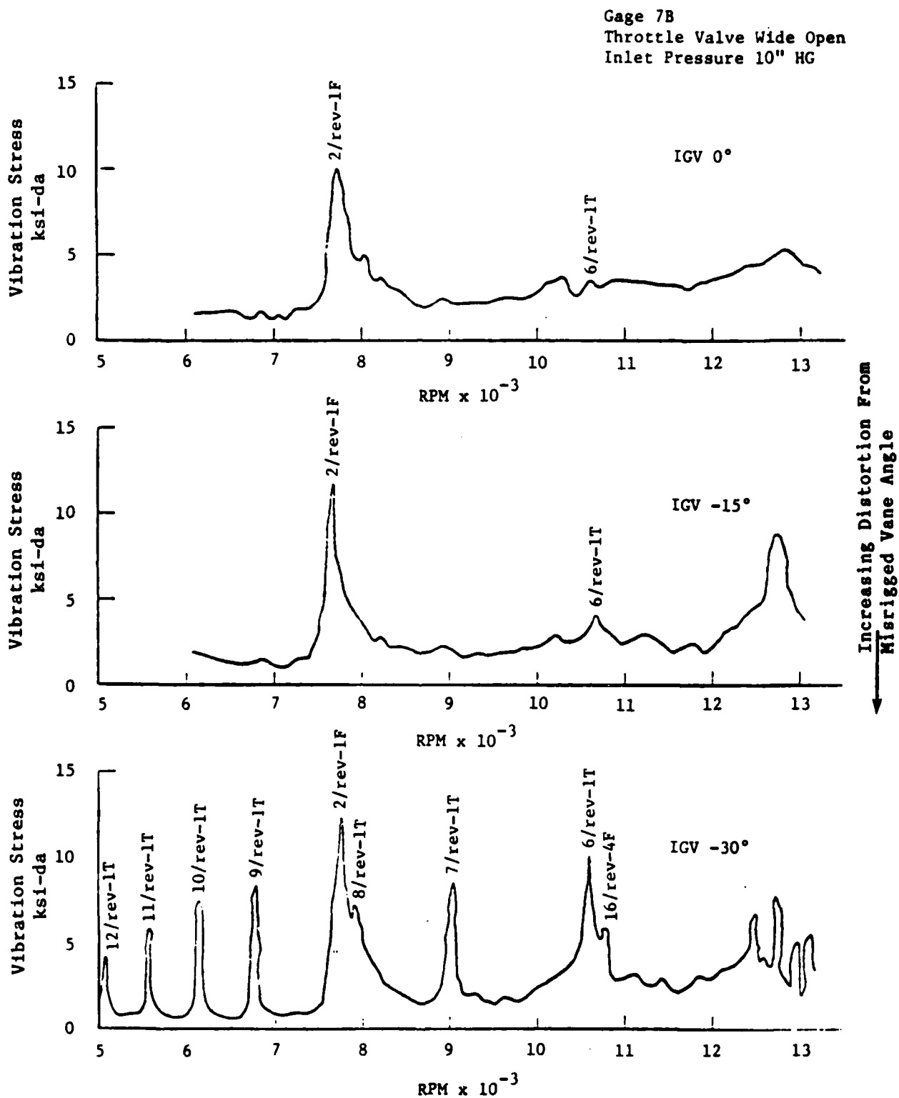
Figure 3. Effect of Single Off-Angle IGV on Rotor Blade Resonant Stress.
