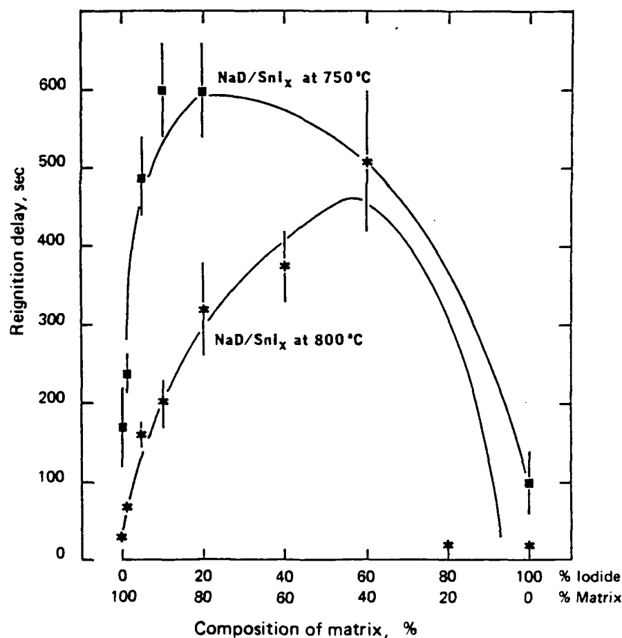
Figure 28. The Synergistic Effect Seen in Fire Control Properties for Sodium Dawsonite Doped With Tin Iodide at Various Temperatures.
