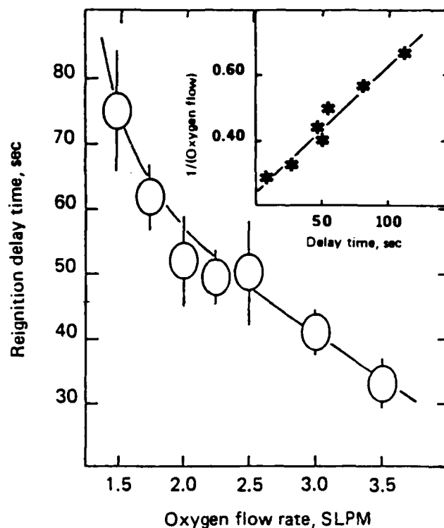
Figure 18. Dependence of the Reignition Delay Time for Commercially Supplied Potassium Bicarbonate Extinguishant as a Function of the Oxygen Partial Pressure Above the Heated Plate Surface (Measured in Terms of the Oxygen Flow Rate Into the Vapor Space Above the Heated Plate).
