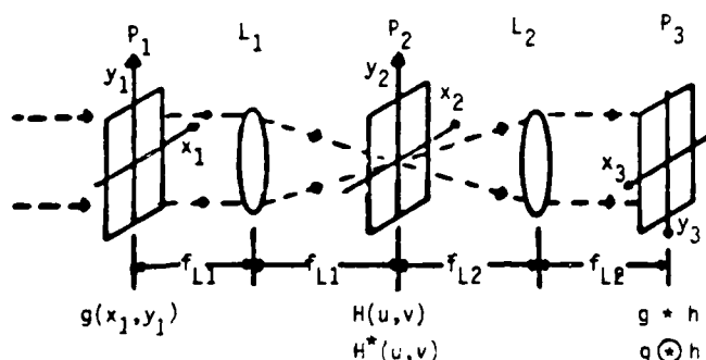
FIGURE 1 Conventional optical Fourier transform and frequency plane correlator
