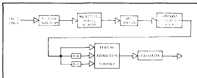
Fig. 1. General Fourier transform (etc.) feature-extraction pattern recognition system block diagram.
