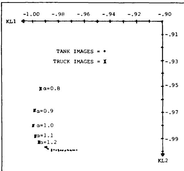
Fig. 2. Magnitude-only WRD Fourier transform features projected onto dominant tank/truck eigenvectors (for 25-image data base). KL1 = dominant truck eigenvector; KL2 = dominant tank eigenvector.
