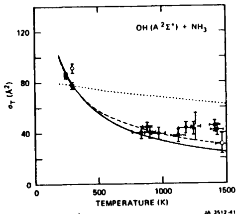
Figure 1. Temperature dependence of the cross section for quenching of ( A^2\Sigma^+ , v'=0 ) OH by NH_3 . Solid symbols are the present LP/LF ( \circ ) and flow reactor ( \blacksquare ) measurements. The open squares are the previous LP/LF results (Ref. 5) and the open circle, the rotationally and thermally averaged value as computed from the state-specific cross sections (Ref. 4). The lines are calculated values, all normalized to the experimental value at 300K.
