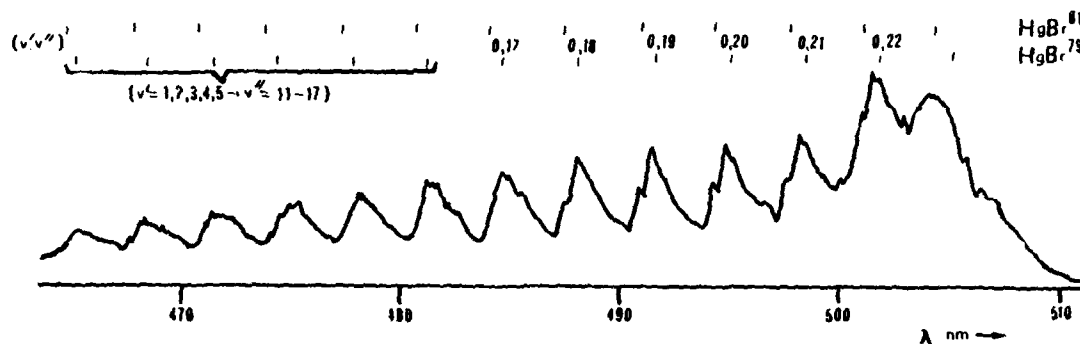
Figure 1: Emission band B^2\Sigma \rightarrow X^2\Sigma of \text{HgBr} from the KrF laser photolysis of \text{HgBr}_2 vapor and 675 torr of Ar; cell temperature is 100^\circ\text{C} .
