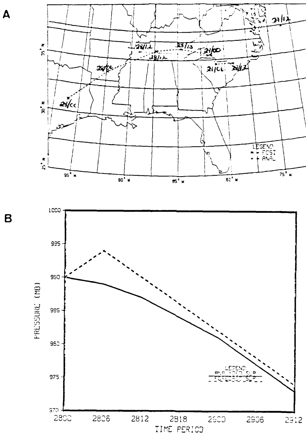
Fig. 3.1 (A) NORAPS analyzed (dotted) and forecast (dashed) surface low track for 28-29 March 1984. (B) NORAPS analyzed (solid) and forecast (dashed) sea-level pressure (mb) for low center above. Times are specified by date (first two digits) and hours (second two digits) in Greenwich Mean Time.
