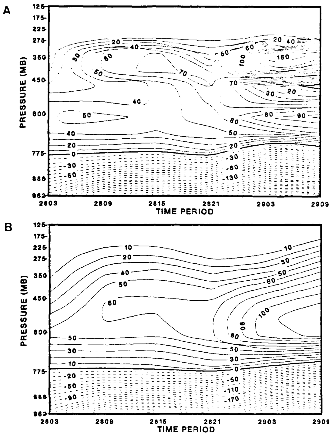
Fig. C.5 Vertical moisture flux for radius 4 in the (A) old forecast and in the (B) new forecast. Contour interval is 10 \times 10^{-4} g/g/day.
