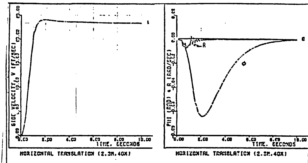
Fig. 5-1 Time Domain Response Functions used to Generate System Specifications (2:52)
