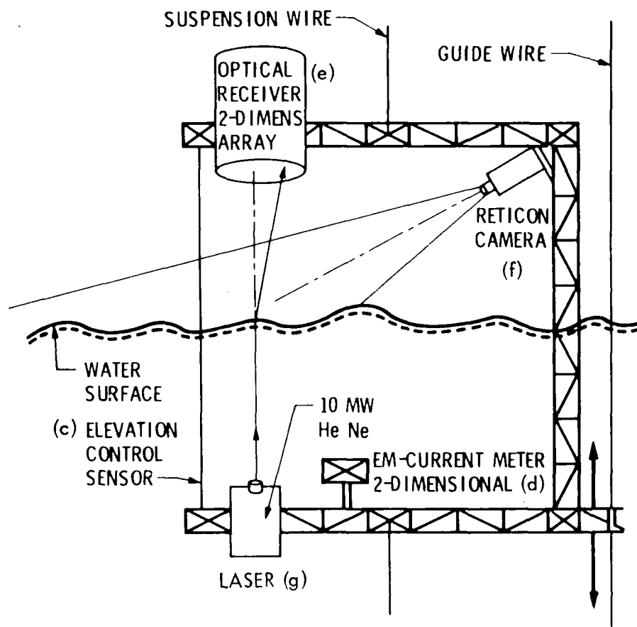
Figure 3. Wave Follower Instrument Frame. Capacitance Gage is used as Elevation Control Sensor (c); Two-dimensional current meter is used for measuring two horizontal currents components below water surface (d); Optical Receiver records two slope components of surface normal (e); Reticon camera records vertical displacement of water surface (f) and using He-Ne Laser (g).
