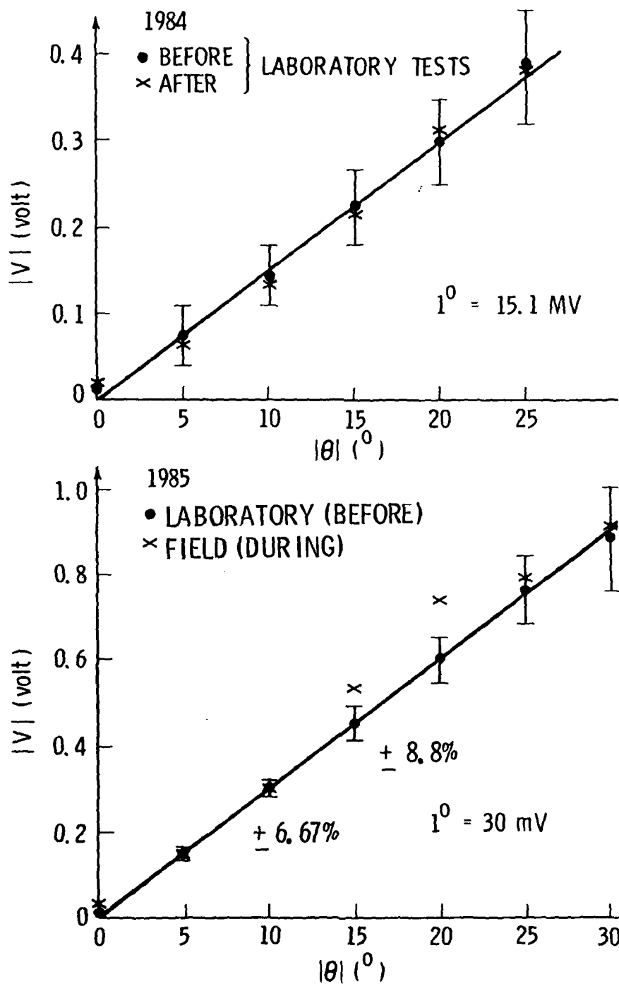
Figure 5. Calibration of Wave Slope Instrument.
