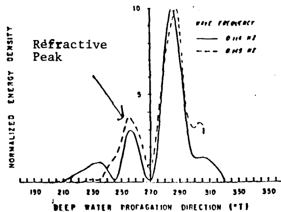
Figure 3. Measured directional spectra at Torrey Pines Beach (refracted into local deep water) for 10 sample days in March 1977. The data runs have a cumulative length of roughly 64 hours [Pawka, 1983].
