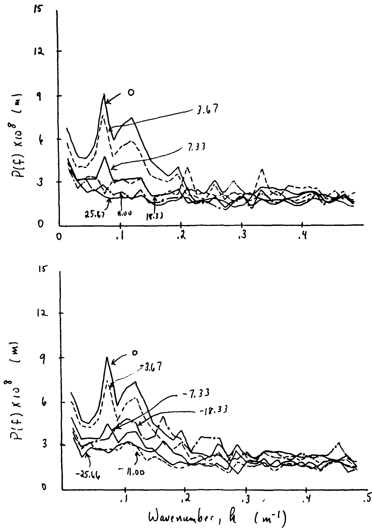
Figure 4. Effect of Focus on Simulated Image - \vec{V} \cdot \vec{k} = \cos(-142^\circ) , Leg No. 7, 10/31/84, Single- Look, N = 36 , V/R = 0.015 \text{ Hz} , T = 2.6 \text{ sec} .
