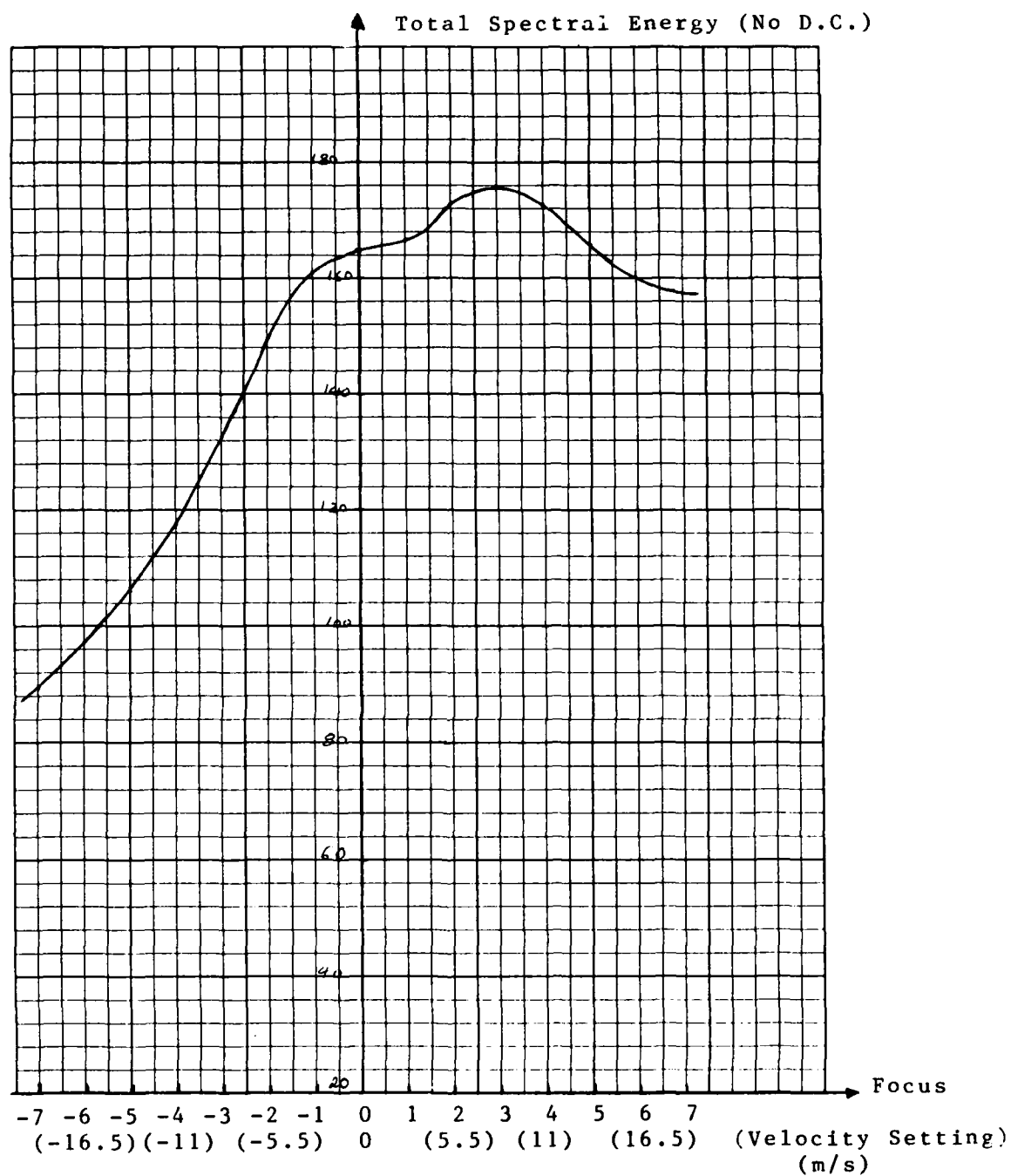
Figure 10. Total Spectral Energy vs. Focus (Range=128, I\Delta=15 ).
