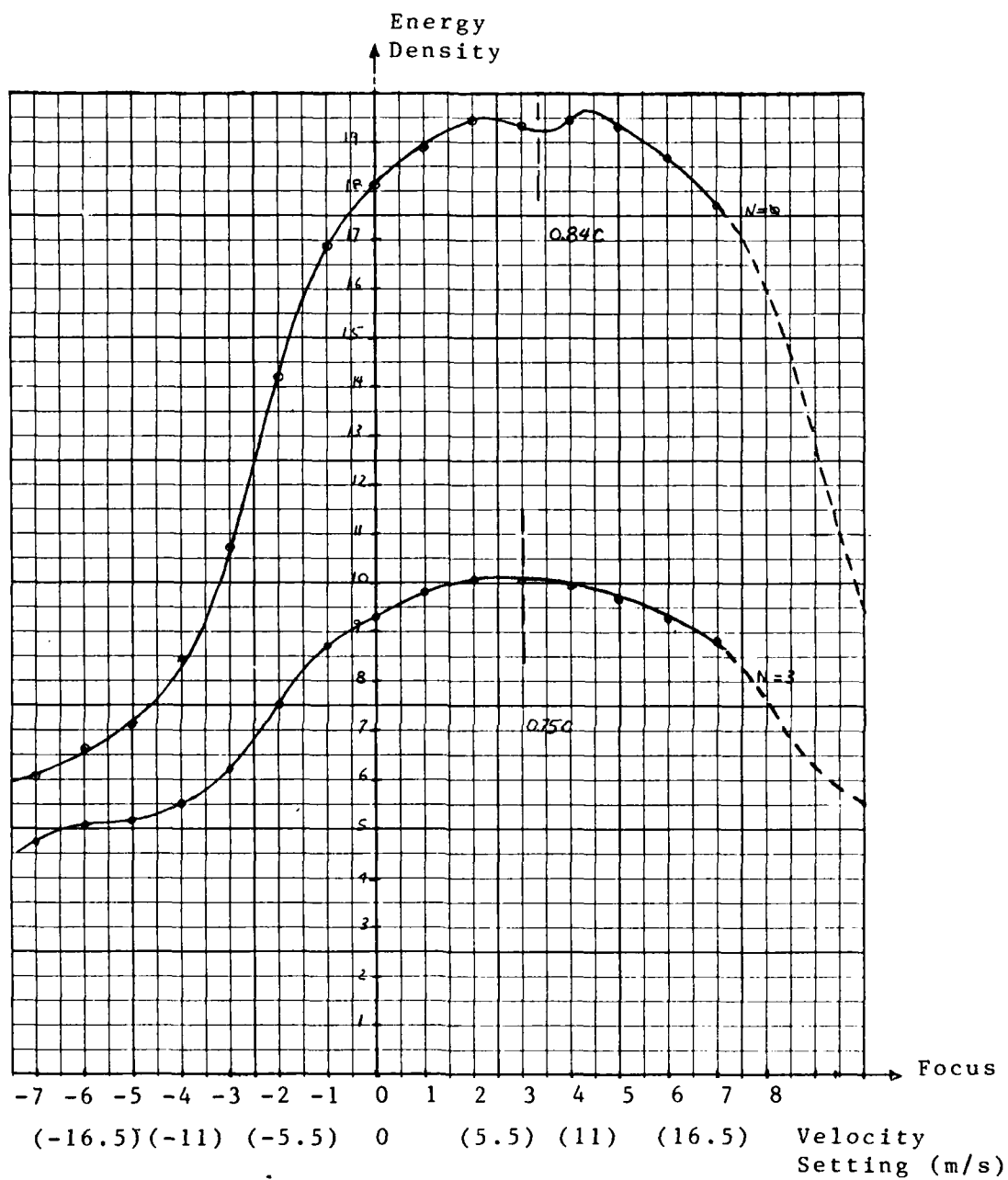
Figure 7. Energy Density at \lambda=140\text{m} vs. focus; \theta_i = 34.9^\circ .
