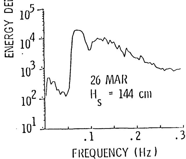
Figure 8c. Wave Height Spectra for Eight Overflight Days in Phase-11. (Continued)
