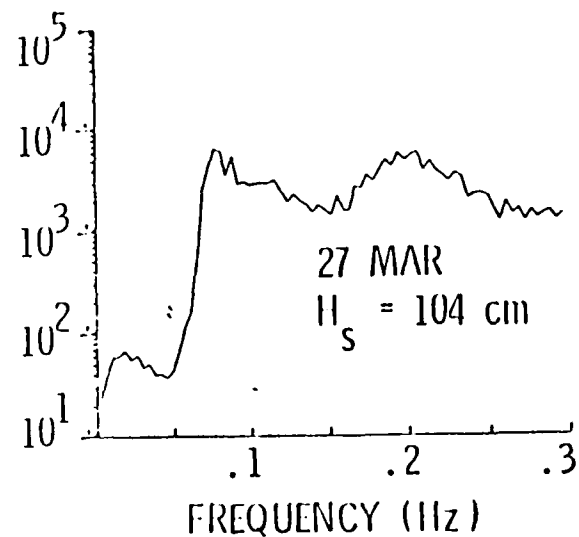
Figure 8c. Wave Height Spectra for Eight Overflight Days in Phase-11. (Continued)
