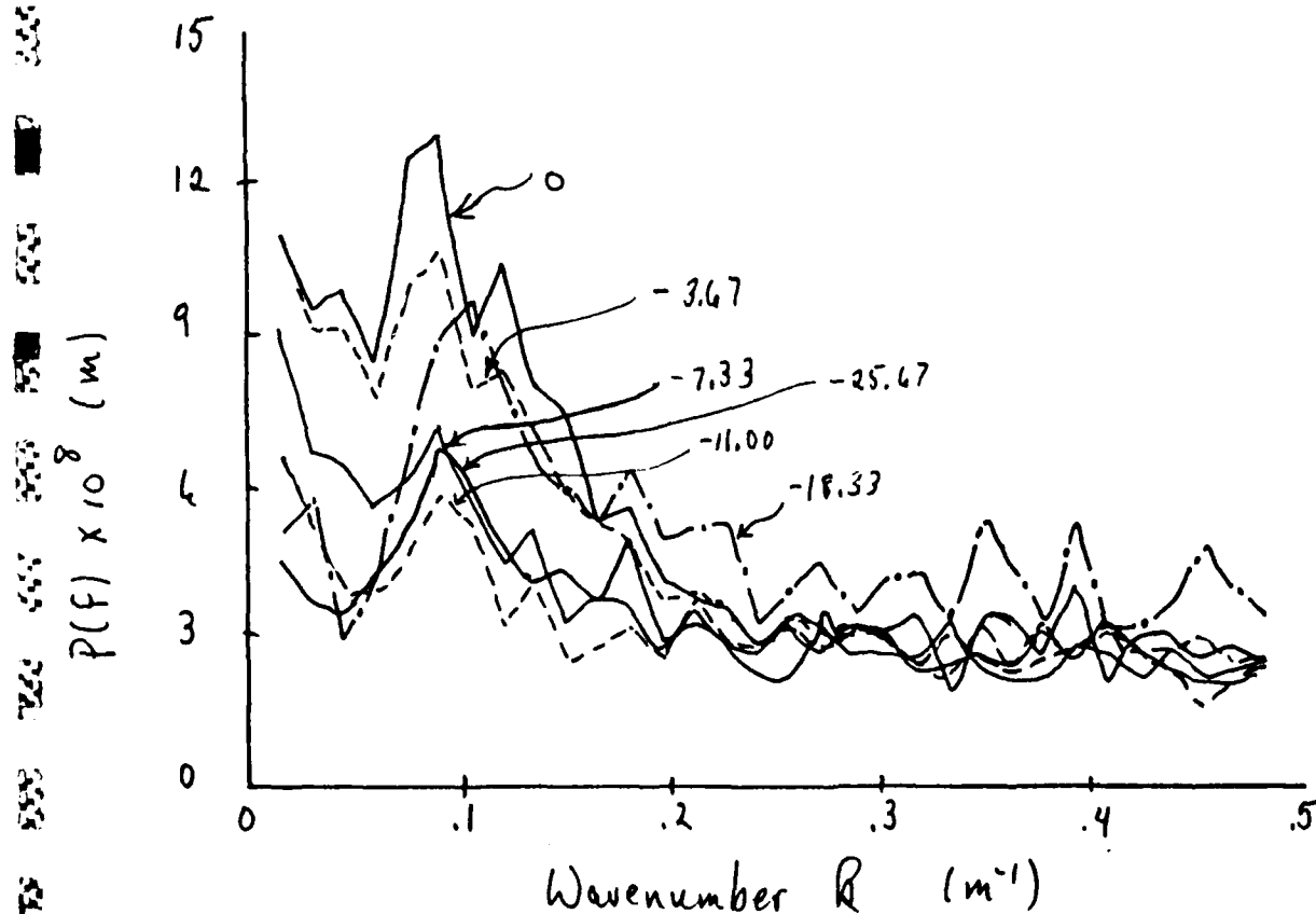
Figure 3. Effect of Focus on Simulated Image- \vec{V} \cdot \vec{k} = \cos(158^\circ) , Leg No. 4, 10/31/84, Single- Look, N = 29 , V/R = 0.015 \text{ Hz} , T = 2.6 \text{ sec} .
