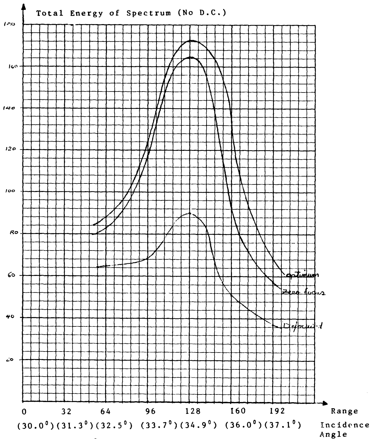
Figure 9. Total Spectrum Energy vs. Range ( I\Delta=15 ).
