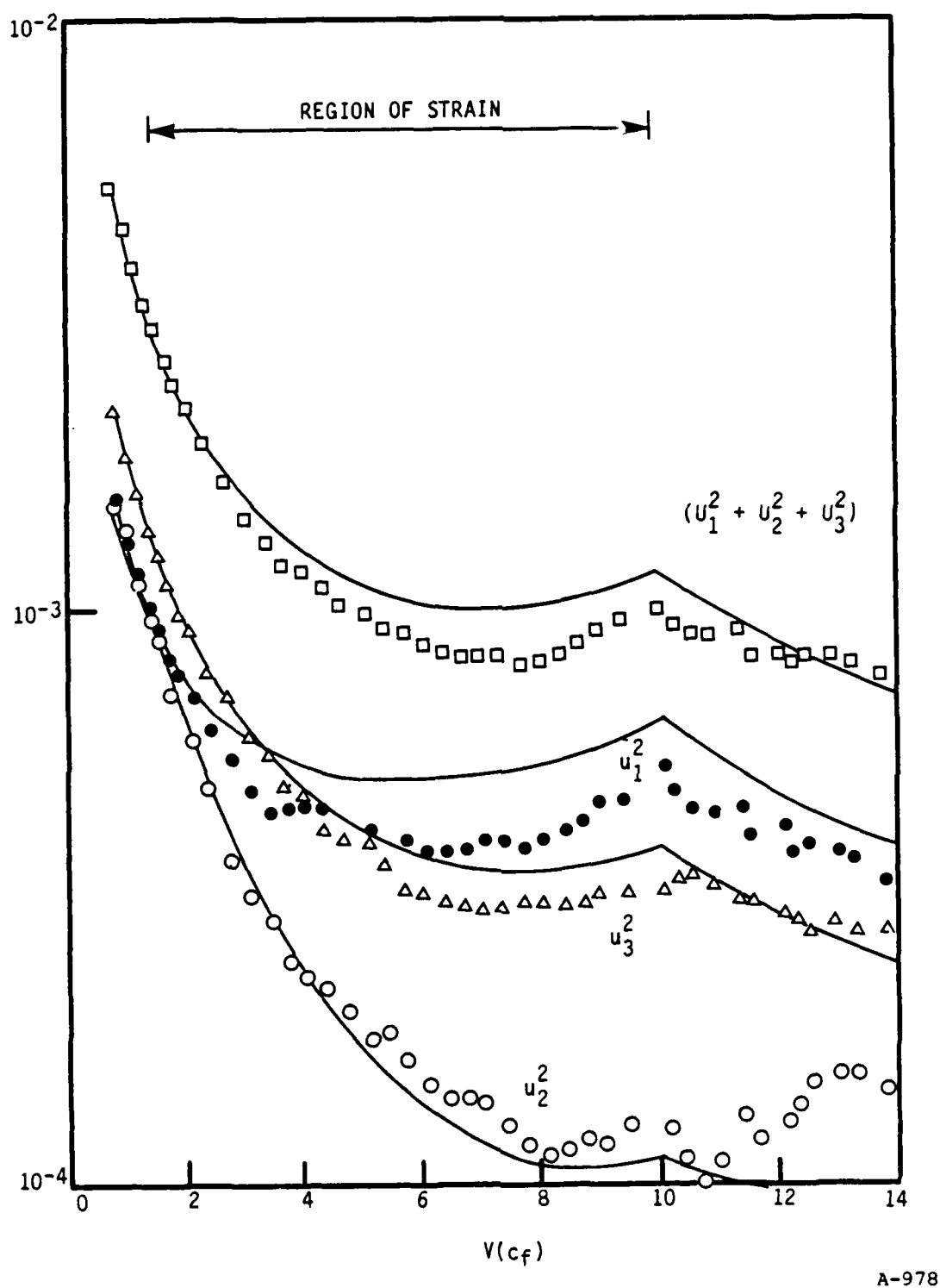
Figure 5. Decay of grid turbulence subjected to plane strain, comparisons with the experiment of Tucker and Reynolds 18
