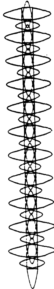
Fig. 22 Mode 25 of the 22-bay beam (frequency = 2205.80 Hz).
