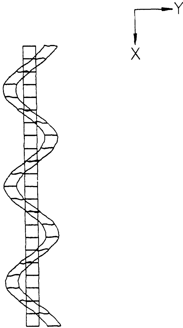
Fig. A24 Mode 5 (frequency = 326.50 Hz).
