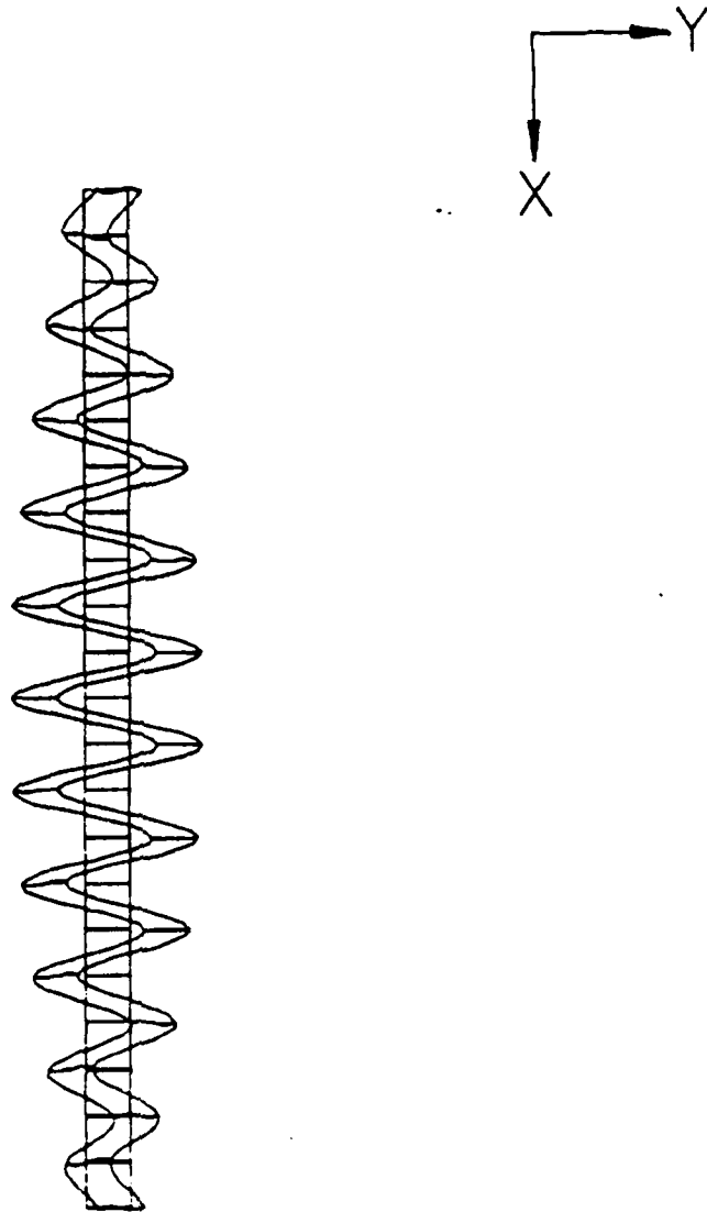
Fig. A27 Mode 23 (frequency = 1544.77 Hz).
