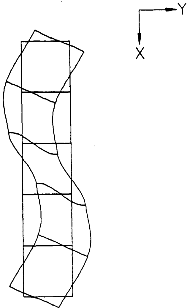
Fig. A2 Mode 2 (frequency = 69.16 Hz).
