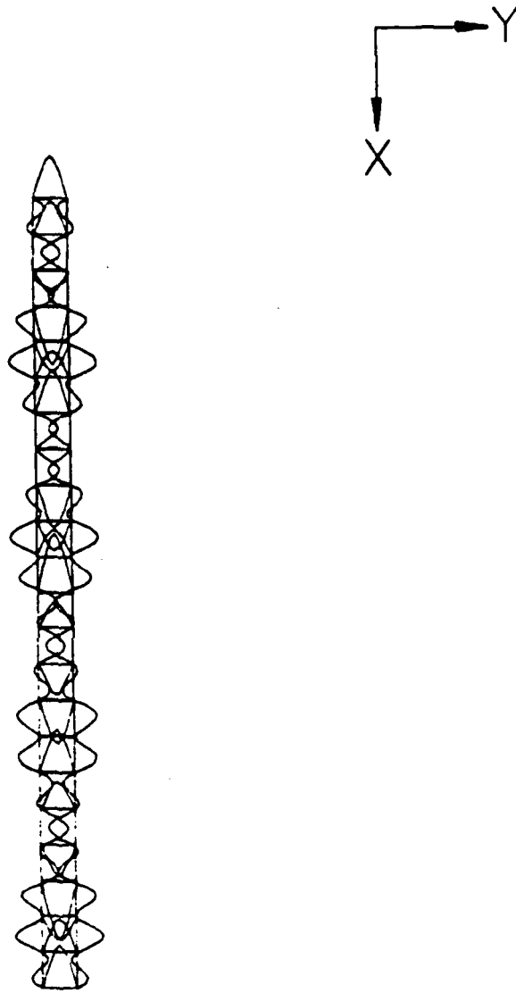
Fig. A30 Mode 44 (frequency = 3304.94 Hz).
