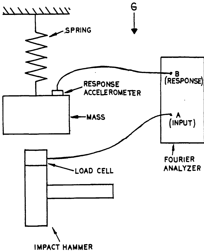
Fig. C3 Mass-spring system setup.
