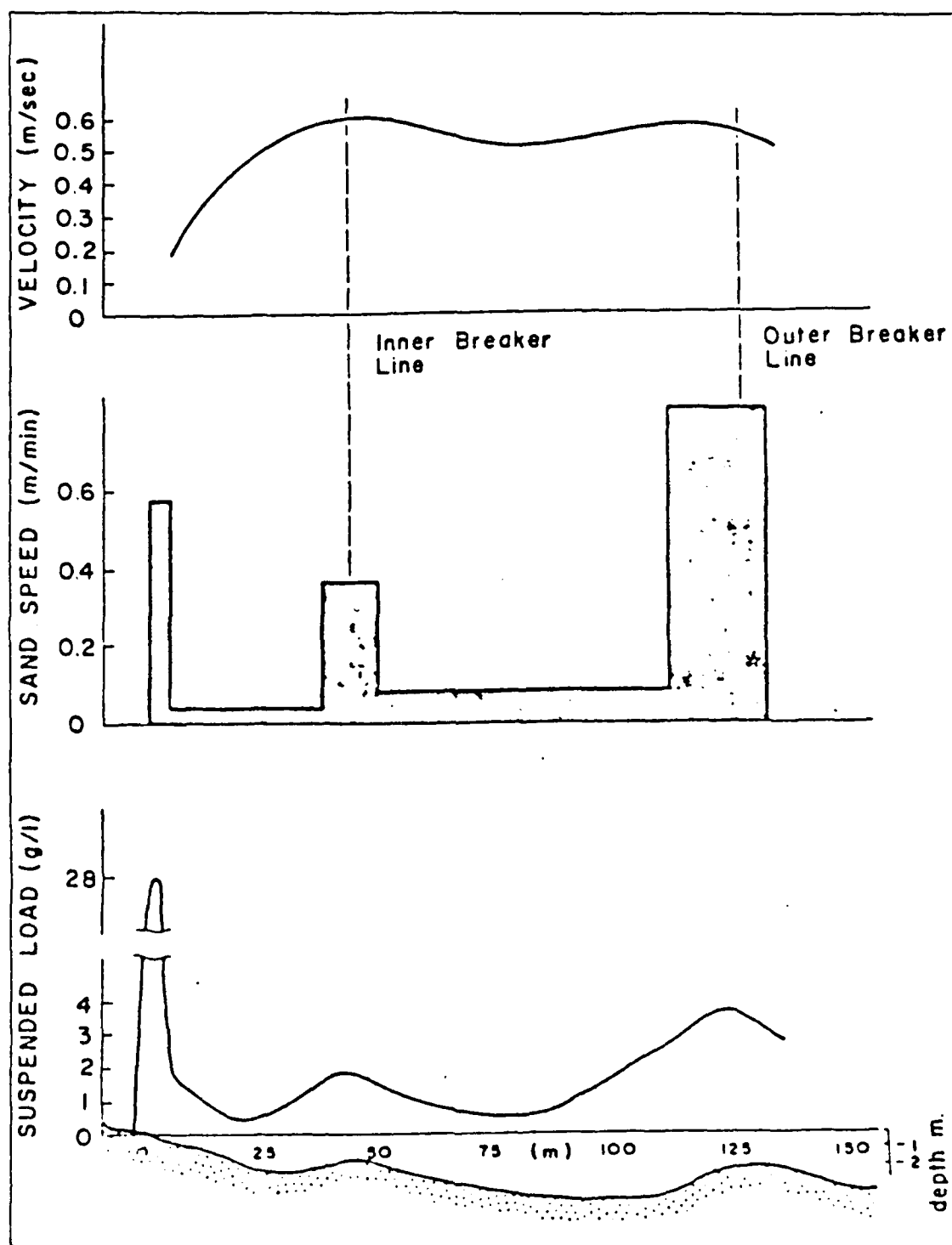
Figure 1.5 Distribution of longshore velocity and sediment transport across the surf zone (after Zenkovich, 1960).
