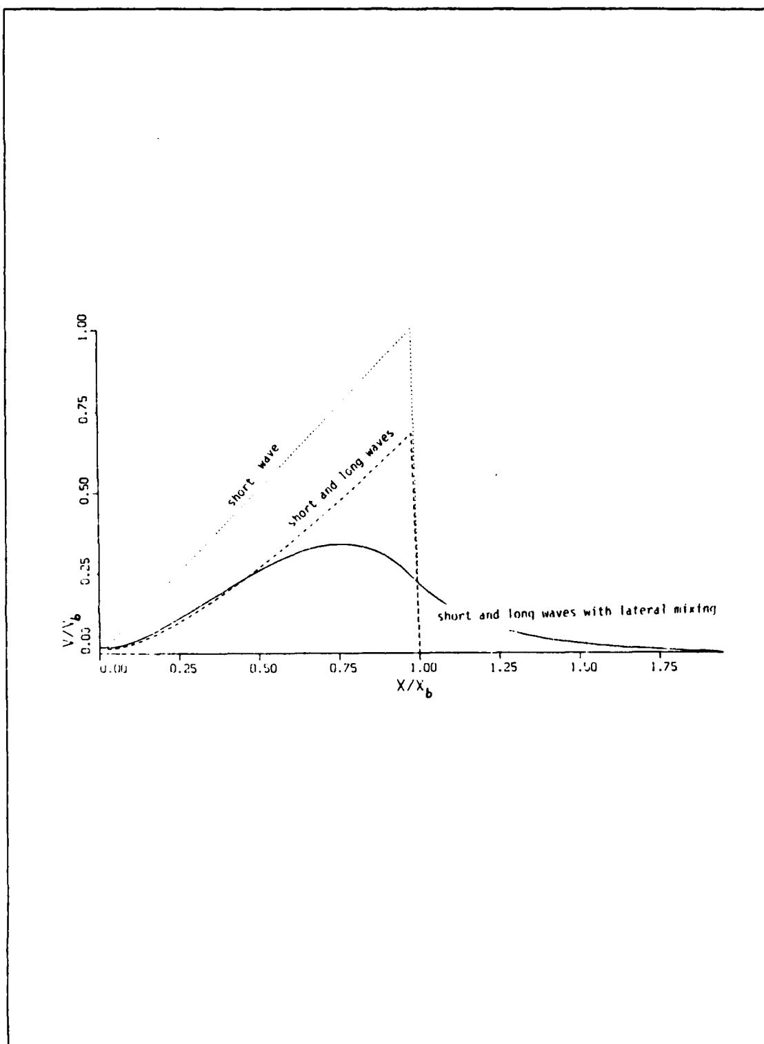
Figure 5.5 Steady longshore Current models, with and without adding lateral mixing, compared with Longuet-Higgins model (1970a).
