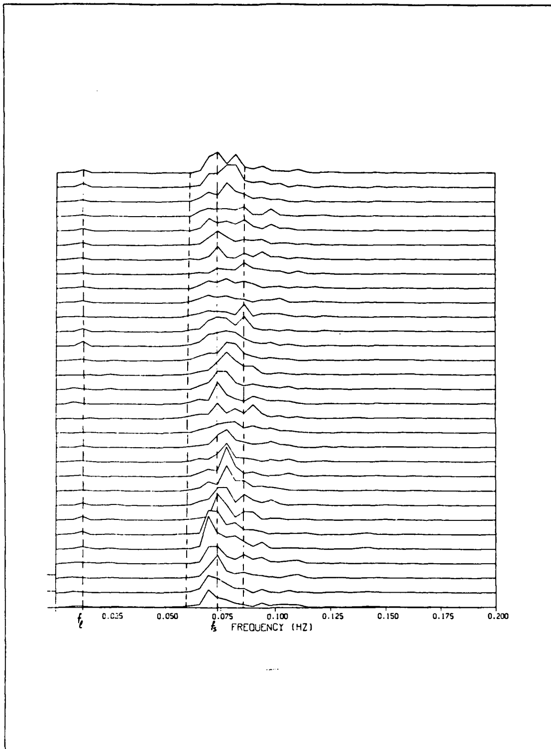
Figure 4.6 Spectral time series of current meter C0Dx with 50% overlapping calculated from four hour record, (4 Feb, 1980, Santa Barbara).
