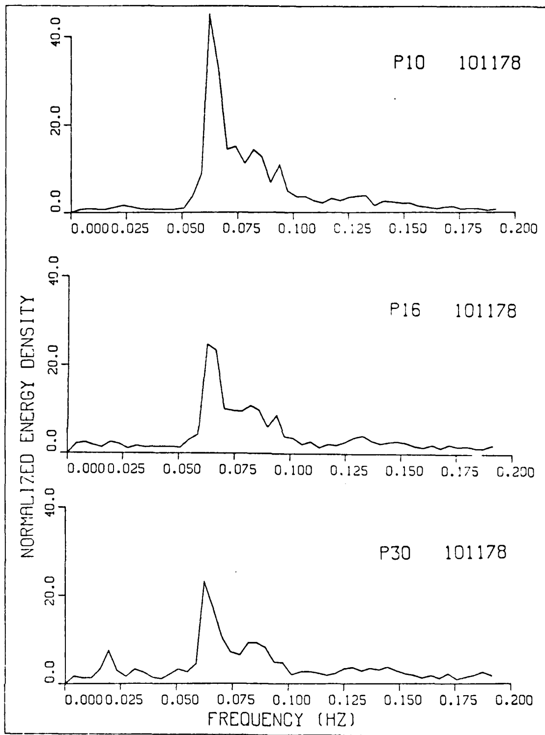
Figure 4.2. Normalized power spectra at different locations in 10 Nov., T.P., showing an onshore relative increase in the infragravity energy level.
