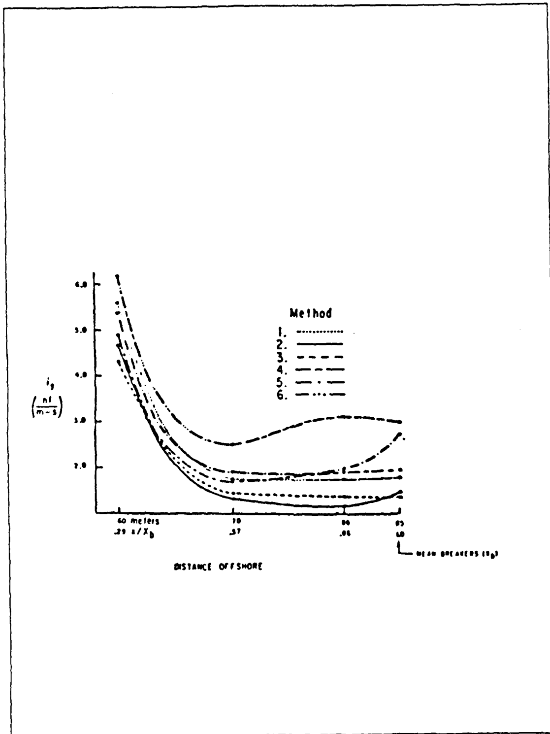
Figure 5.6 Measured longshore sediment transport rate i_s distribution, Santa Barbara (after White and Inman, 1986).
