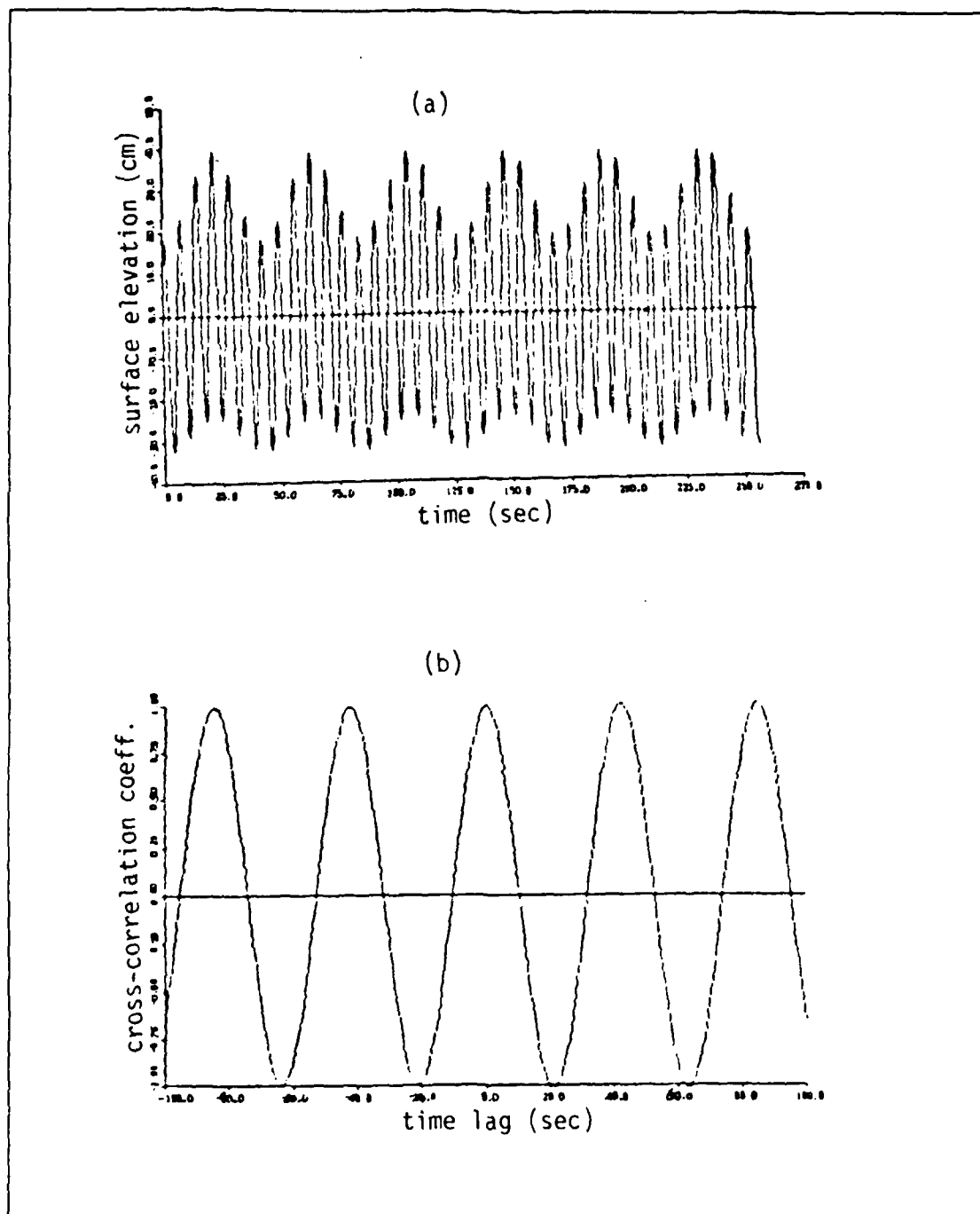
Figure 4.14 Theoretical model to examine the positive correlation between the wave envelope and the associated low frequency motion within the surf zone, (a) segment of time series (b) cross-correlation function.
