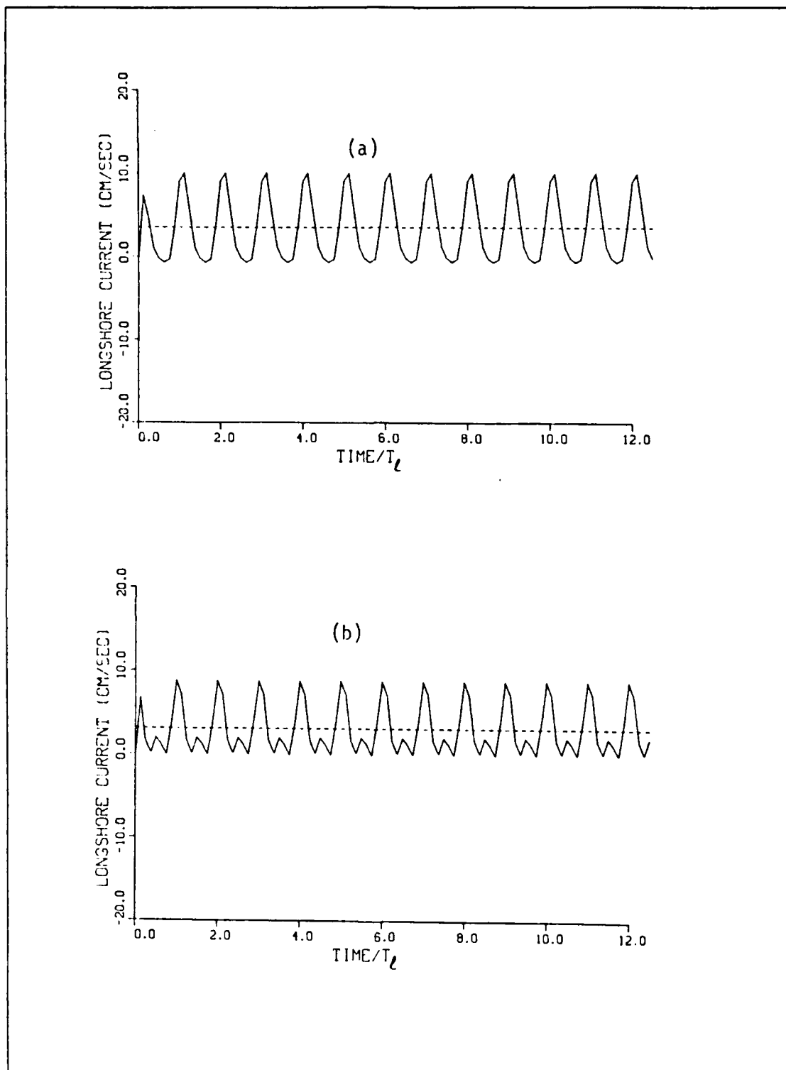
Figure 5.4 Time variability of the longshore current (a) x = 2.0 m (b) x = 1.0 m.
