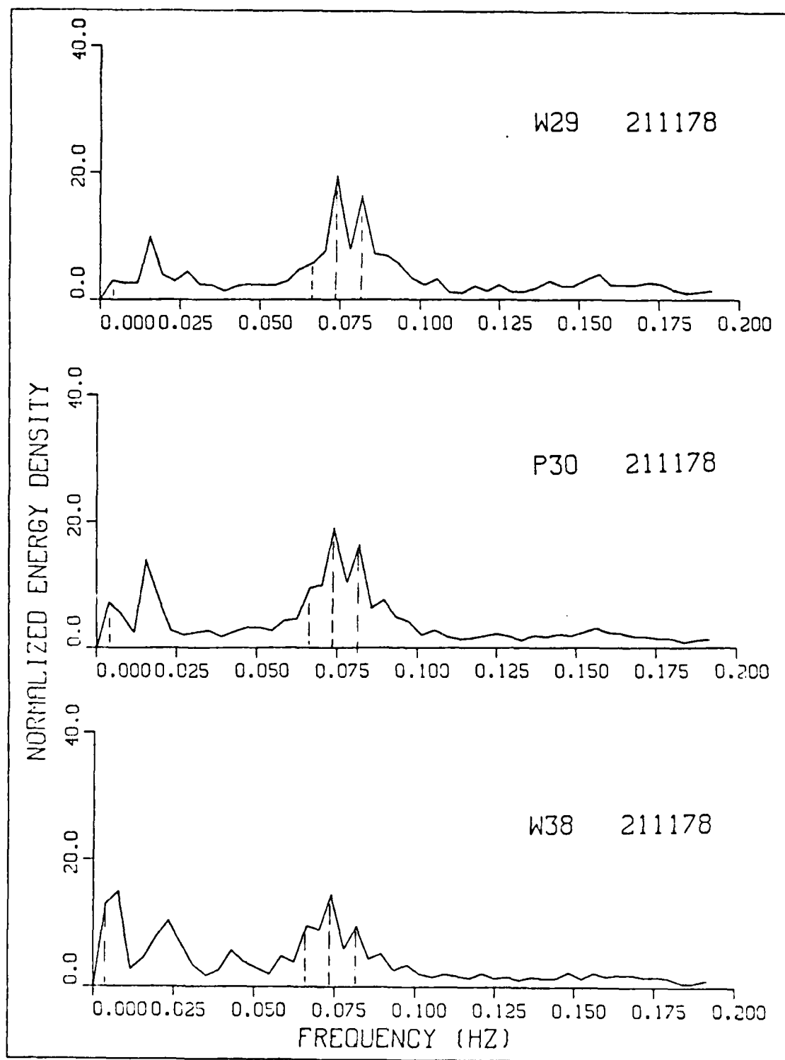
Figure 4.5. Normalized spectra showing significant peaks at frequencies of dominant long wave f_L , short wave f_S and side bands.
