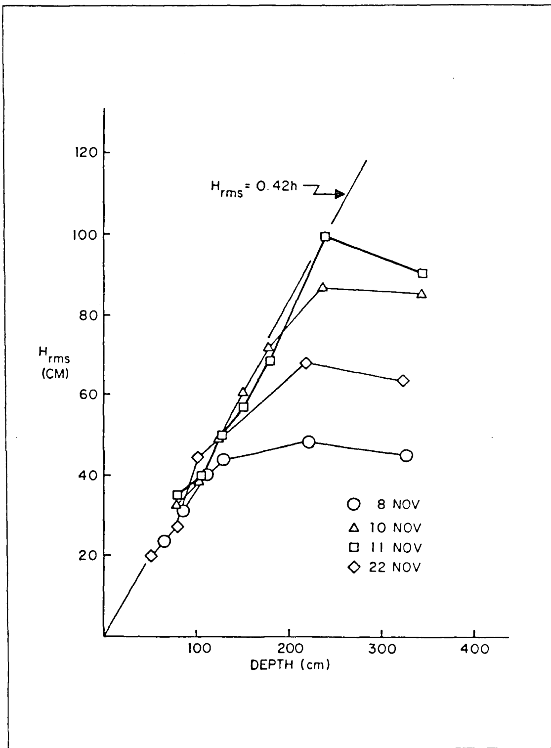
Figure 2.1 Wave heights inside the surf zone defining breaker index and showing saturation (after Thornton and Guza, 1982).
