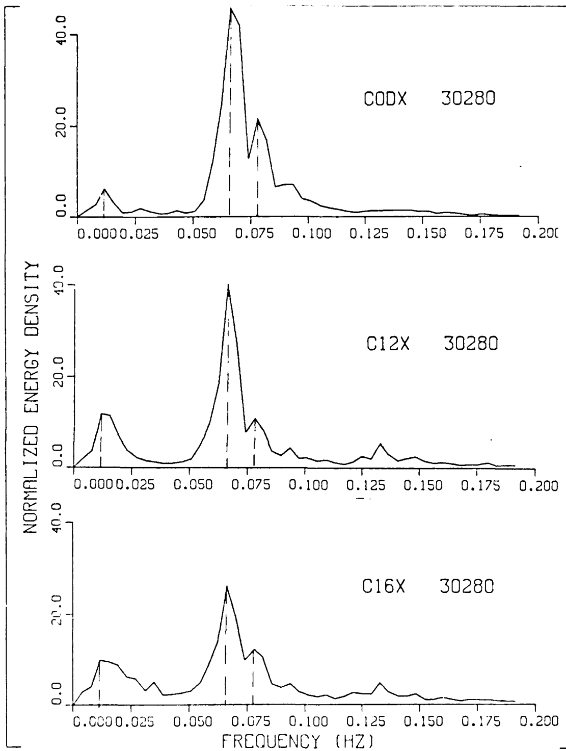
Figure 4.3 Normalized power spectra at different locations in 3 Feb., S.B.
