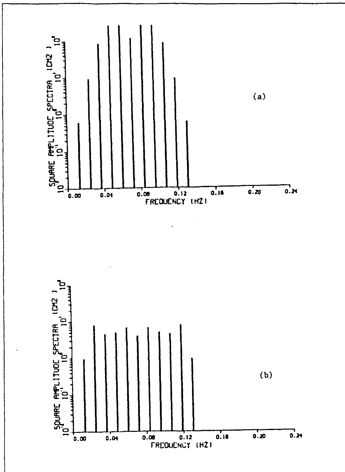
Figure 3.3 Amplitude square spectra of the modulated short wave at offshore distance: (a) x = 40.0 m (b) x = 0.5 m.
