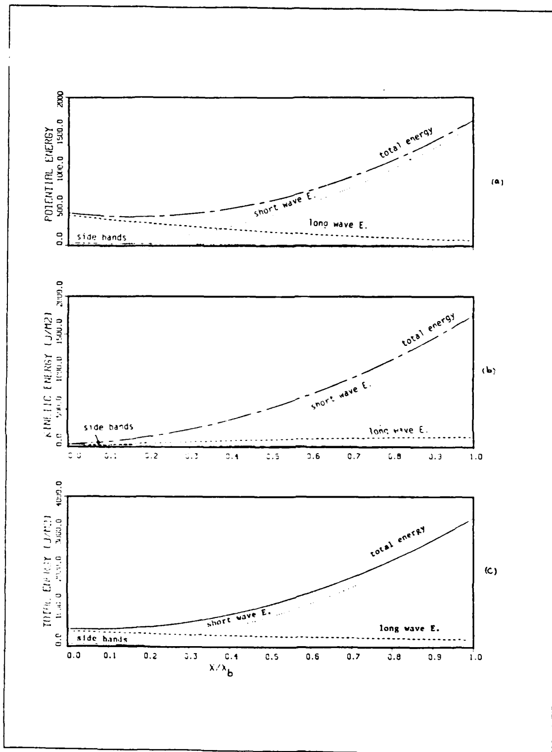
Figure 3.5 Theoretical wave model to predict energy inside the surf zone, (a) potential energy (b) kinetic energy (c) total energy.
