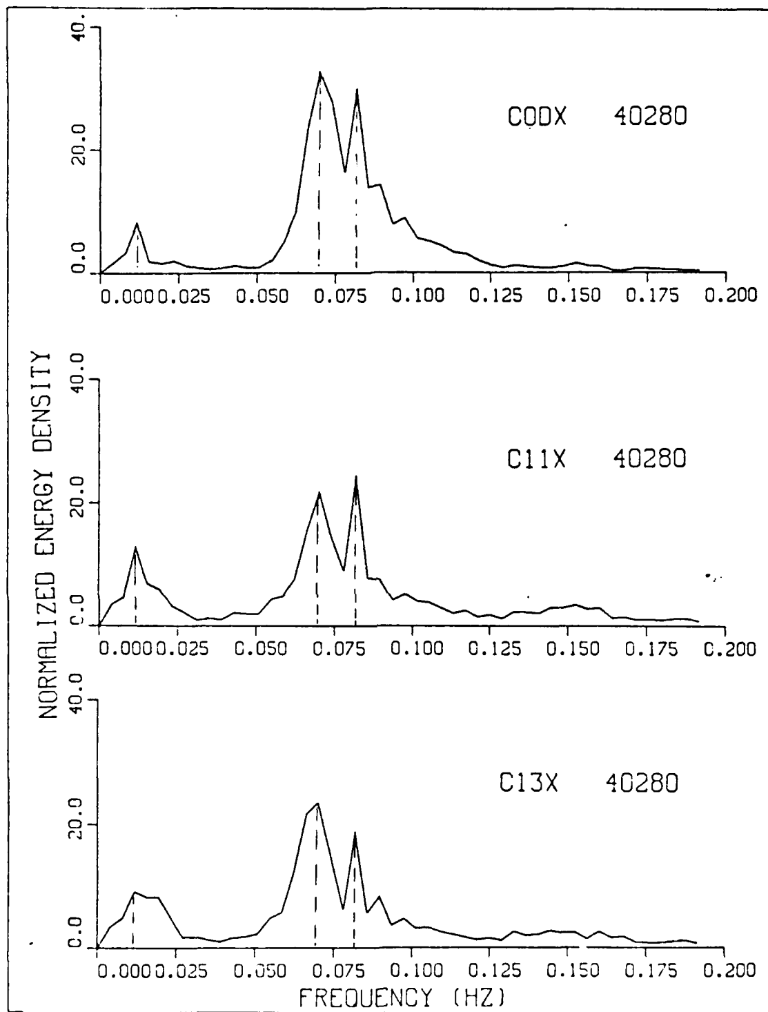
Figure 4.4 Normalized power spectra at different locations in 4 Feb., S.B.
