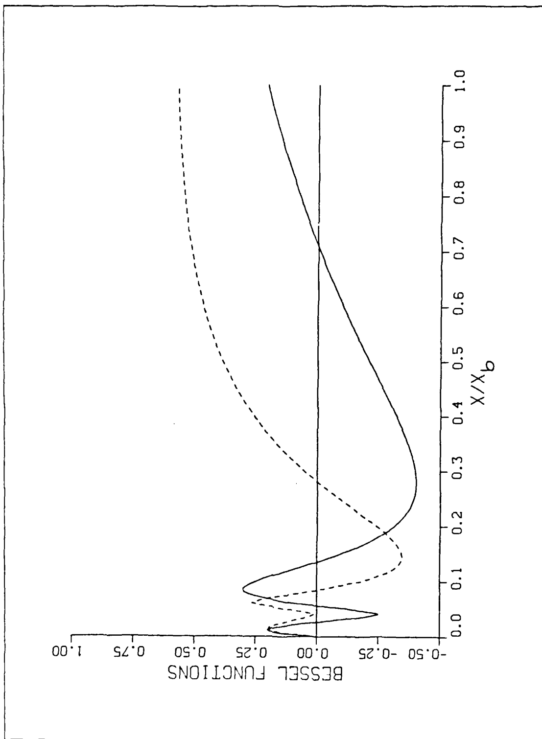
Figure 3.2 Behaviour of the Bessel functions J_0(m_k) (solid curve) and J_1(m_k) (dashed curve) across the surf zone.
