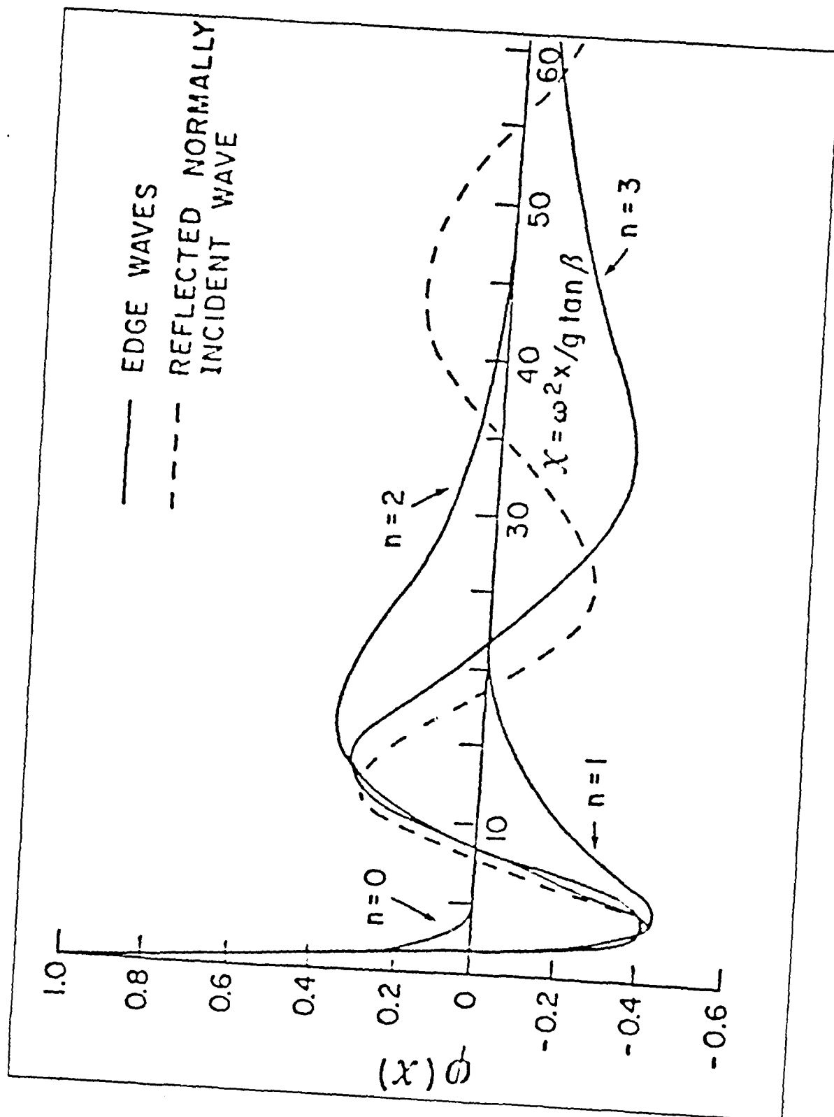
Figure 2.2 Modes of edge waves and reflected waves, \phi is the velocity potential.
