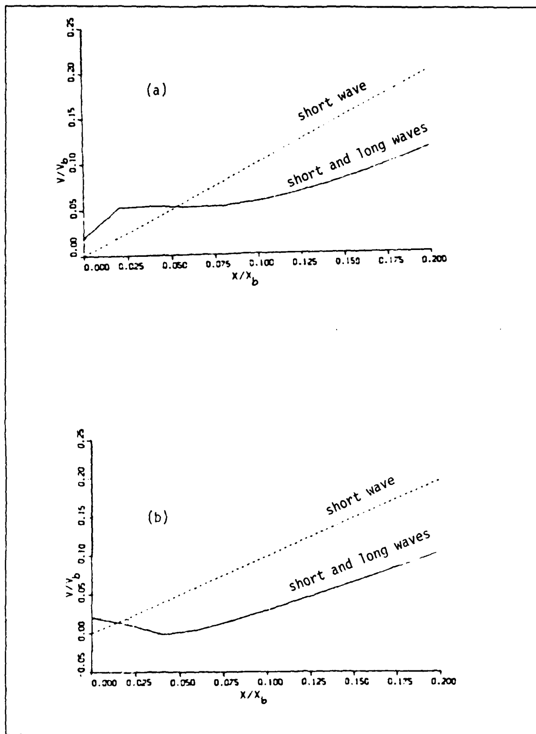
Figure 5.3 Unsteady longshore current distribution, at time (a) t = \text{long wave period} (b) t = 1/2 \text{ long wave period} .
