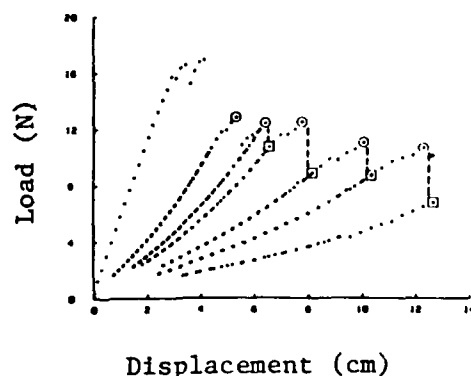
Figure 5. Load vs. displacement ( 2u ) for type C specimen.
