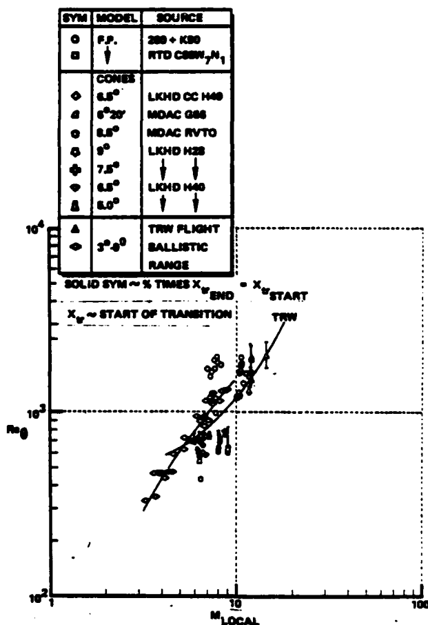
Figure 6 Correlation of Transition Measurements in the Calspan Shock Tunnels with Ballistic and Downrange Measurements
