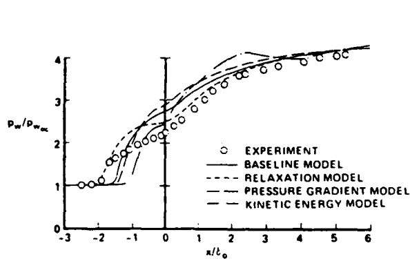
Figure 8 Comparison of computations and surface measurements; \alpha = 24^\circ , Ref. 8.
