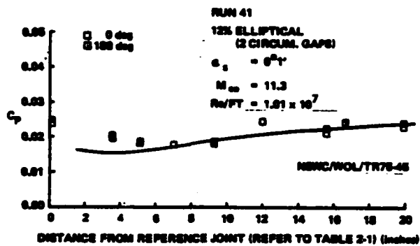
Figure 32 Pressure Distribution on the Frustum of the 6° Cone Downstream of Two Circumferential Gaps
