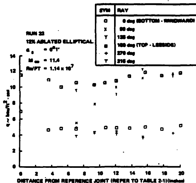
Figure 26 Heat Transfer Distribution to the 6^\circ Cone in Asymmetric Transitional Flow Induced by Two Adjacent Gauges in the Elliptical Nose Tip
