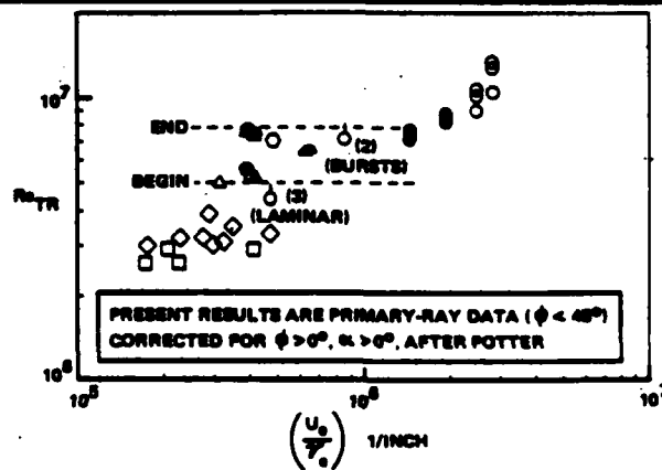
Figure 7 Transition Reynolds Number Vs. Unit Reynolds Number; Present Data Vs. Krogmann and Stetson
