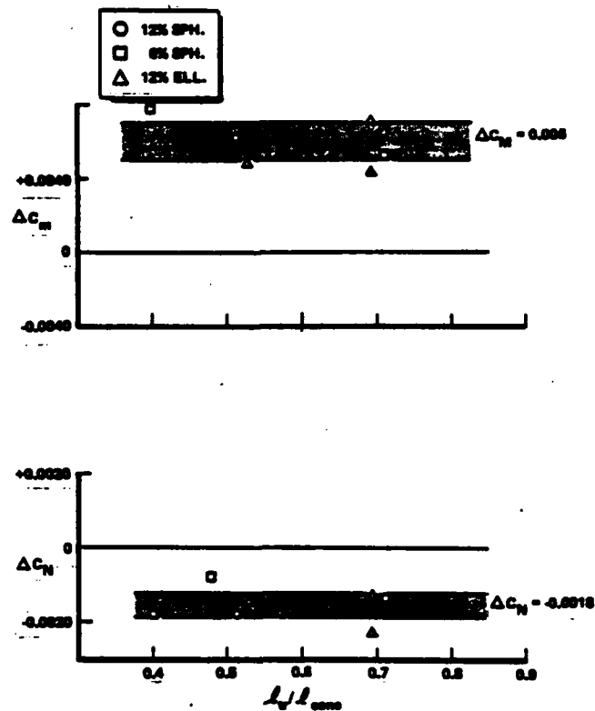
Figure 34 Incremental Force and Moment Measurements Resulting from Regions of Body-Fixed Transition
