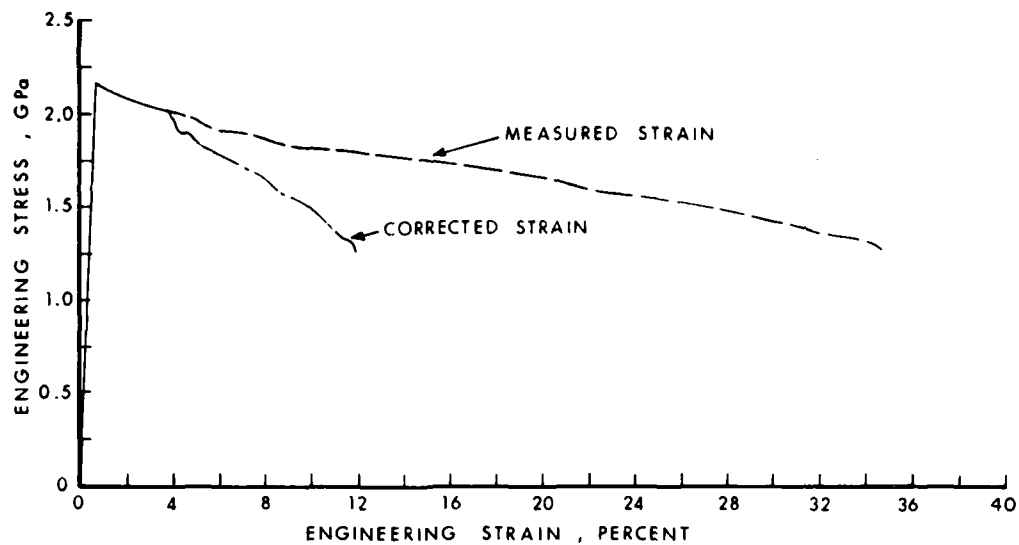
Figure 10. Measured and Corrected Engineering Stress versus Engineering Strain, to Rupture, for Precipitation Hardened 300 Maraging Steel in Tension, from Test T115.
