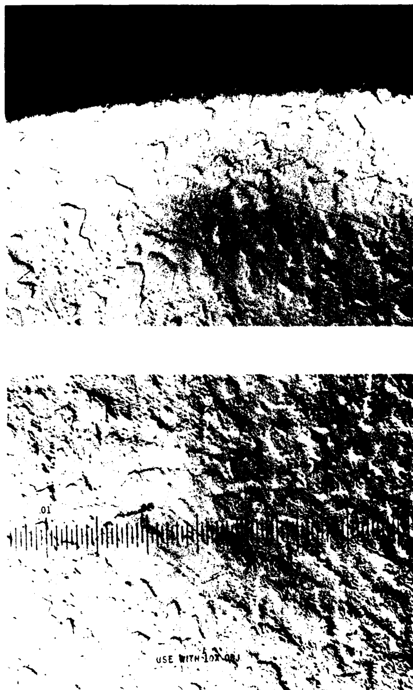
Figure 2. Transverse Sections of Annealed Ta-10W Bar. Bar was used on tensile test T152. Top photo is at the edge of the bar and bottom photo is from the middle of the bar. Specimen is overetched. Reticle is graduated in inches.
