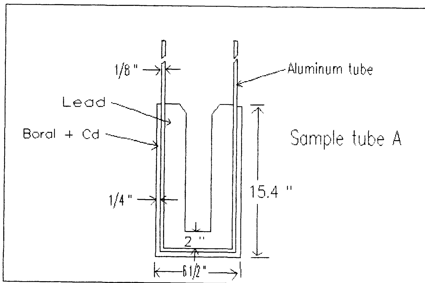
Fig. 33 Tube A shielding design
