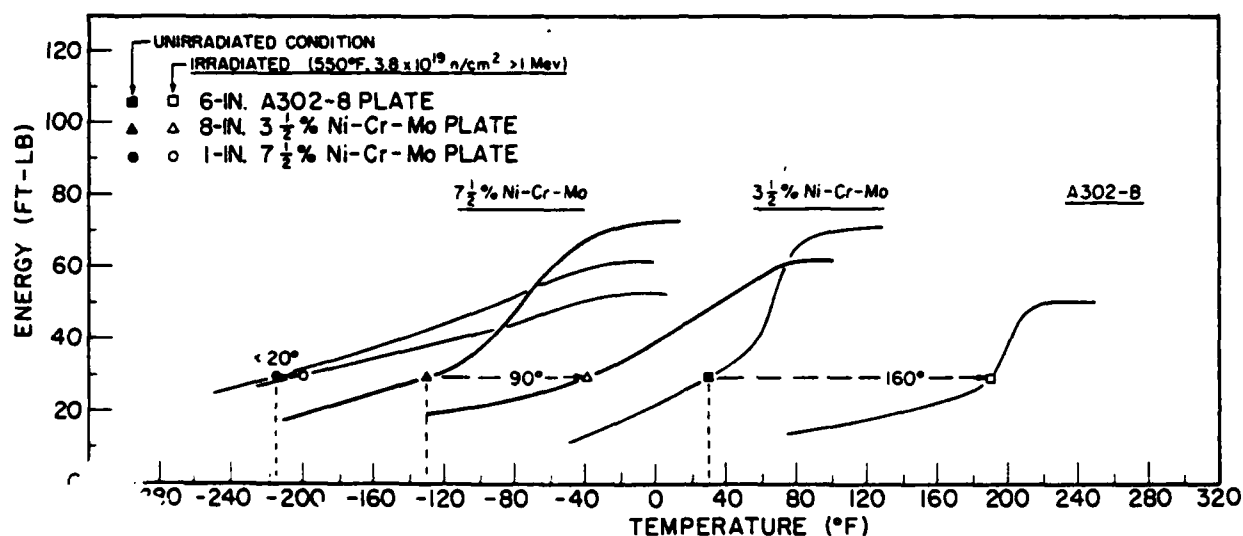
Fig. 28 Charpy V-notch ductility characteristics of three steels of different strength levels after simultaneous irradiations at 550°F (Ref. [21])
