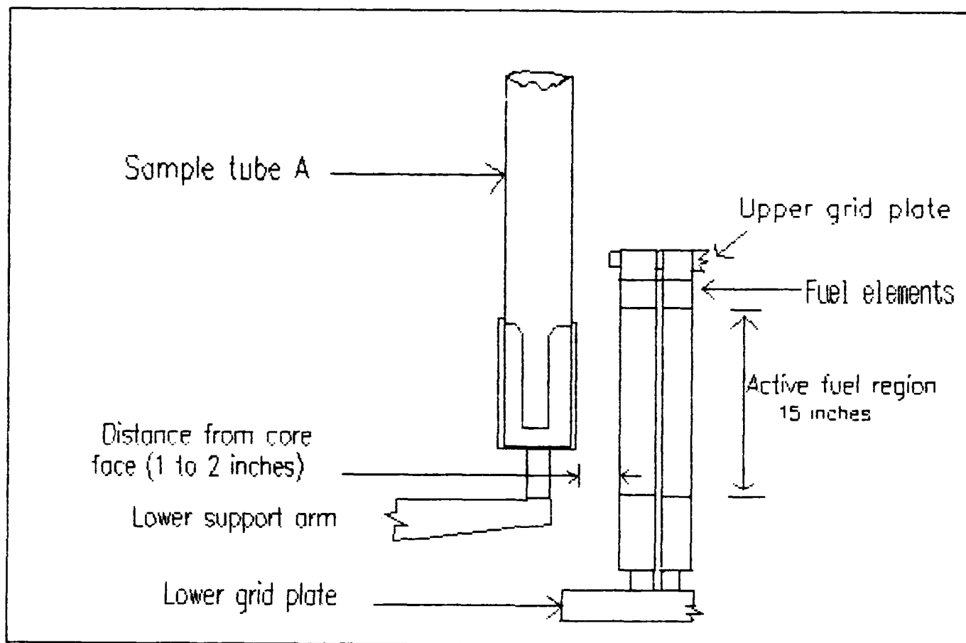
Fig. 32 Tube A irradiation arrangement
