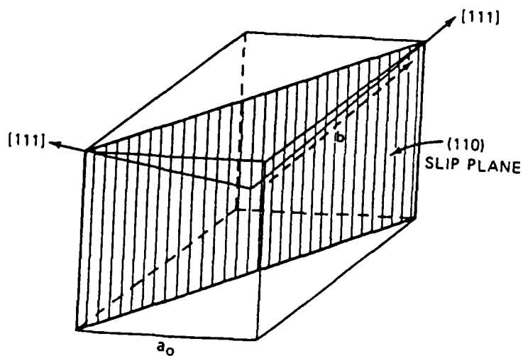
Figure 15 Slip planes and slip direction in bcc crystals (Ref. [2])
