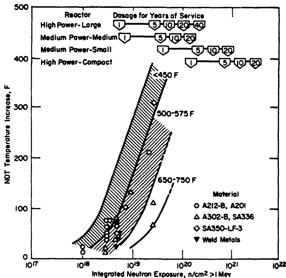
Fig. 22 Increase in the NDT resulting from irradiation at higher temperatures (Ref. [3])
