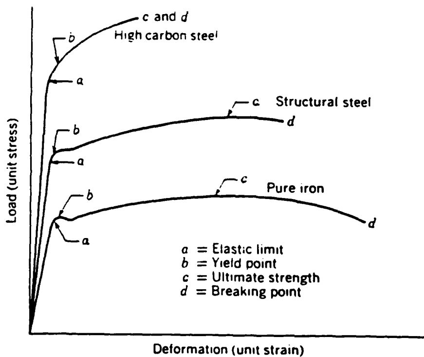
(6a) Stress-strain diagrams (Ref. [10])
