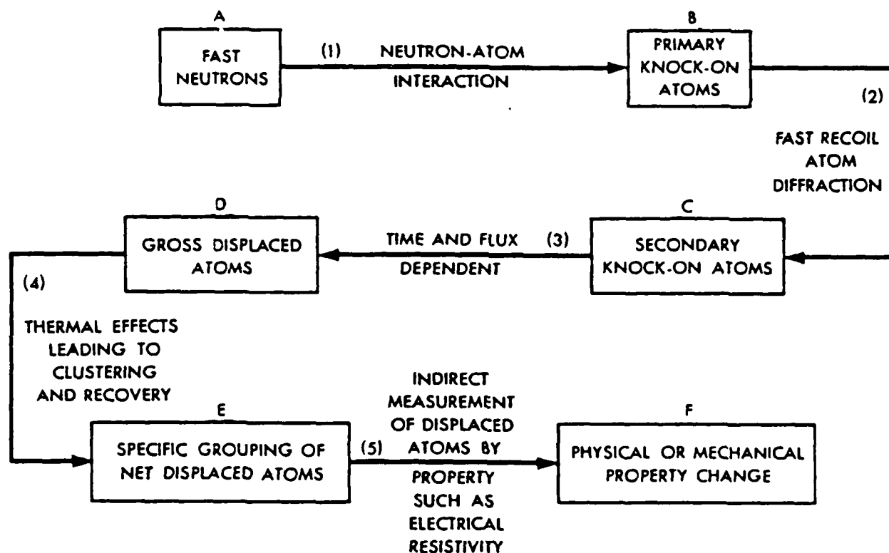
Fig. 5 Schematic diagram of the damage mechanism in a neutron-irradiated solid (Ref.[8])
