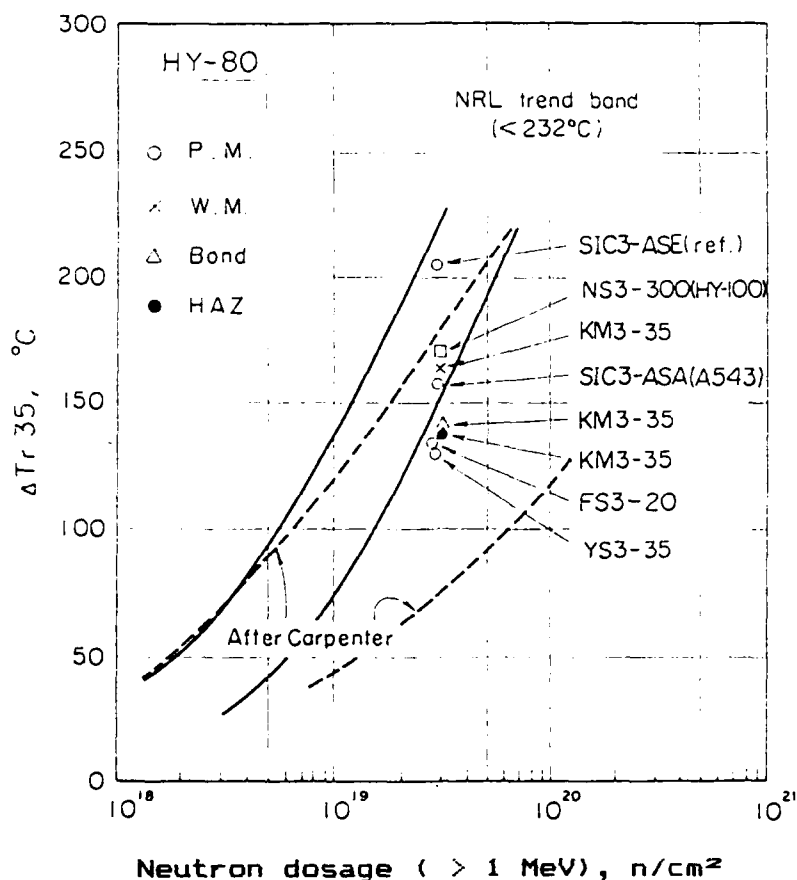
Fig. 26 DBTT changes of HY-80 steels as compared to trends established by NRL and by Carpenter (Ref. [18])
