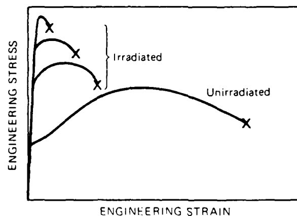
Fig. 18 Effect of fast neutron irradiation on the tensile properties of reactor steels (Ref. [2])
