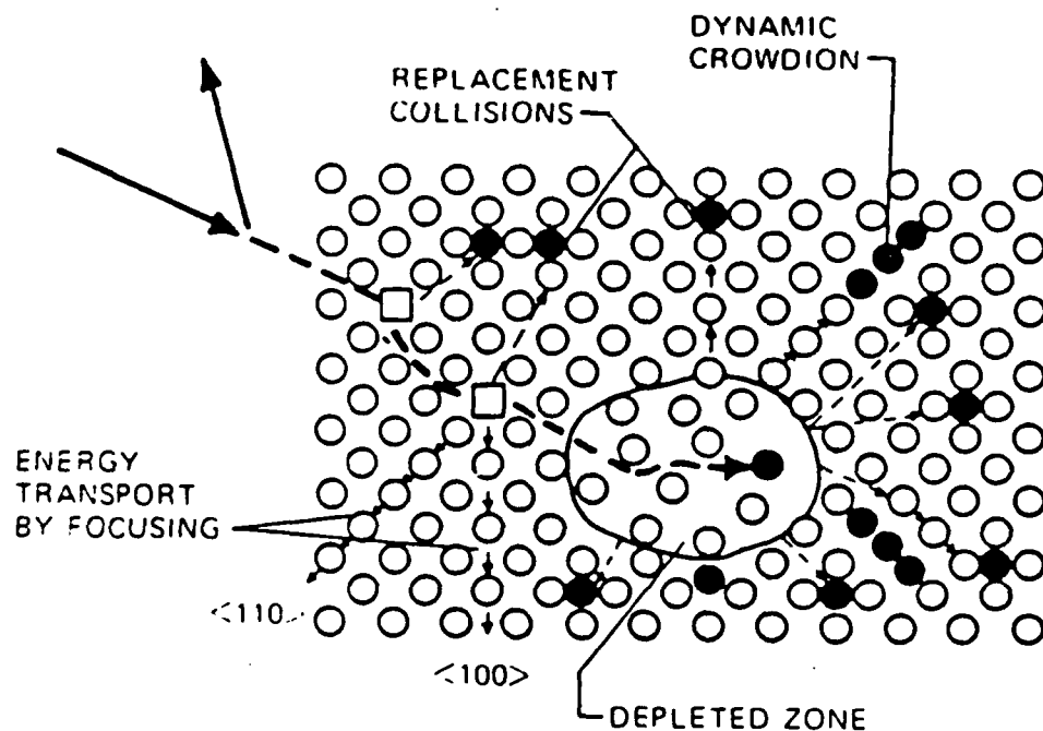
Fig. 3 Later version of a displacement spike (Ref. [2])
