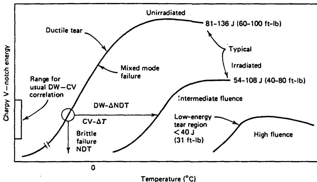
Fig. 16 Transition temperature shift resulting from neutron-irradiation (Ref. [11])
