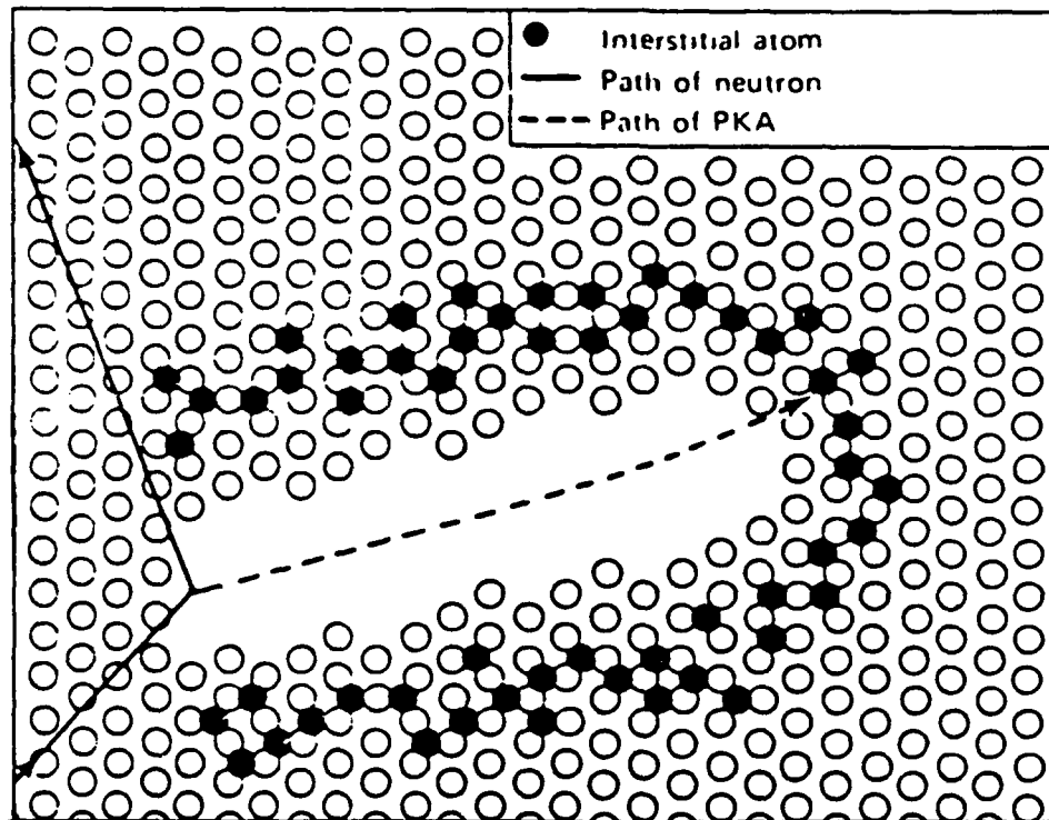
Fig. 2 Original version of a displacement spike (Ref. [2])
