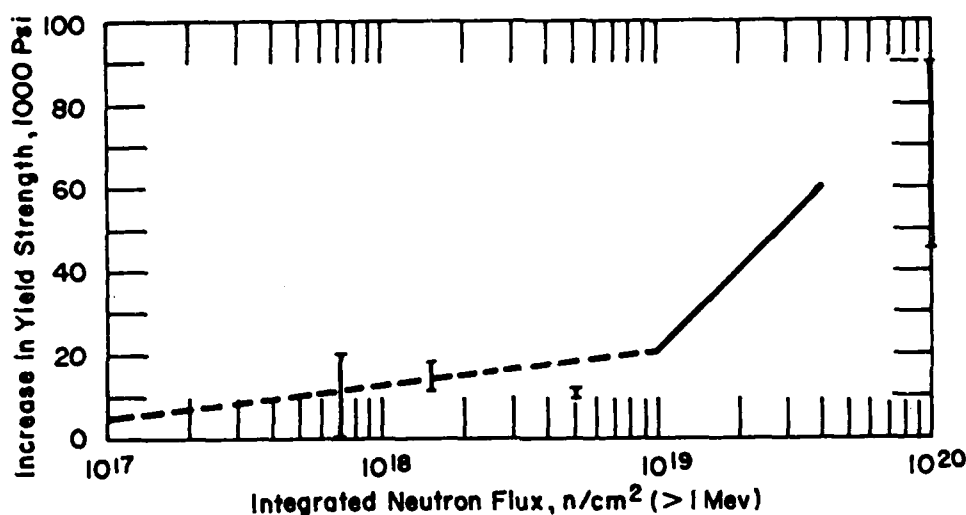
Fig. 24 Yield strength increases of carbon and alloy steels after irradiation at temperatures to 500°F (Ref. [3])
