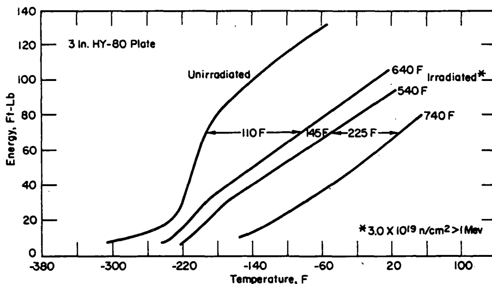
Fig. 23 Transition temperature shifts resulting from elevated temperature irradiation of HY-80 steel (Ref. [3,14])
