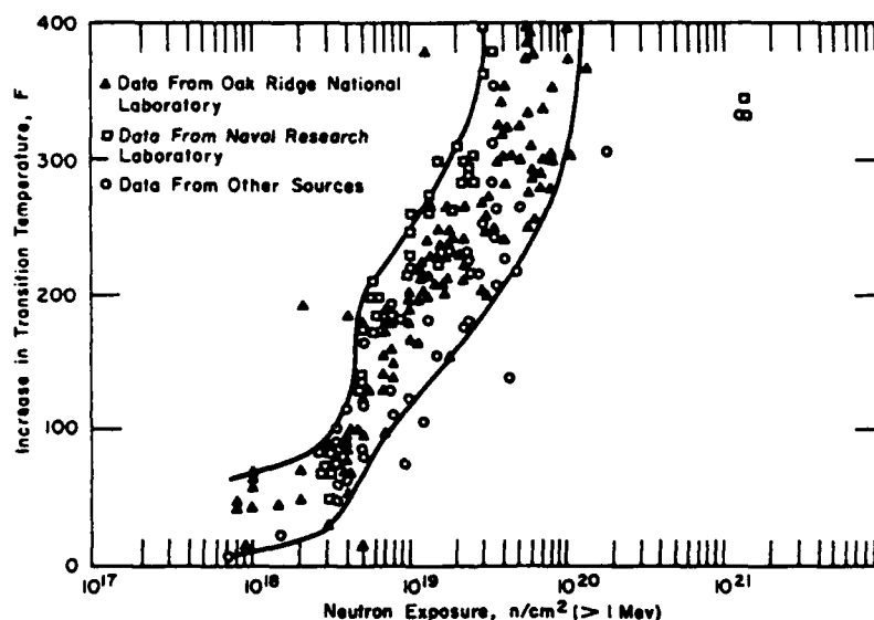
Fig. 21 Effect of neutron radiation on the notch-toughness of carbon and alloy steels irradiated below 500°F (Ref. [3])
