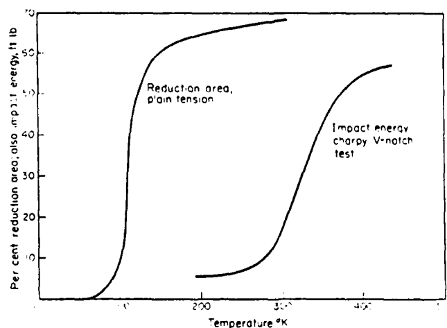
Fig. 9 Ductile-brittle transition (Ref. [4])
