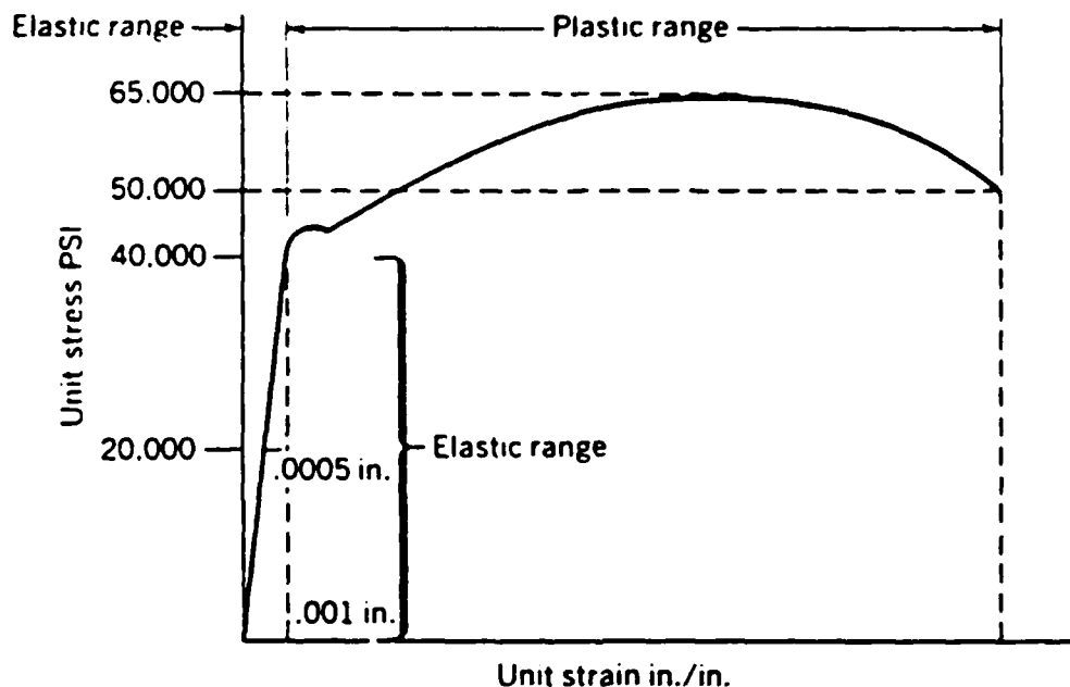
Fig. 7 Stress-strain diagram for a ductile steel (Ref.[10])
