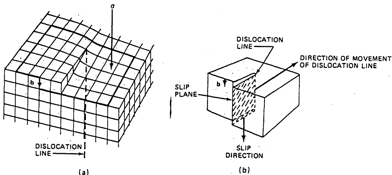
Fig. 13 The screw dislocation (Ref. [2])
