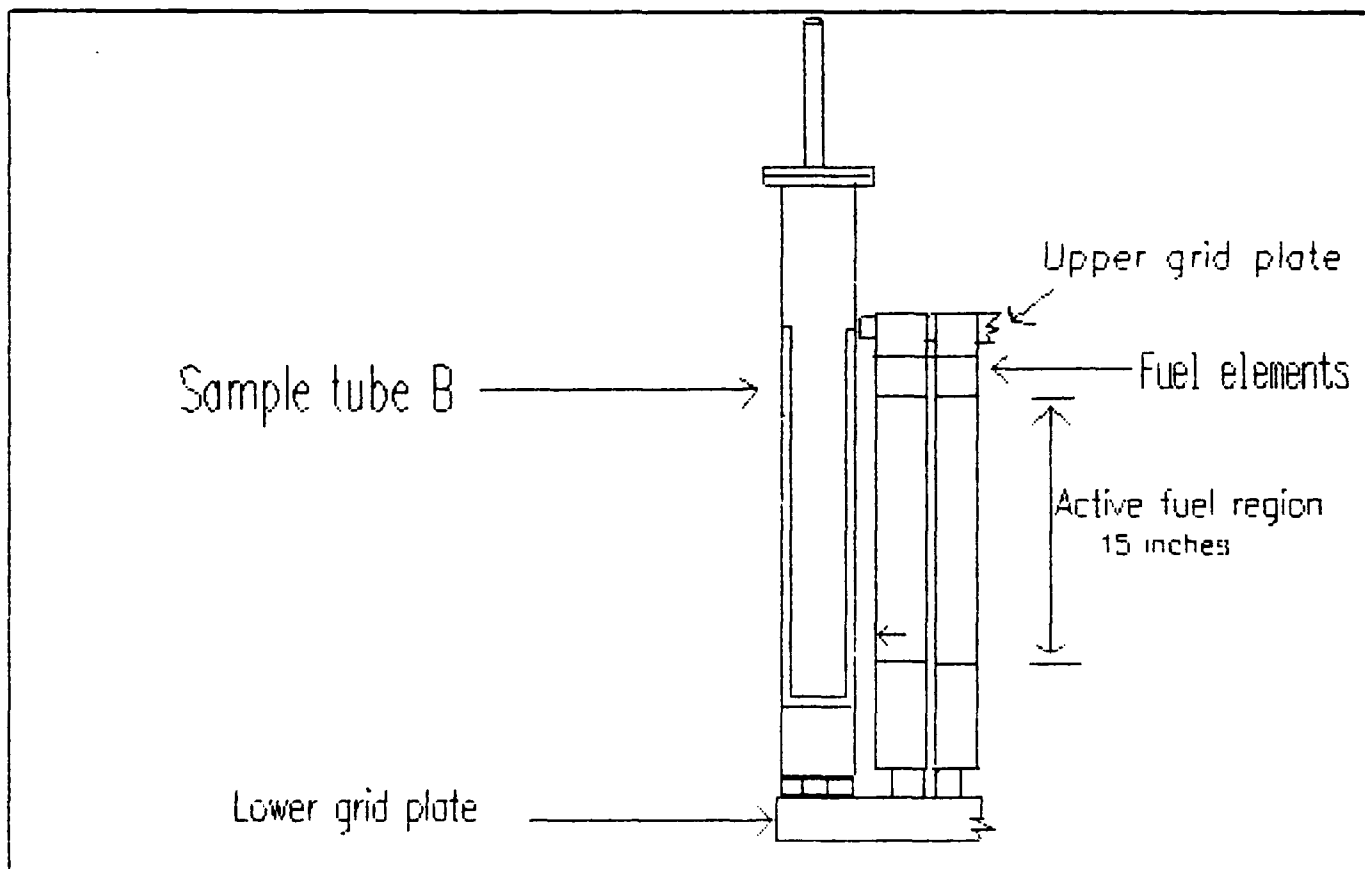
Fig. 34 Tube B irradiation arrangement
