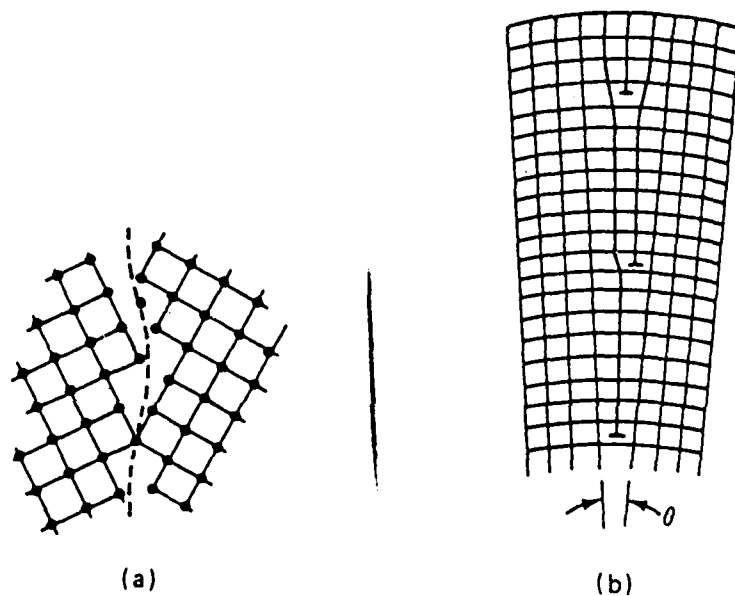
Fig. 11 Grain-boundary models: (a) Large-angle grain boundary (b) Small-angle grain boundary (Ref. [2])
