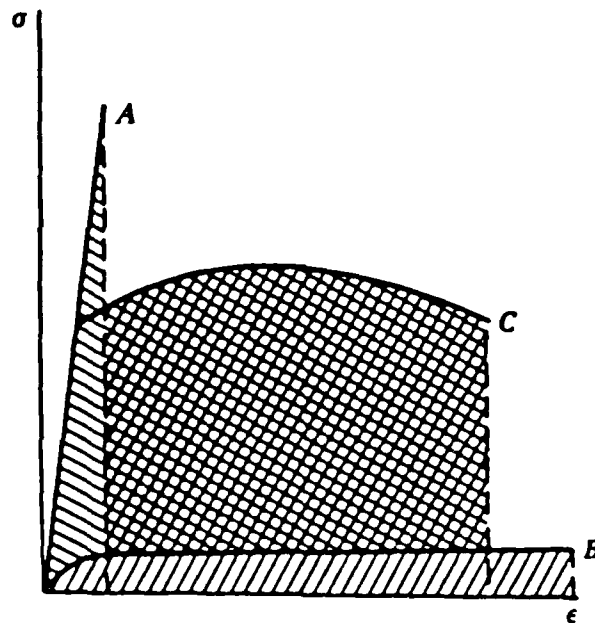
Fig. 8 Stress-strain curves showing toughness (Ref. [11])
