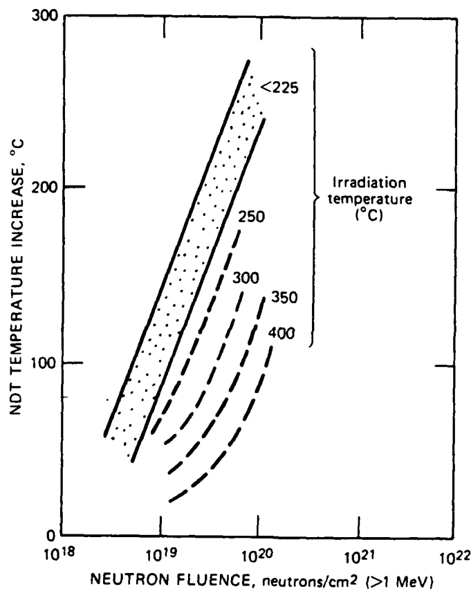
Fig. 17 Effect of fast neutron fluence on the increase in the nil-ductility-temperature (Ref. [2])
