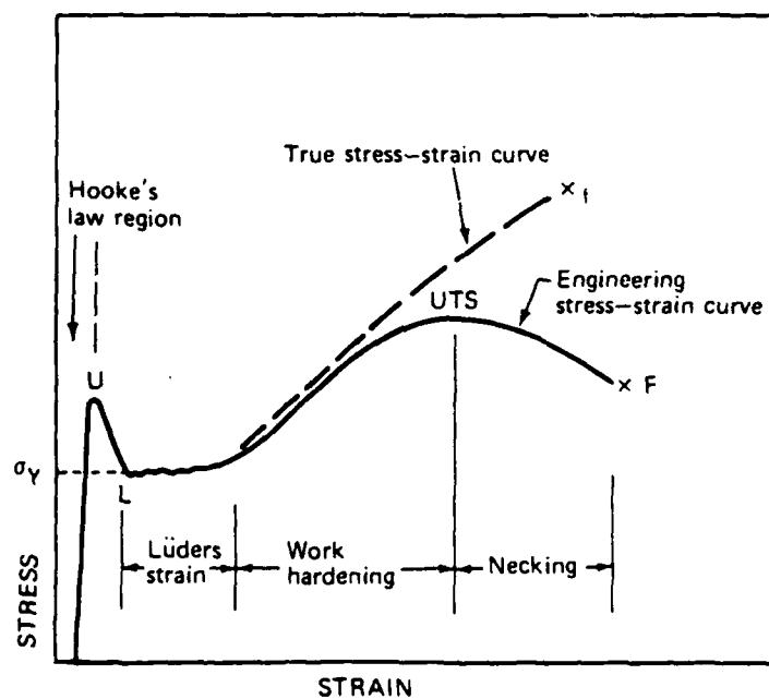
(6b) Stress-strain curve for a ferritic steel (Ref. [2])
