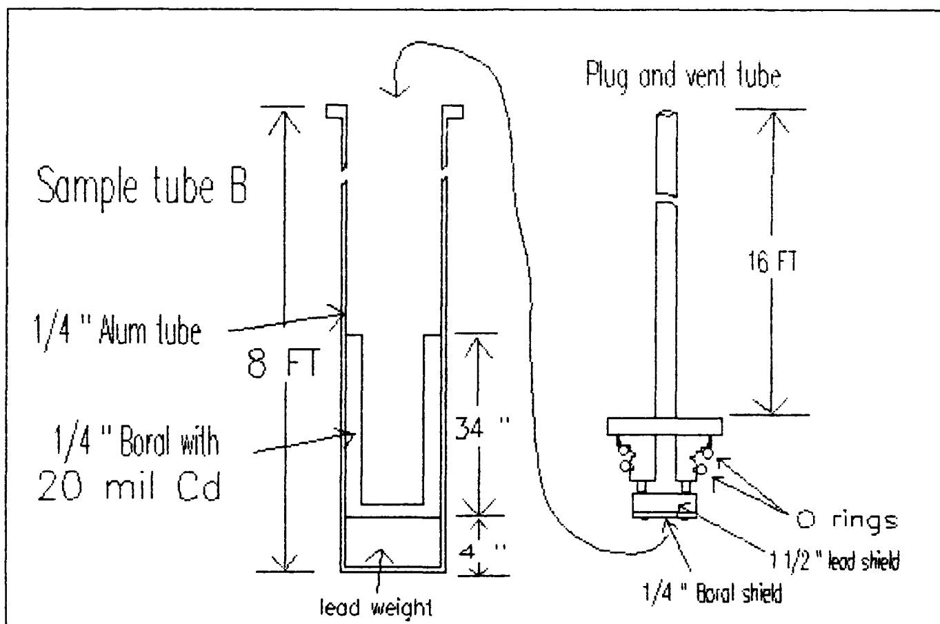
Fig. 35 Tube B shielding design
