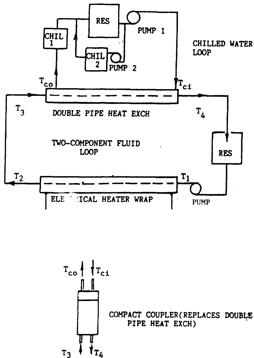
Fig. 1. Schematic of Test Loop Showing Standard Double-Pipe Heat Exchanger and Compact Coupler
