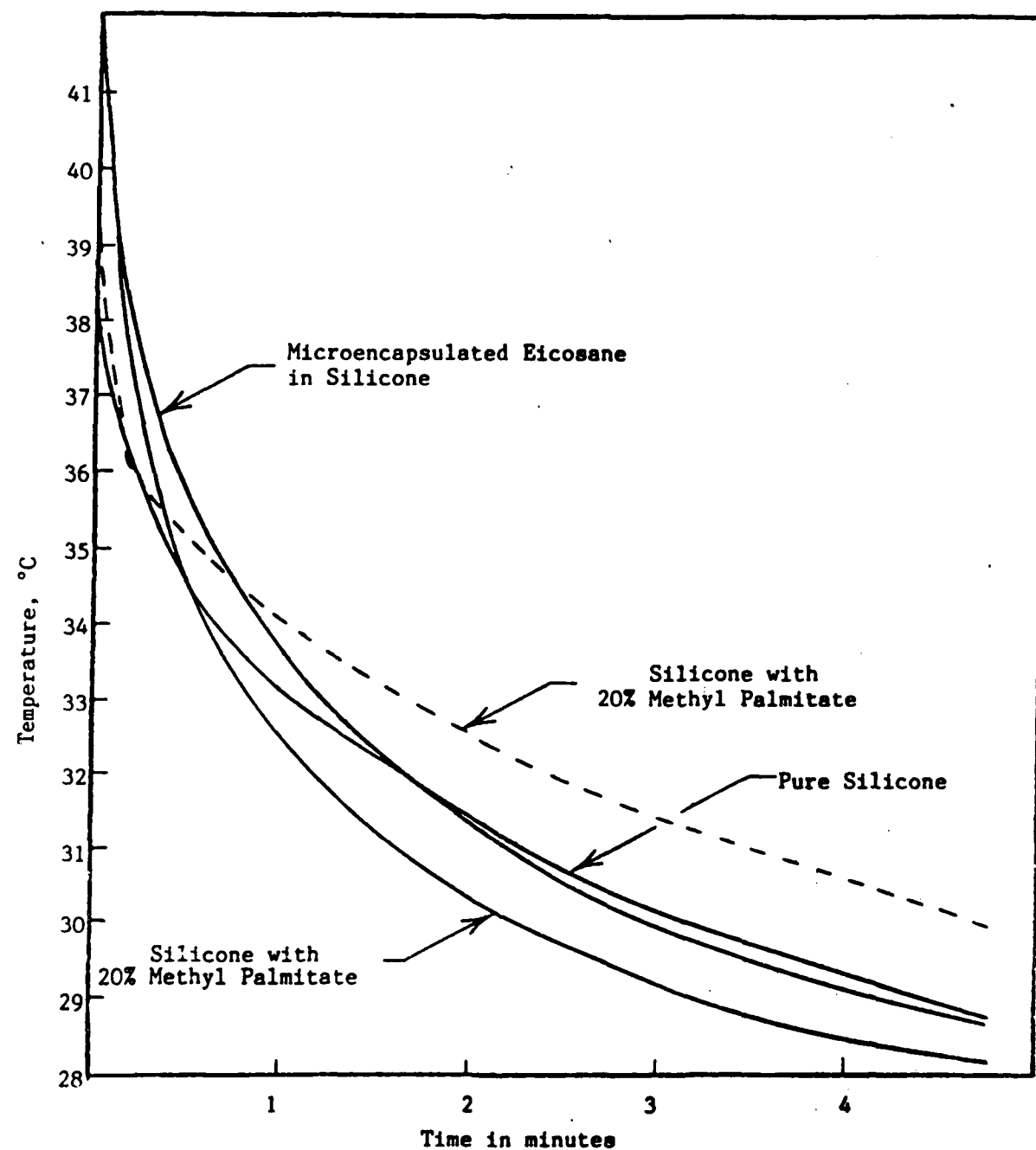
Fig. 14 - Temperature Decay of Resistors of Circuit Number 1 After Sudden Removal of Voltage.
