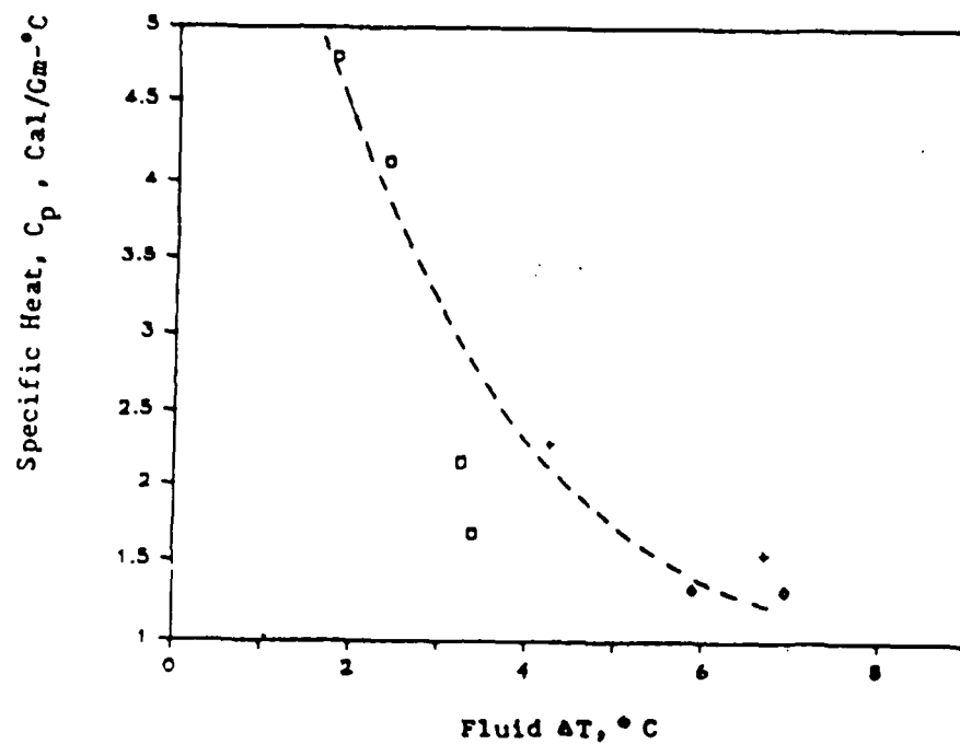
Figure 2. Slurry Specific Heat Versus Slurry Temperature Change, Illustrating Loop Tuning and High C_p that Results
