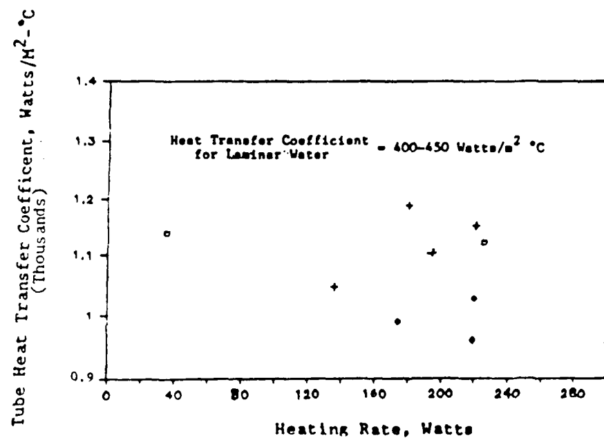
Figure 3. Heat Transfer Coefficient Inside Heater Tube, for Various Runs of Different PCM Slurries
