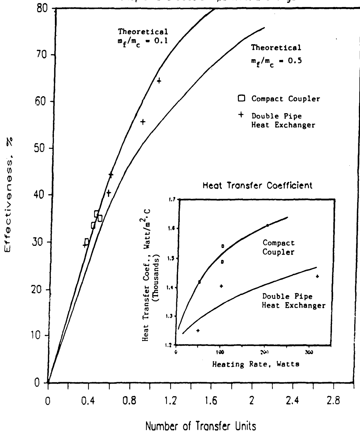
FIG. 5 - HEAT TRANSFER COEF. AND EFFECTIVENESS Coupler and Double Pipe Heat Exchanger
