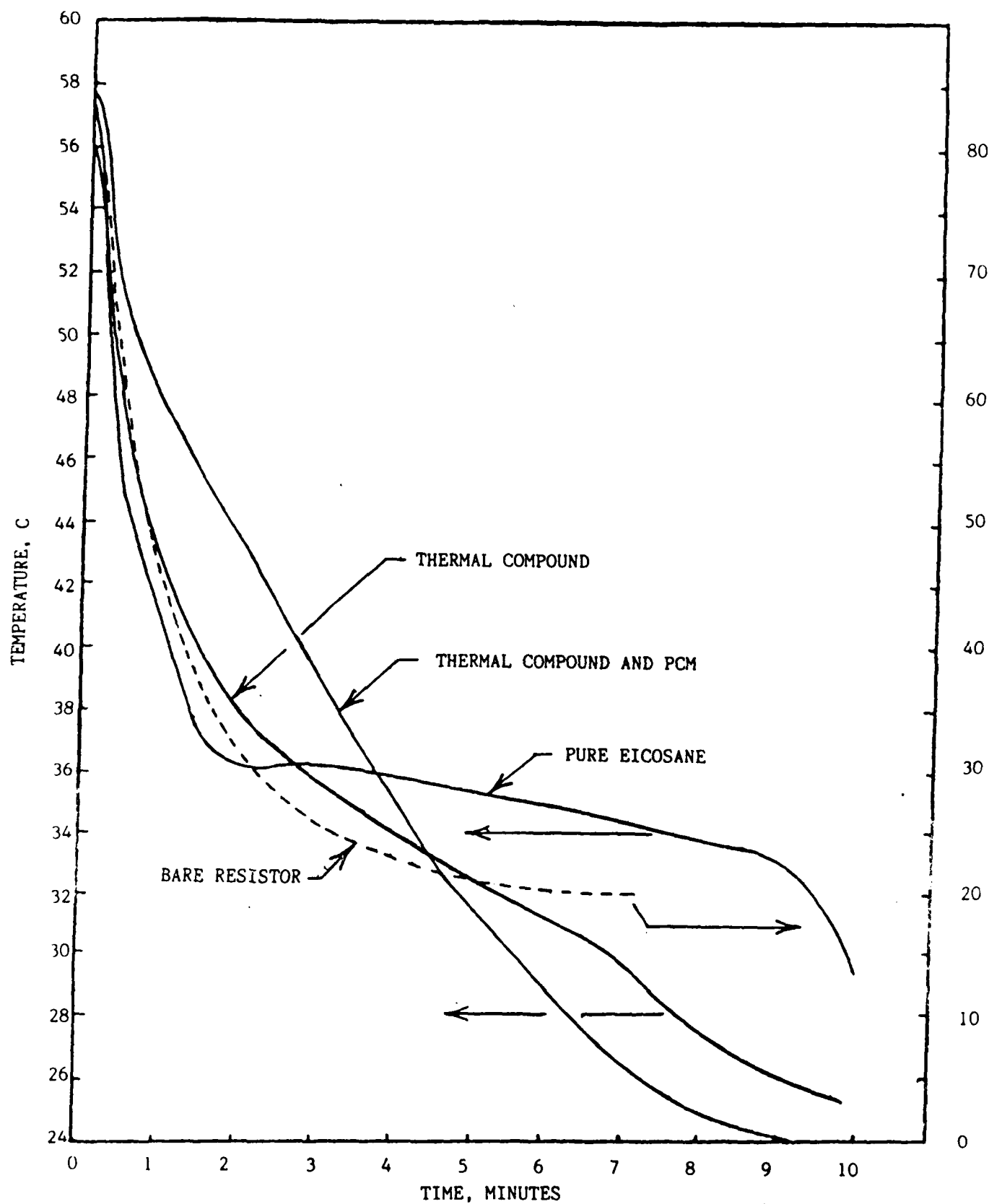
Fig. 11 - Temperature Decay of Resistors of Circuit Number 2 After Sudden Removal of Voltage
