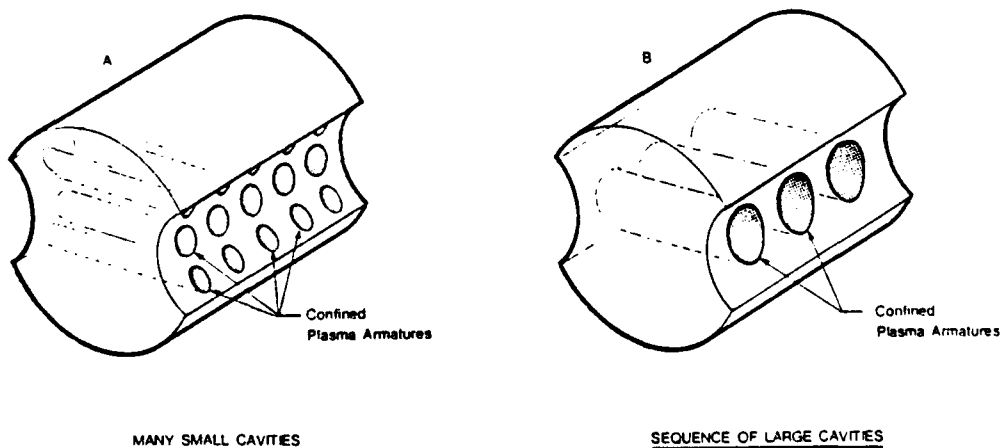
FIGURES 20A & 20B Possible control of current density due to distribution of plasma confining cavities
