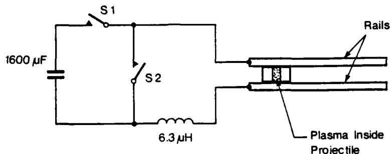
FIGURE 7 Circuit Diagram
