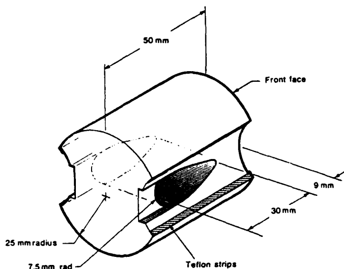
FIGURE 4 Polycarbonate Projectile
