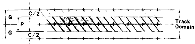
FIG. 6a Representation of a wire-path size of P constructed on a minimum grid increment of size G for clearance C . Actual width of the path of the grid is traced by a 2G \times 2G spot, to give a path size P = 2G - C .
