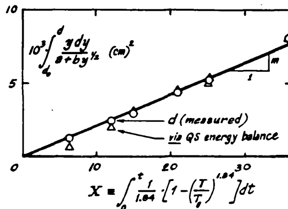
Fig. 3: Straight line plot for testing the dependence of soot deposition rate on surface- and gas-temperature. 3
