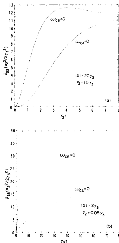
FIG. 5. The transient behavior of the upper state population \tilde{\rho}_{33}(t) at the two resonance peaks \omega_{CB}=0 and \omega_{CA}=0 for the same situation as in Fig. 4. The short bar on the right-hand side indicates a steady-state value which is independent of initial atomic conditions and is the same for the two peaks. The population is measured in units of \alpha_2^2/(2\gamma_3^2) which is always assumed to be much less than unity.
