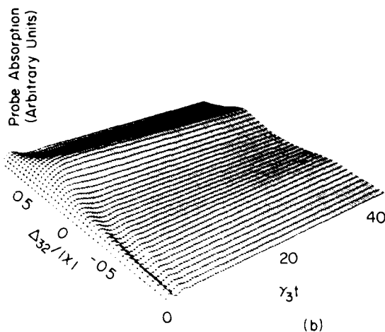
FIG. 8. The transient probe absorption ( -\text{Im}\tilde{\rho}_{12} ) spectra as a function of both probe detuning ( \Delta_{32}/|\chi| ) and time ( \gamma_3 t ) for the same situation and initial conditions as in Fig. 4, namely, \Delta_{21}=0 , \tilde{\rho}_{HH}(0)=1 , and (a) |\chi|=2\alpha_1=20\gamma_3 , \gamma_2=1.5\gamma_3 , (b) |\chi|=2\alpha_1=2\gamma_3 , \gamma_2=0.05\gamma_3 . The transient probe response is plotted up to only half of the time range in Figs. 4–7 and, consequently, has not yet arrived at the steady-state spectra which are independent of initial conditions and are given in Fig. 2.
