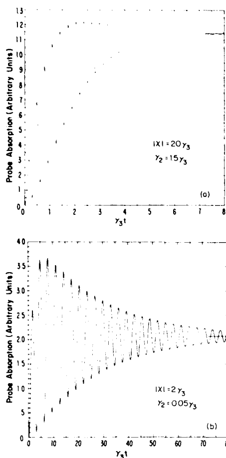
FIG. 6. Same as in Fig. 4 except that the initial conditions are now \tilde{\rho}_{AA}(0) = \tilde{\rho}_{BB}(0) = \tilde{\rho}_{BA}(0) = \frac{1}{2} , i.e., \tilde{\rho}_{11}(0) = 1 . The probe absorption is the same at the resonance peaks \omega_{CB} = 0 and \omega_{CA} = 0 owing to the resonant dressing field and the symmetry in the initial conditions in the DAP.
