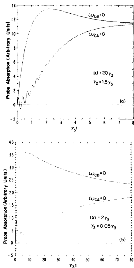
FIG. 4. The transient probe absorption [-\text{Im}\tilde{\rho}_{32}(t)] at the two resonance peaks \omega_{CB}=0 ( \Delta_{32} = |\chi|/2 ) and \omega_{CA}=0 ( \Delta_{32} = -|\chi|/2 ) as a function of \gamma_3 t when a strong pump (dressing) field is exactly on resonance with the 1-2 transition ( \Delta_{21}=0 ), the atom is initially in a single dressed state \tilde{\rho}_{BB}(0)=1 , and (a) |\chi|=2\alpha_1=20\gamma_3 , \gamma_2=1.5\gamma_3 , (b) |\chi|=2\alpha_1=2\gamma_3 , \gamma_2=0.05\gamma_3 . The short bars on the right-hand side indicate the steady-state value which is independent of initial conditions and is the same for the two peaks. The choice of parameters of (a) [(b)] apply to all figures (a) [(b)] in Figs. 4–11.
