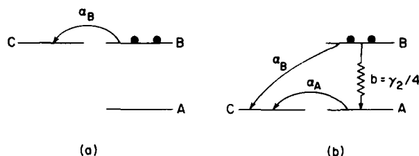
FIG. 3. Energy levels of the three-level system with a strong resonant dressing field and \bar{\rho}_{BB}(0) = 1 in the DAP when the probe is resonant with (a) initially populated state B ( \omega_{CB} = 0 ) and (b) initially unpopulated state A ( \omega_{CA} = 0 ). In (a), the probe absorption builds up proportional to t initially and reaches its steady-state value with no oscillation. In (b), except for a small oscillatory component arising from a nonresonant direct coupling between levels B and C , the probe absorption builds up, on average, proportional to t^2 initially via the level coupling B \rightarrow A \rightarrow C . The probe absorption in (a) ( \omega_{CB} = 0 ) is much larger than that in (b) ( \omega_{CA} = 0 ) at early times. In this figure, \alpha_A and \alpha_B give the probe coupling strengths, while b is the rate of transfer of population from state B to A .
