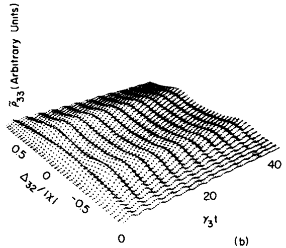
FIG. 11. Same as in Fig. 9 except that the initial conditions are now \tilde{\rho}_{AA}(0) = \tilde{\rho}_{BB}(0) = \tilde{\rho}_{BA}(0) = \frac{1}{2} and the transient response at the peaks are given in Fig. 7. The spectra are symmetric about zero probe detuning.
