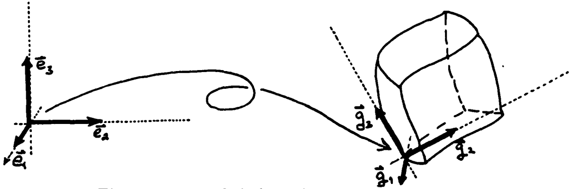
Figure 2.1: The body frame is translated and rotated with respect to the inertial frame.
