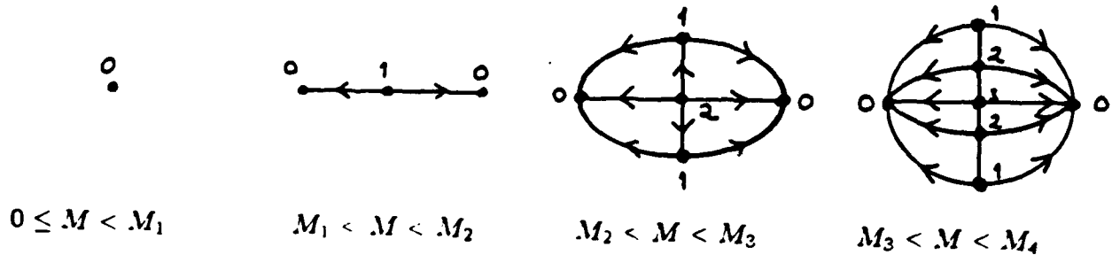
Figure 6.4. Global phase portrait of the system (6.7),(6.8). Indices show the dimension of the unstable manifolds, which are depicted by arrows.
