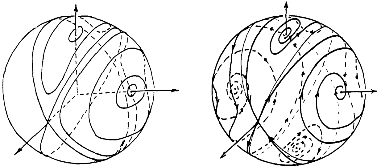
Figure 5.2: Momentum spheres in the conservative and dissipative cases.
