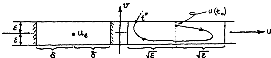
Figure 6.5 Solutions which remain \epsilon -close to \{v = 0\} must be \delta -close to a stationary point.
