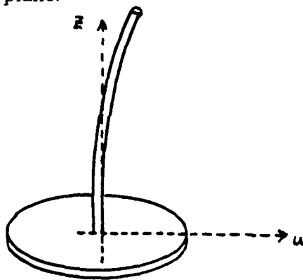
Figure 6.1: A model problem with 1 rotational d.o.f.
