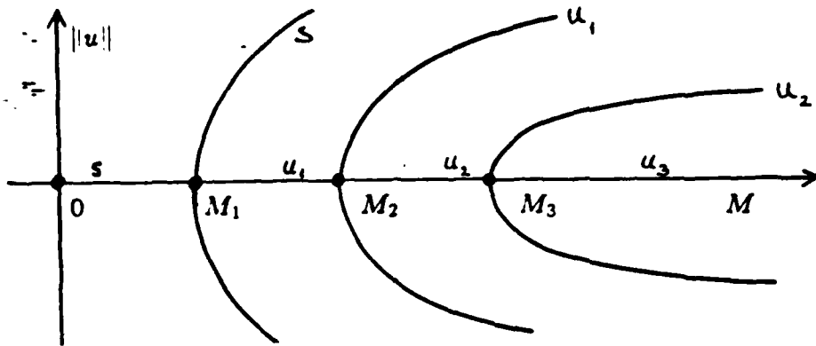
Figure 6.3 s denotes stable equilibria, and u_1, u_2, \dots denote unstable equilibria with 1, 2, \dots dimensional unstable manifolds. The numbers and L^2 -norm of equilibria depend on the parameter M .
