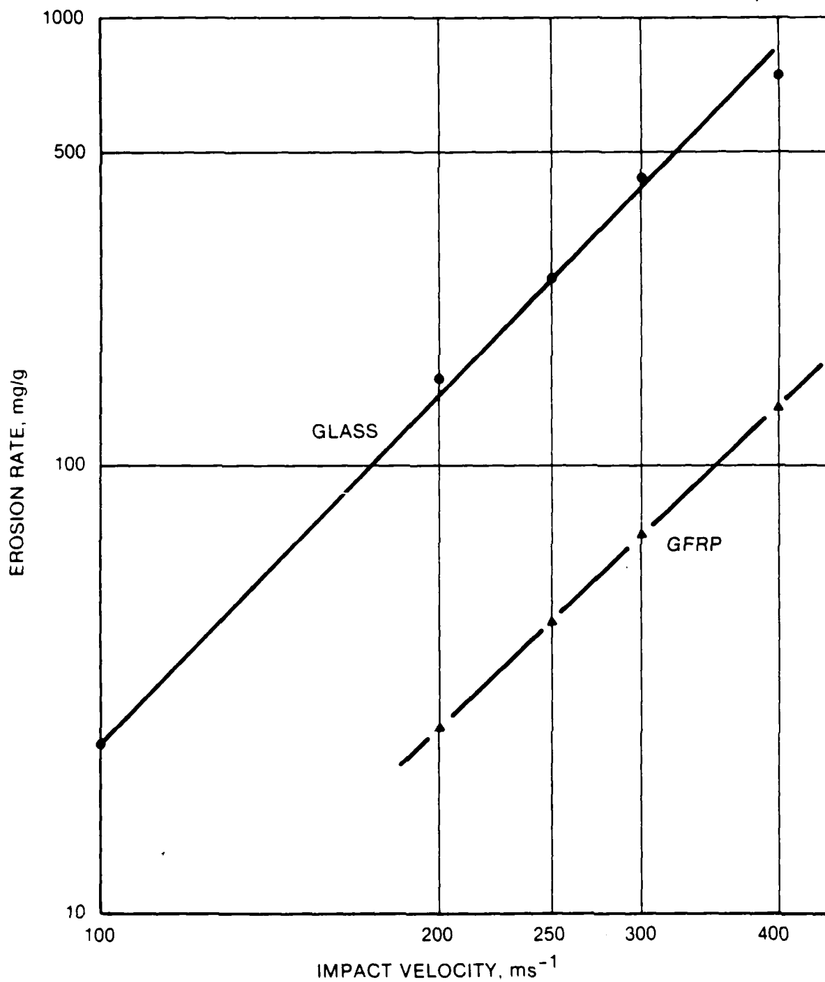
Figure 7. Steady-state erosion rates for graphite-fiber reinforced epoxy as a function of particle impact velocity (Behrendt, (1974).
