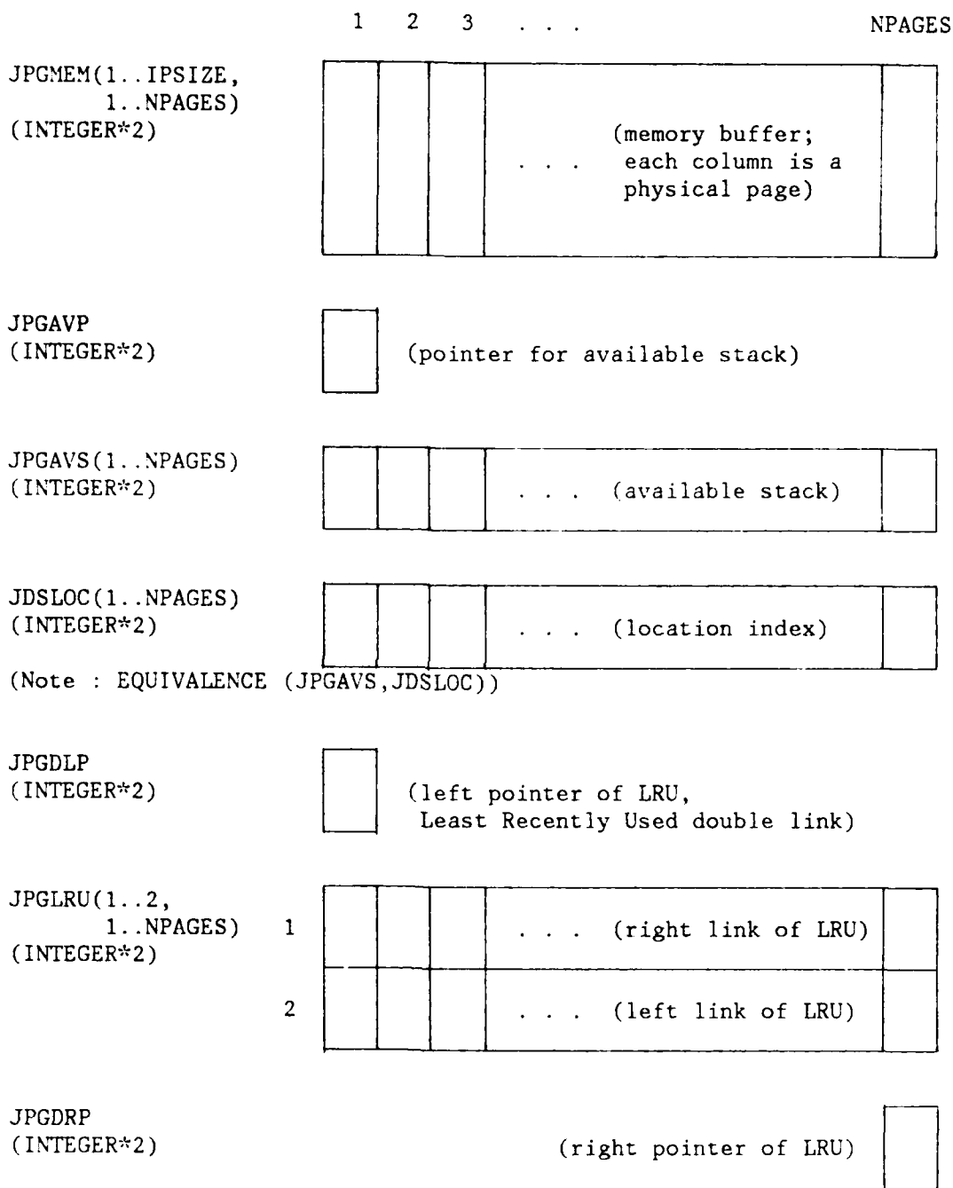
Figure 6.5. Layout of MMS Information Table for MMS in MIDAS/N Version 2.0 (Part 1)
