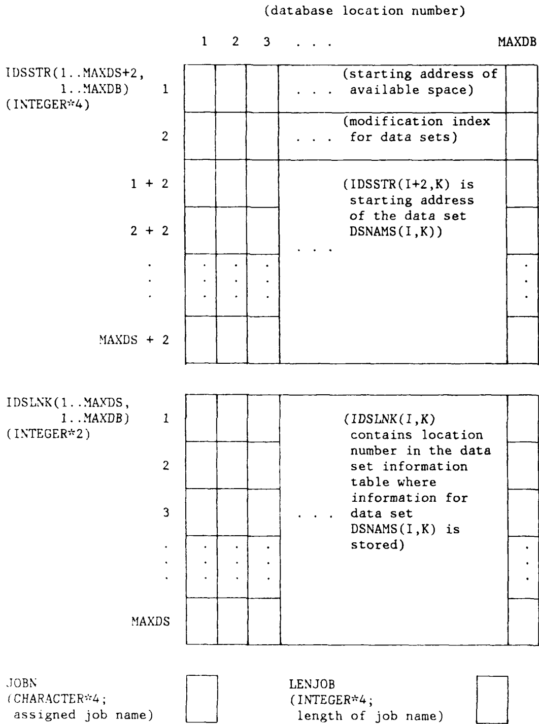
Figure 4.2. Layout of APIPS Information Table (Part 2)
