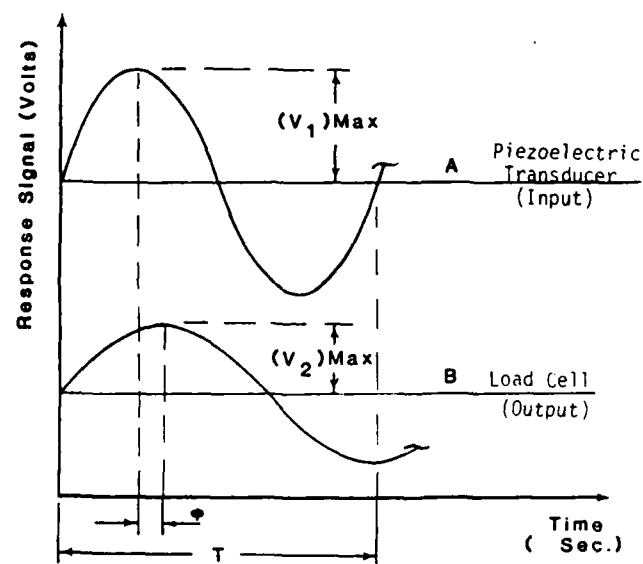
Figure E-2c. Sample Measurements for Simplified Steady State Approach
