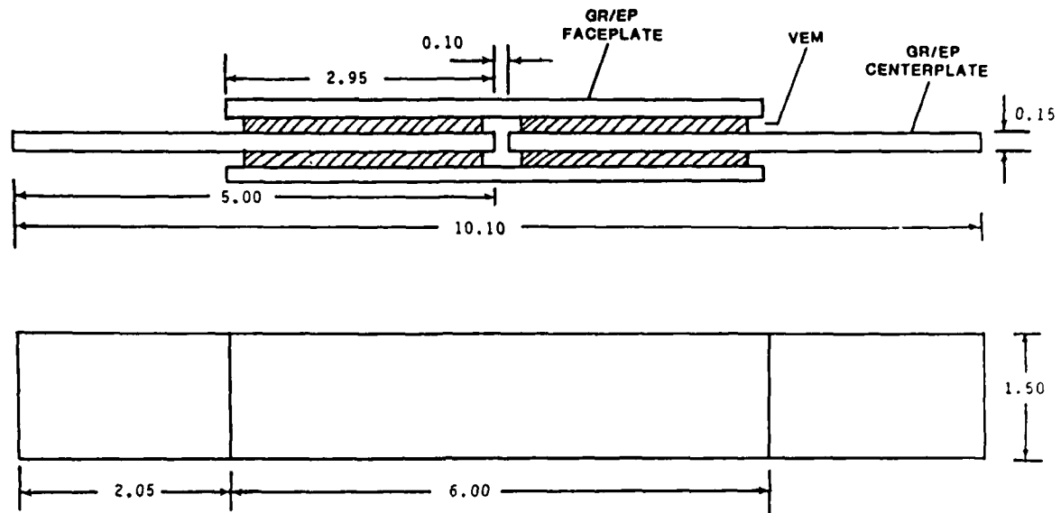
Figure 7a. Passively Damped Joint Specimen Without Elastic Link Between Members
