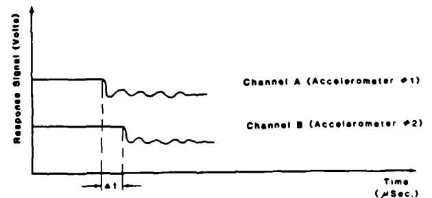
EXAMPLE OF DISPLAY FOR STIFFNESS MEASUREMENT
