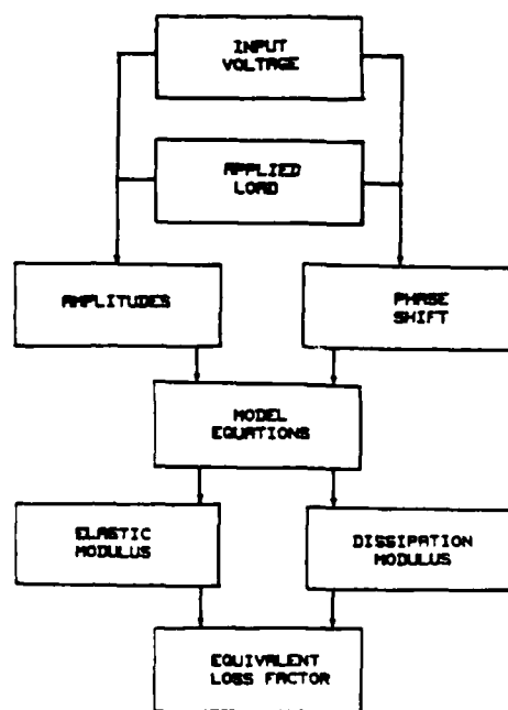
Figure E-2b. Data Analysis Flow for Simplified Steady State Approach
