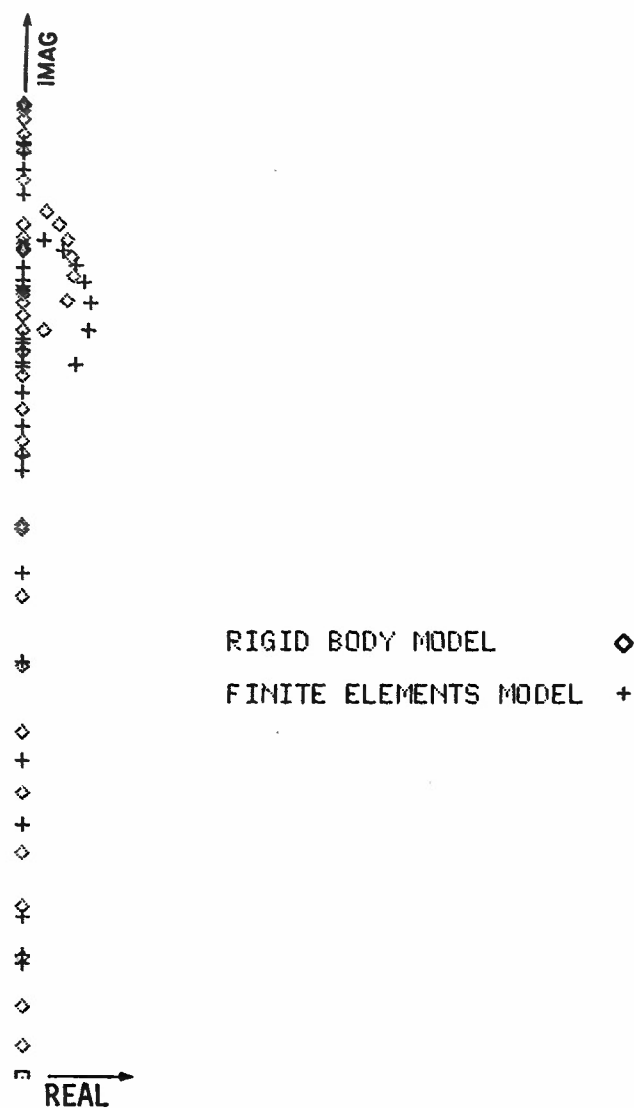
Figure 79. Comparison of the eigenvalues associated with "normal and rotational displacements" obtained with the rigid body and the finite elements model.
