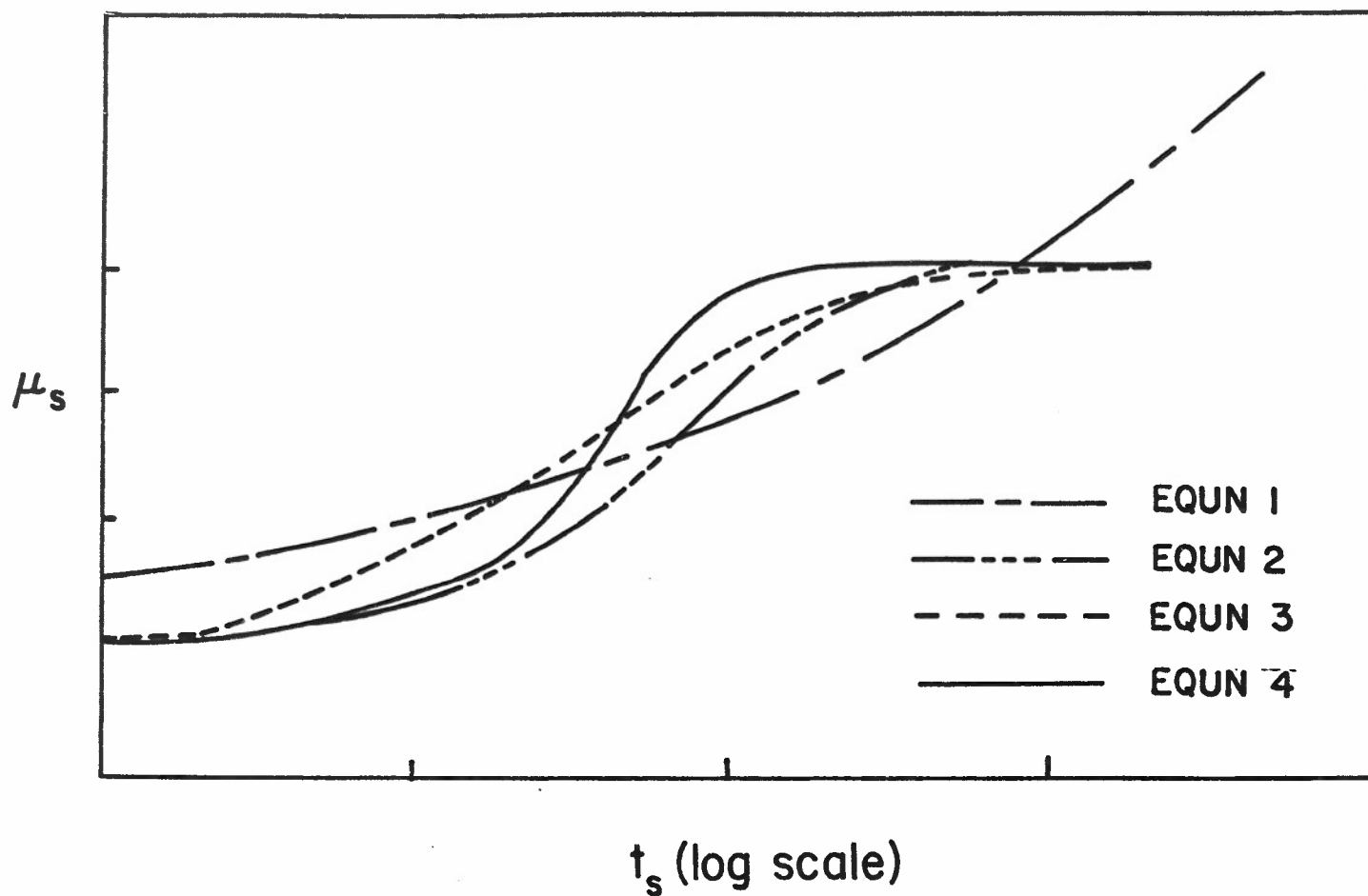
Figure 27. Coefficient of static friction vs. time of stationary contact; equations from the literature (see TABLE 1). (RICHARDSON and NOLLE [1976])
