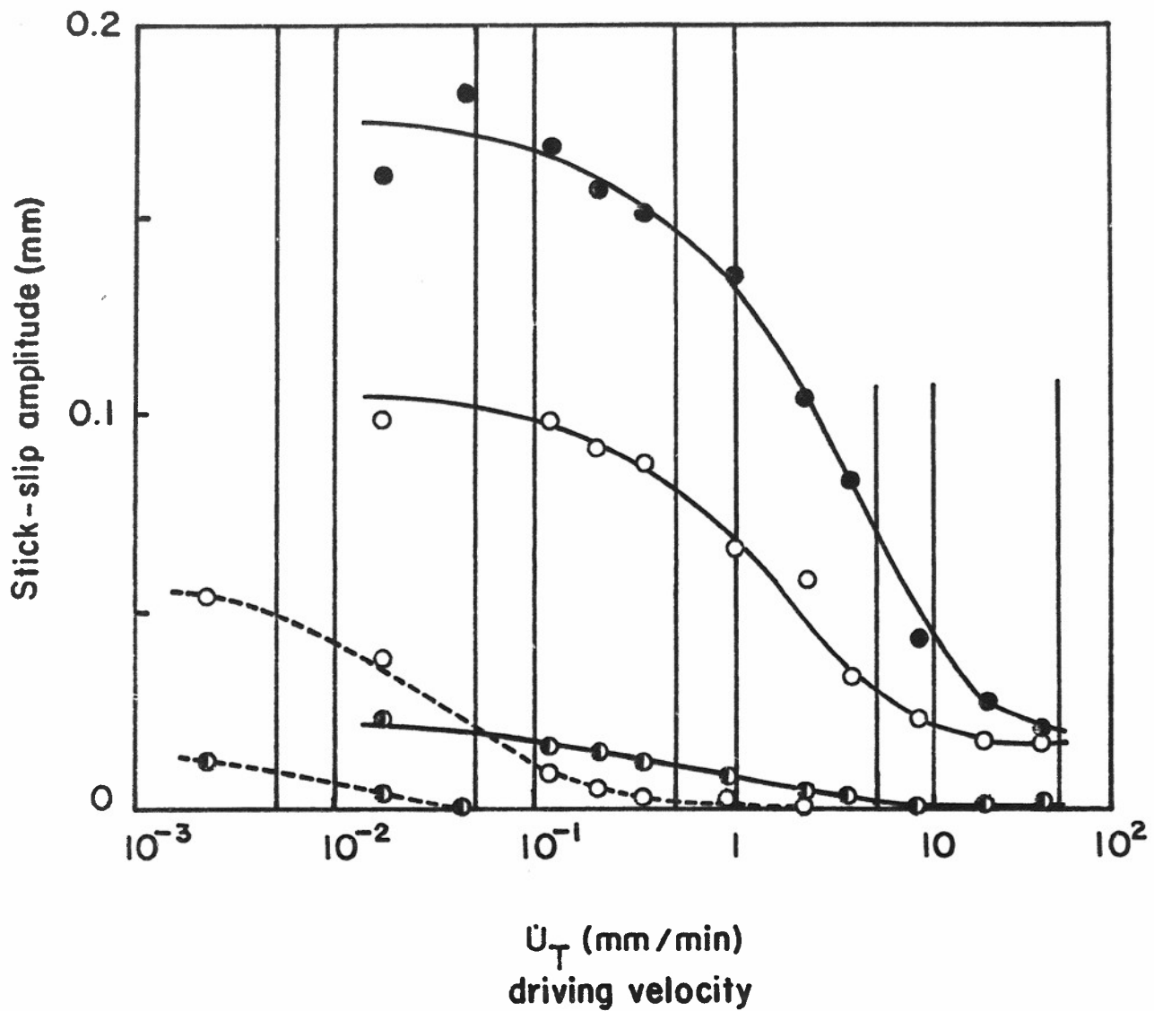
Figure 34 . Relation between amplitude of the stick-slip motion and driving velocity for various masses of the slider.
