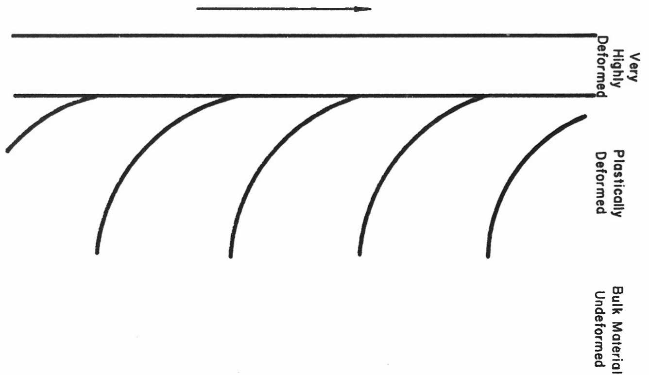
Figure 19. Longitudinal section of a wear specimen.
