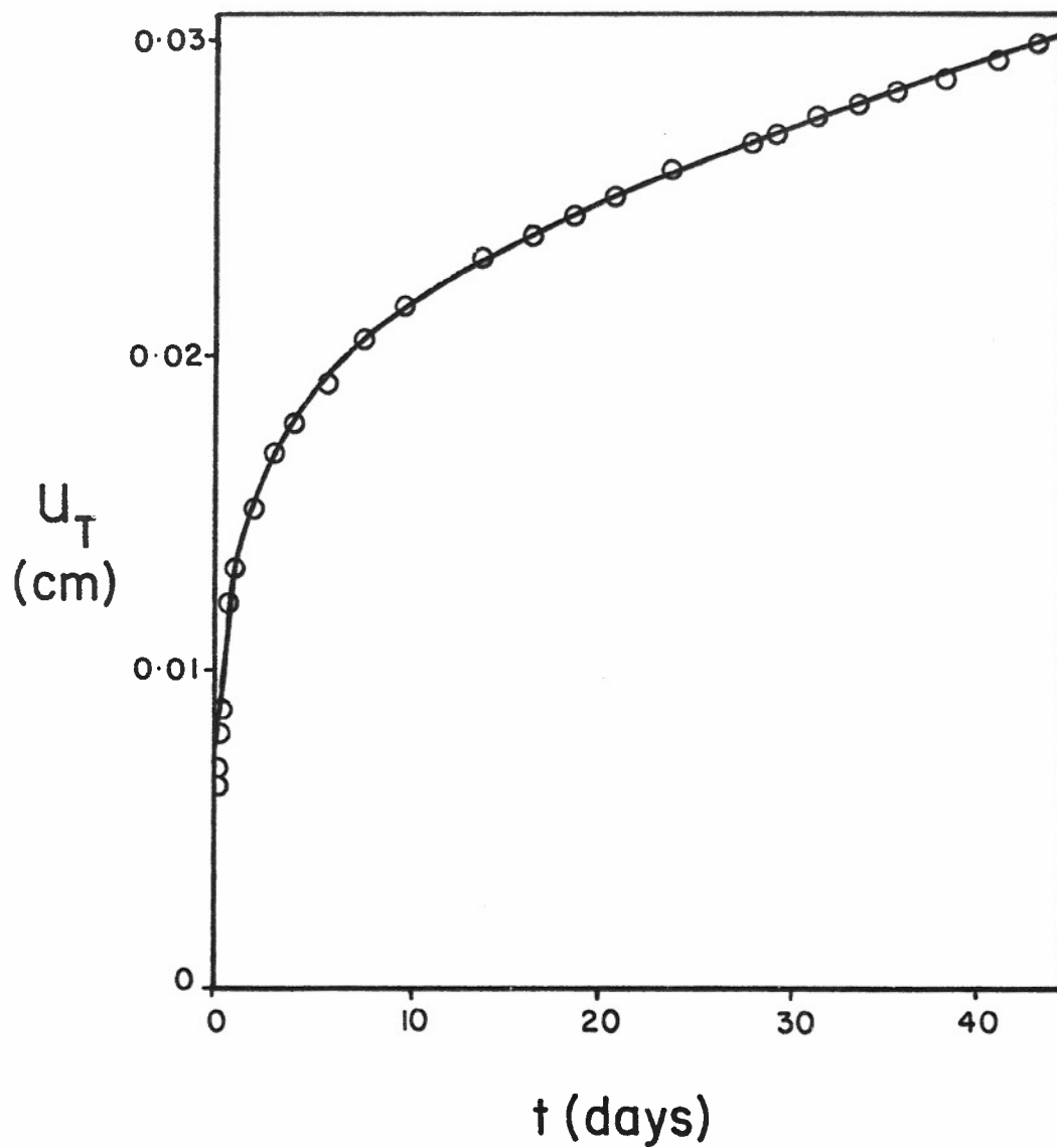
Figure 24. Creep Sliding.
