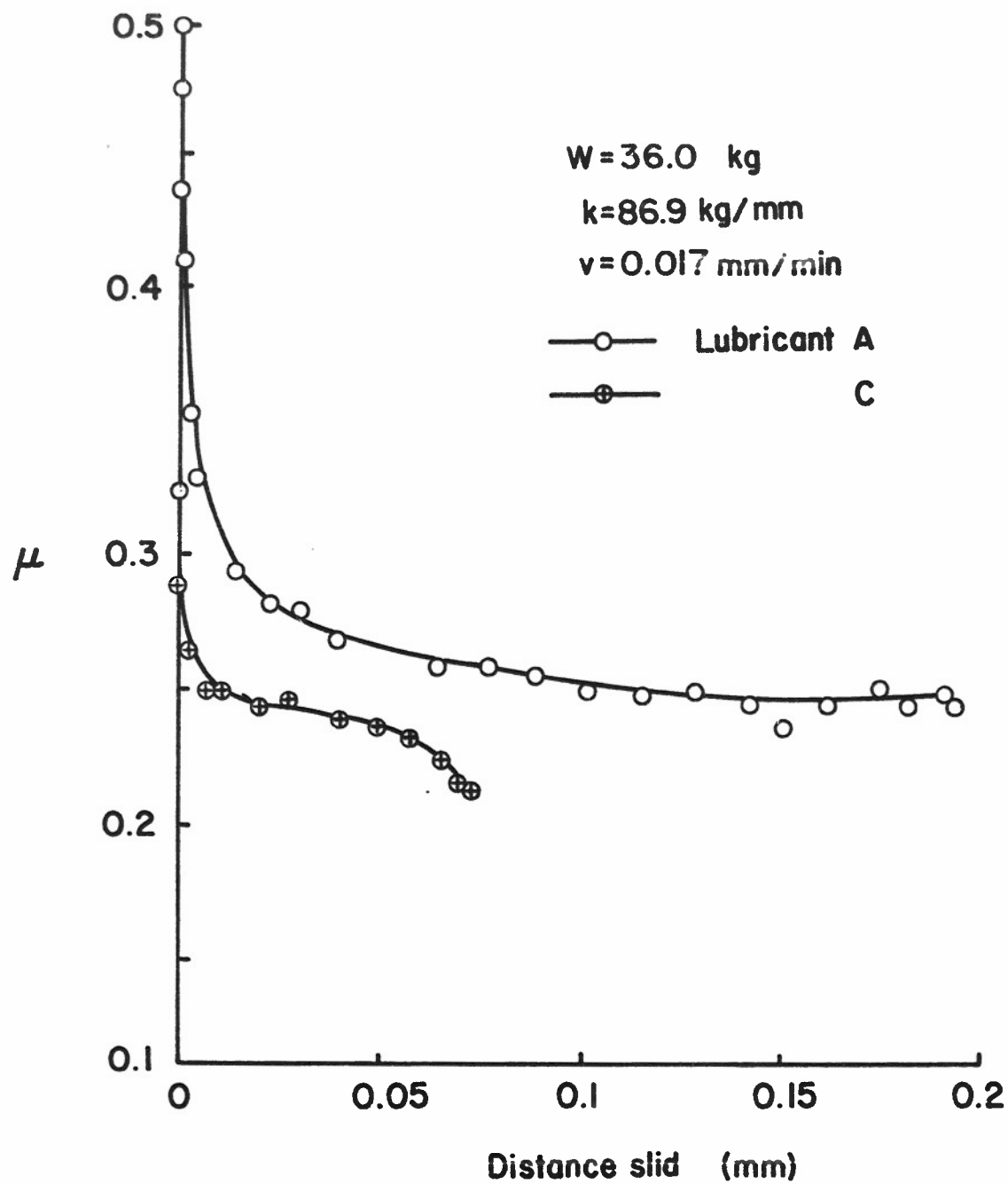
Figure 40. Relation between coefficient of friction and distance slid in a stick-slip experiment.
