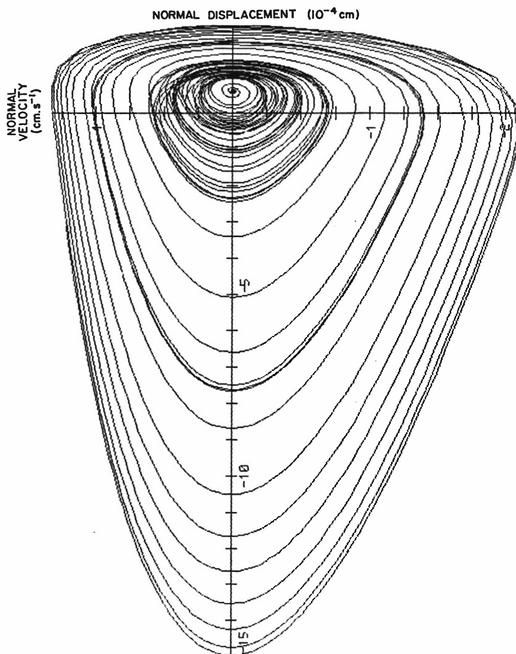
Figure 68. Phase plane plot of the initial part of the normal oscillation of the center of mass ( \mu = 1 ).
