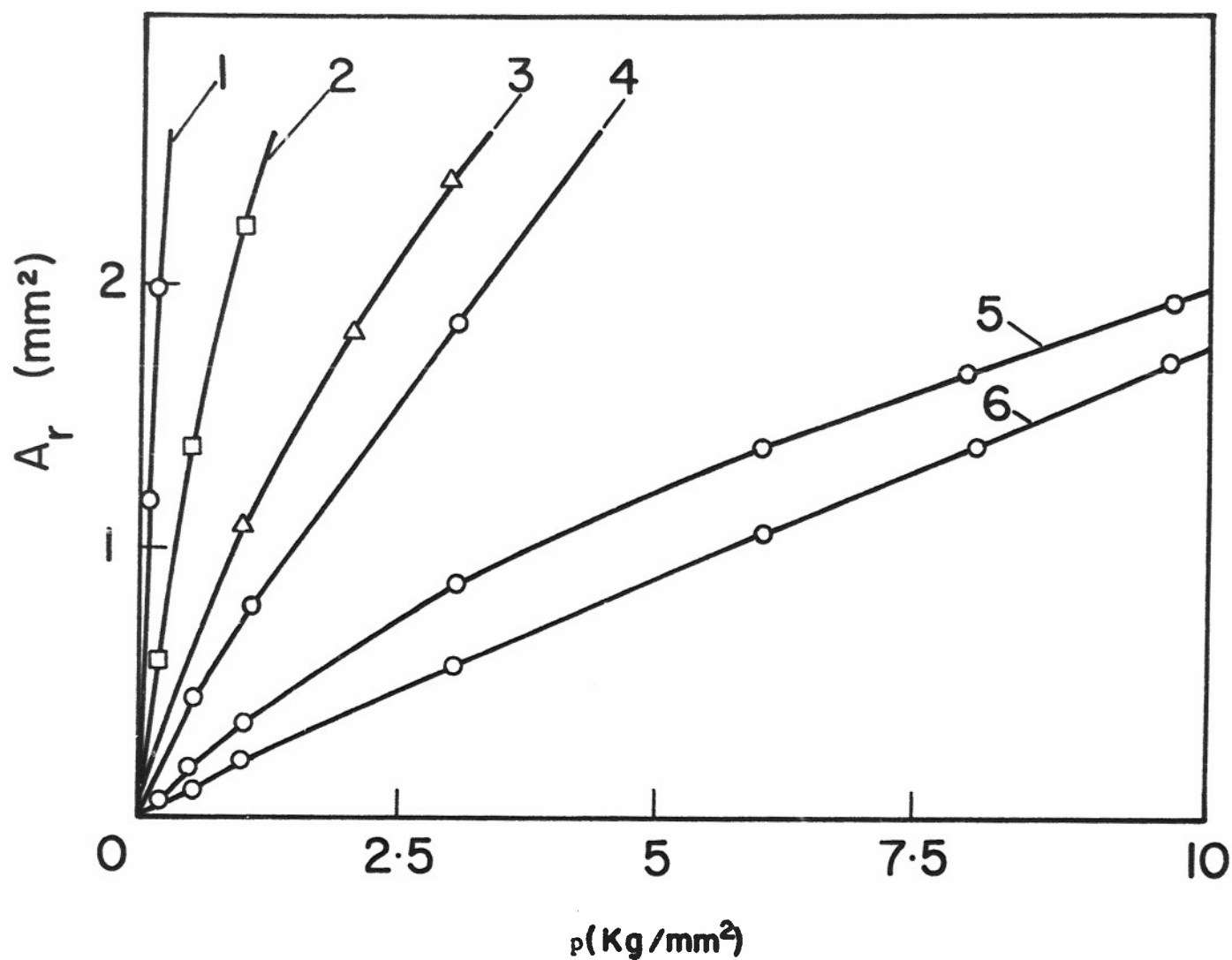
Figure 11. Real area of contact vs. pressure for different metals in contact with a glass prism.
