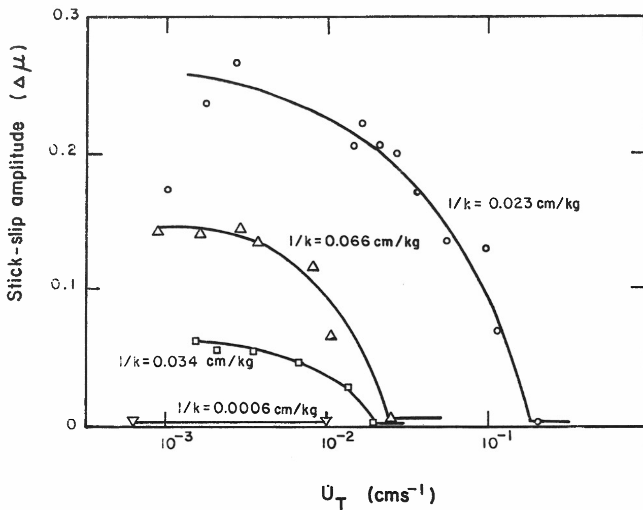
Figure 33. Relation between amplitude of the stick-slip motion and driving velocity for various spring stiffnesses (K).
