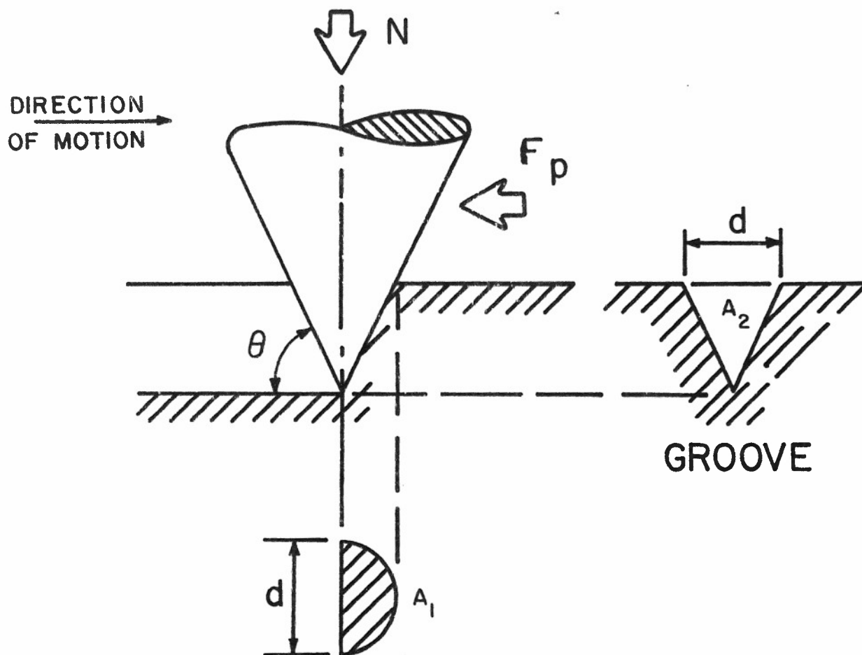
Figure 18. Plowing component of friction for a cone sliding on a softer metal.
