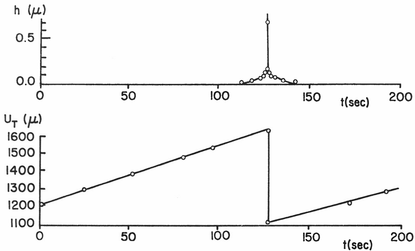
Figure 46. Simultaneous tangential ( u_T vs. t ) and normal ( h vs. t ) jumps of the slider during stick-slip motion. Unlubricated. (TOLSTOI [1967]).
