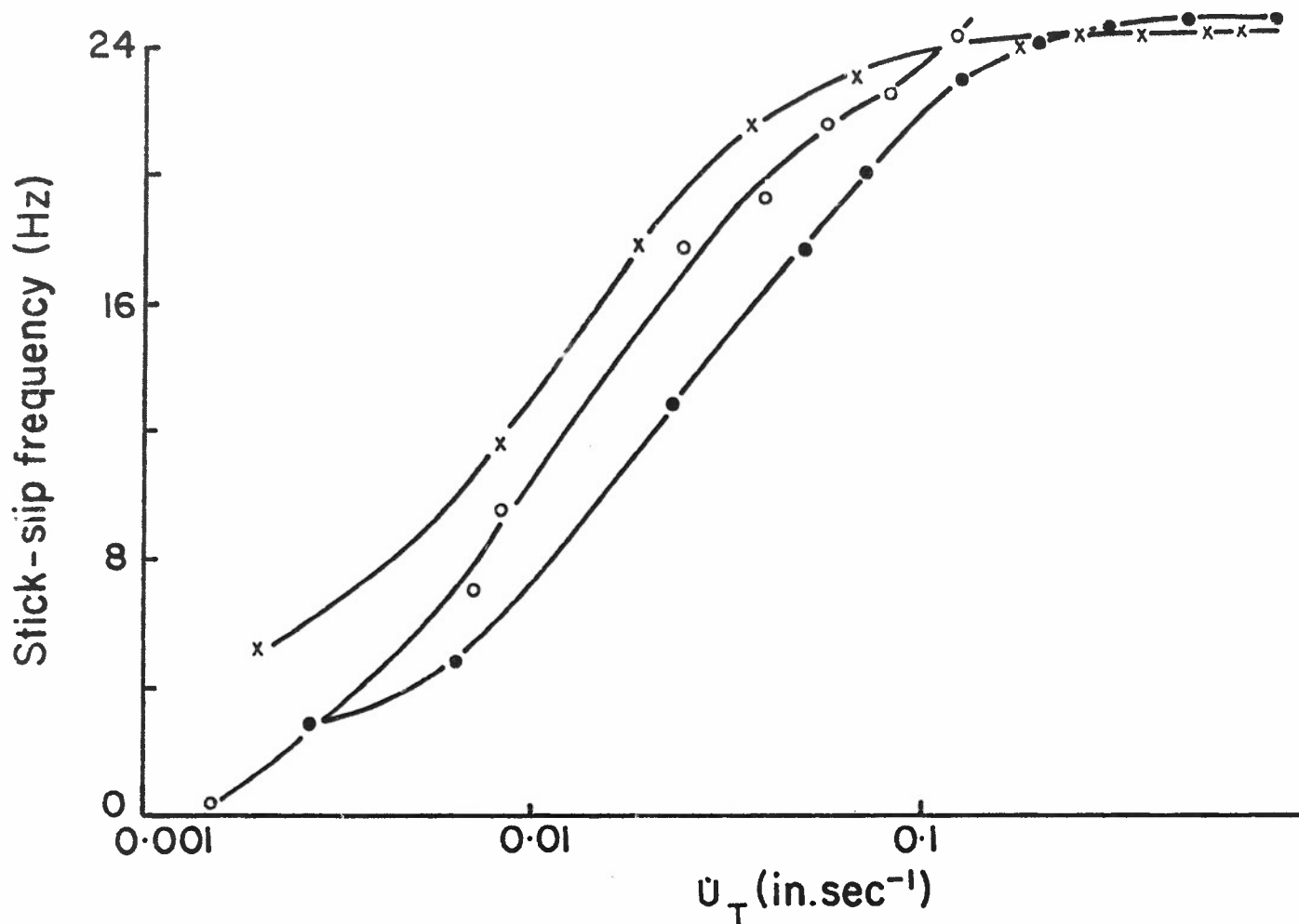
Figure 37. Variation of stick-slip frequency with driving velocity for various lubrication conditions.
