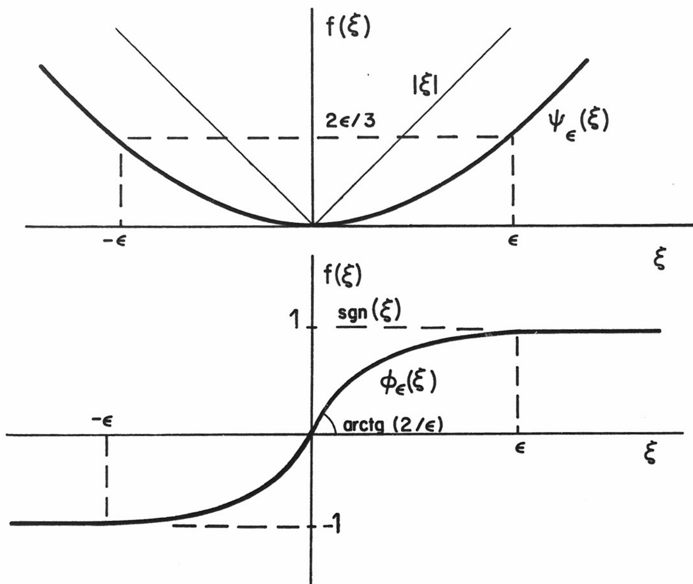
Figure 50. Graphs of the function \psi_\epsilon and \phi_\epsilon for the case of unidimensional \Gamma_C .
