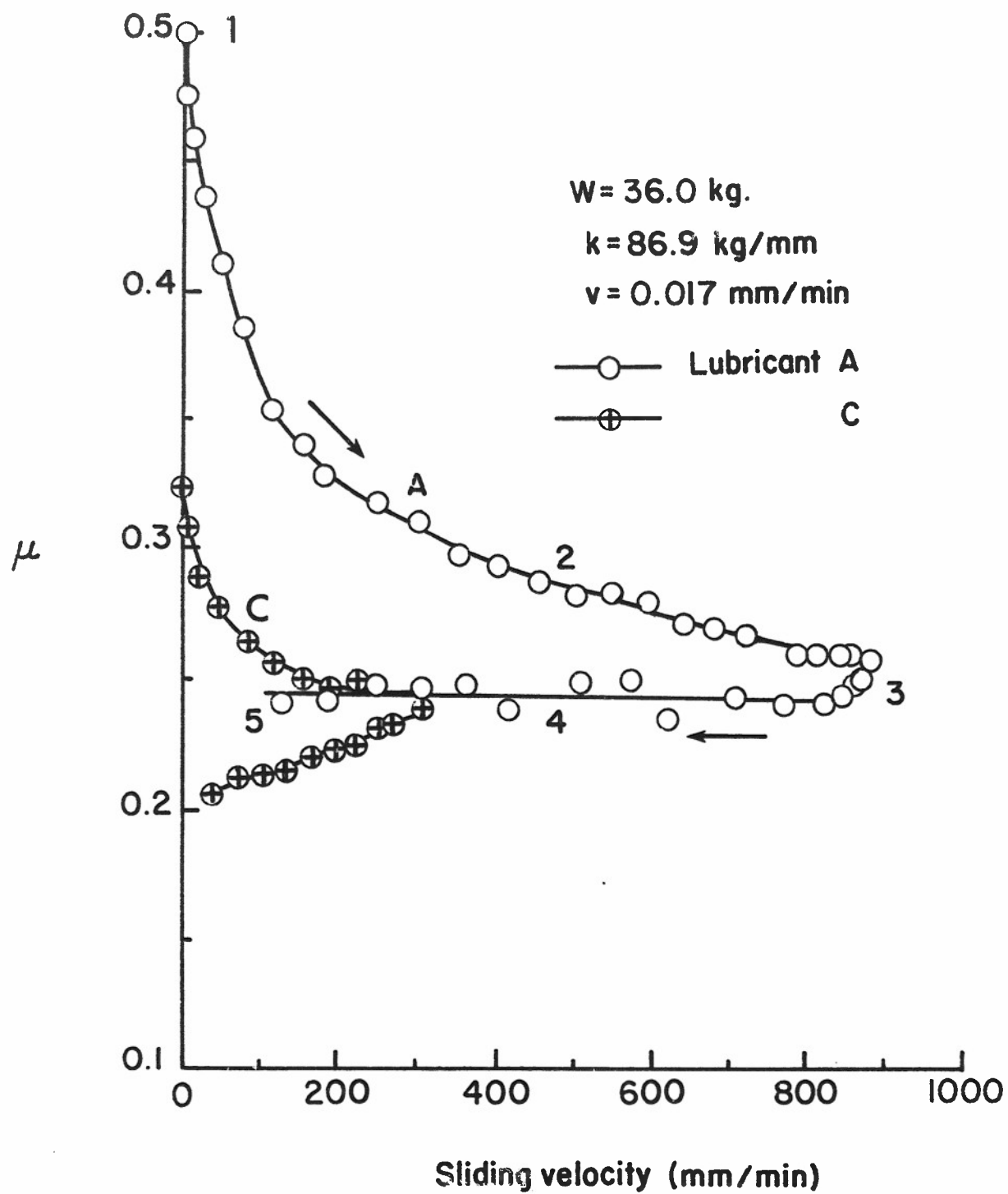
Figure 43. Coefficient of friction versus sliding velocity. (KATO, YAMAGUCHI and MATSUBAYASHI [1970]).
