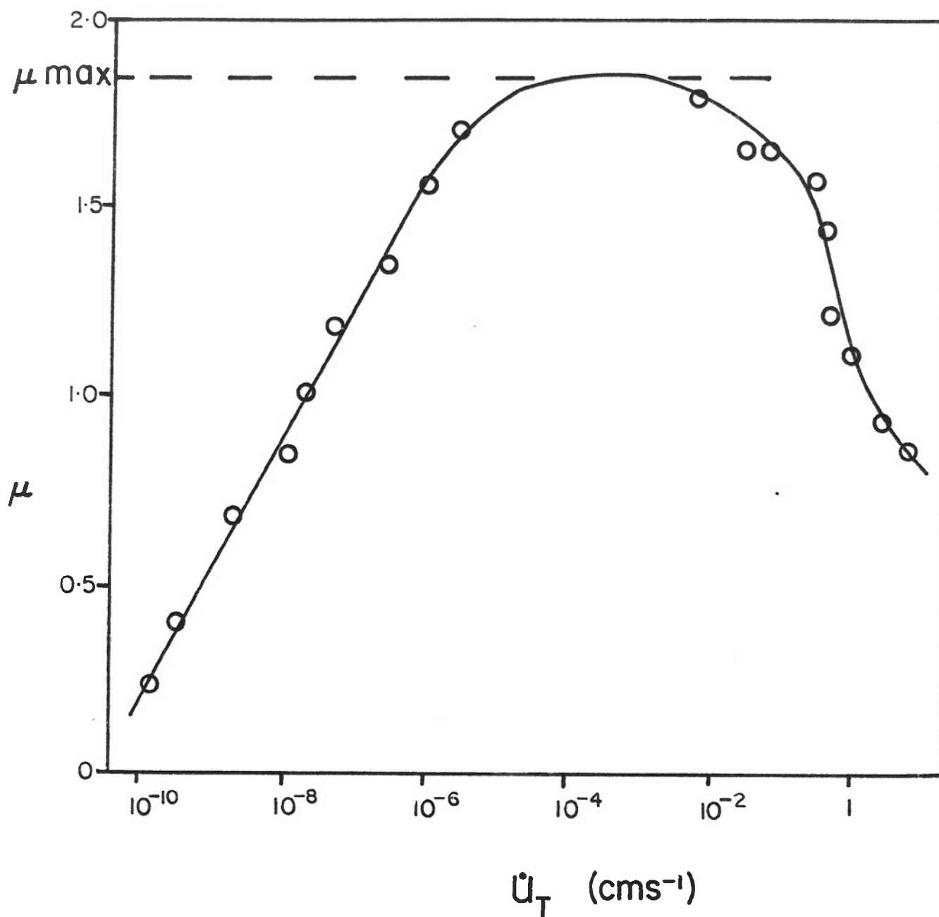
Figure 25. Coefficient of friction as a function of final sliding velocity.
