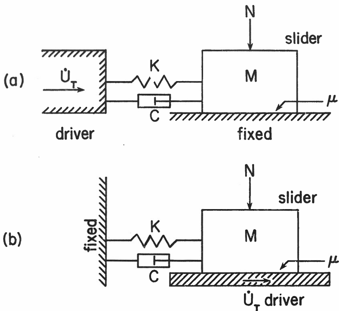
Figure 30. Models of two (equivalent) sliding systems which may have stick-slip oscillations.
