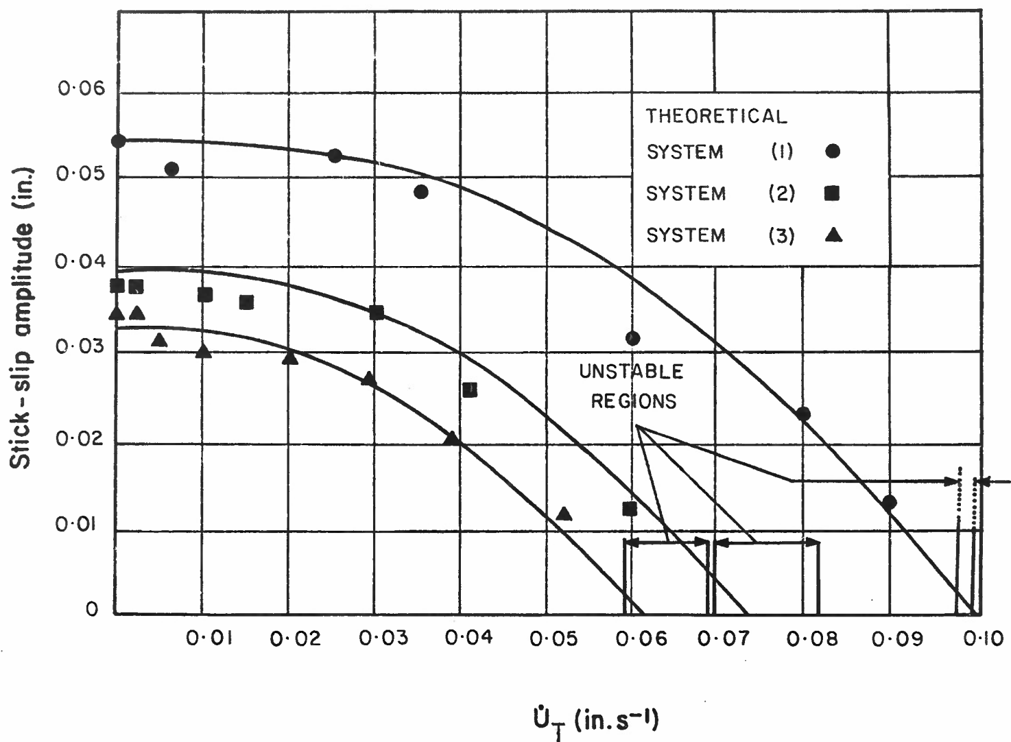
Figure 32. Relation between amplitude of the stick-slip motion and velocity for various damping coefficients.
