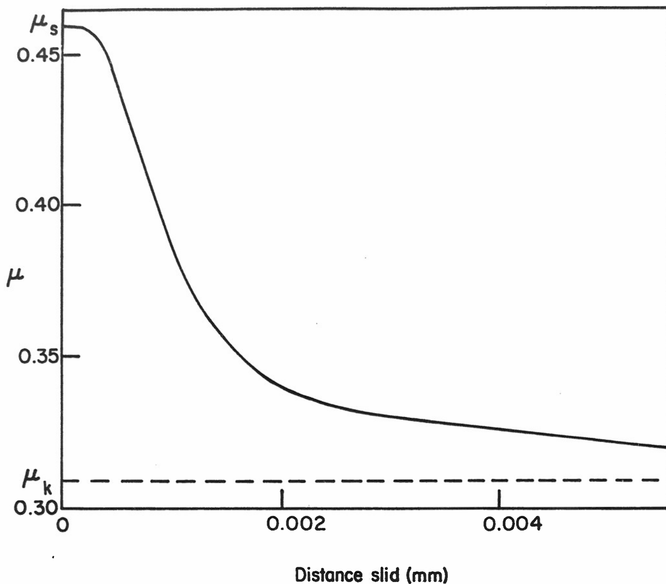
Figure 39. Relation between coefficient of friction and distance slid in an impact experiment.
