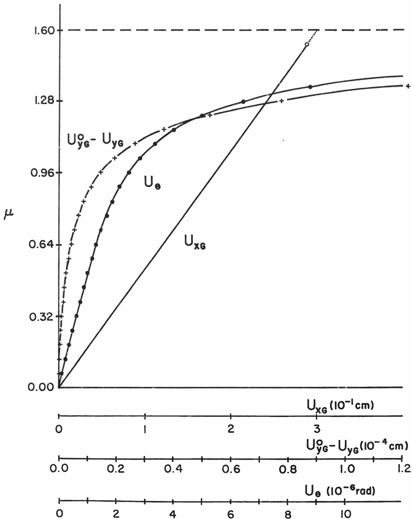
Figure 62. Equilibrium Displacements of a Rigid Block in Steady Sliding on a Moving Belt for the Admissible Values of the Coefficient of Friction.
