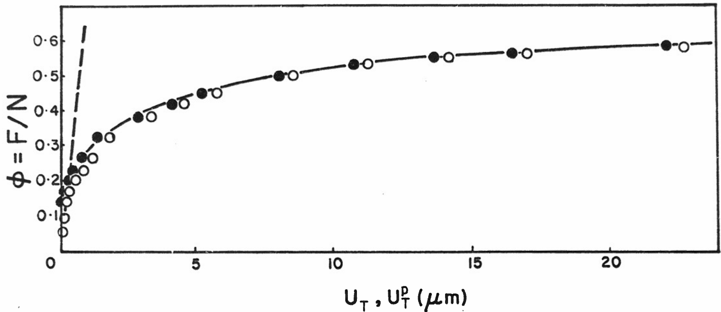
Figure 22. The irreversible part of the tangential displacement.
