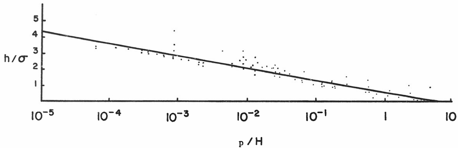
Figure 14. Dimensionless separation vs. dimensionless load. Regression line obtained on the basis of the experimental results of 7 different papers by various authors. (WOO and THOMAS [1980]).
