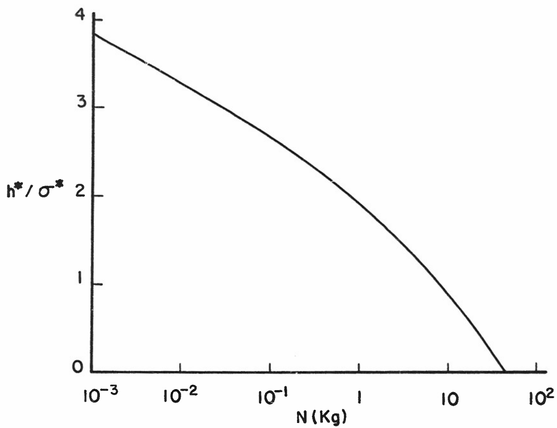
Figure 7. Relation between separation and load. (GREENWOOD and WILLIAMSON [1966]).
