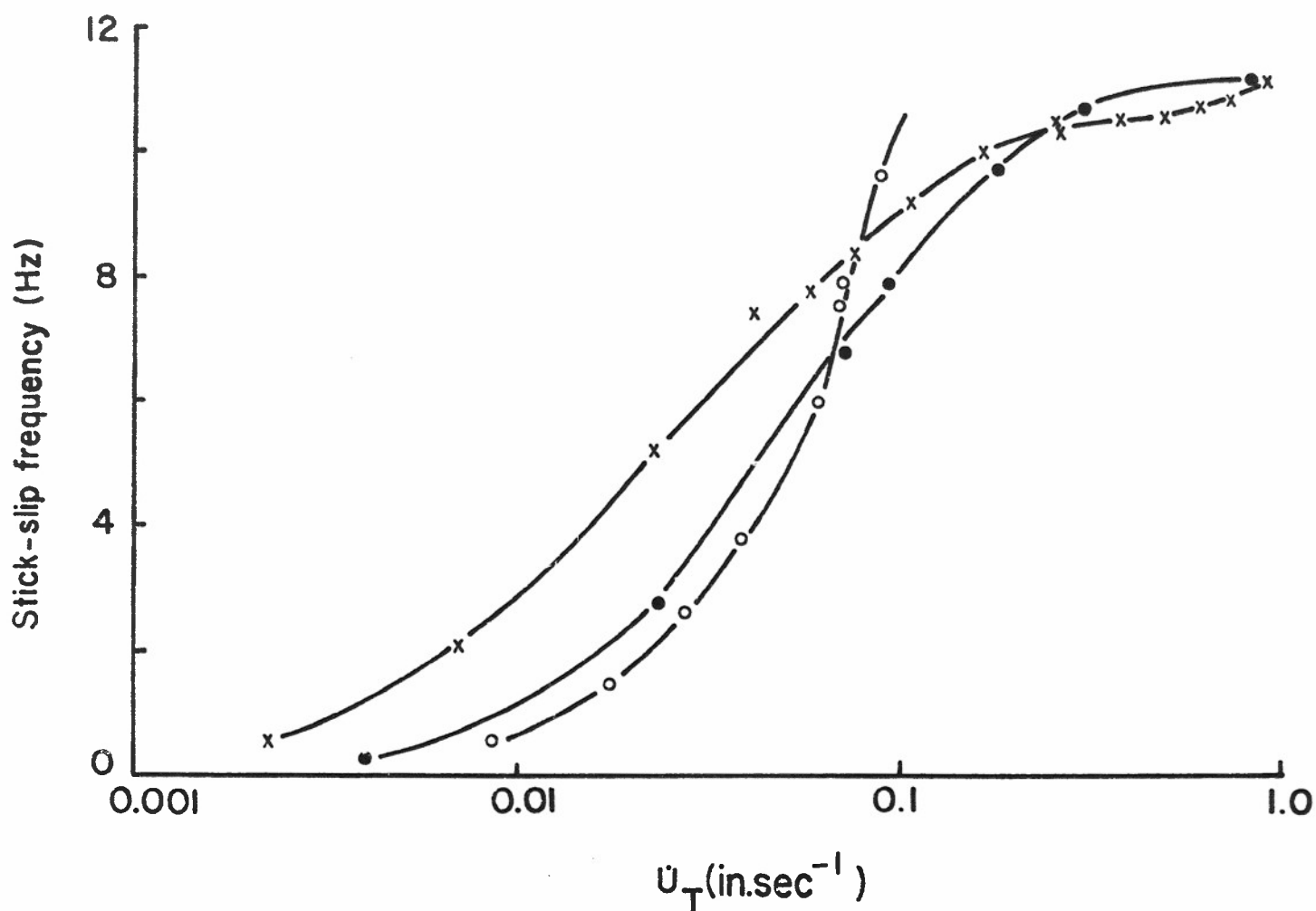
Figure 36. Variation of stick-slip frequency with driving velocity for various lubrication conditions.
