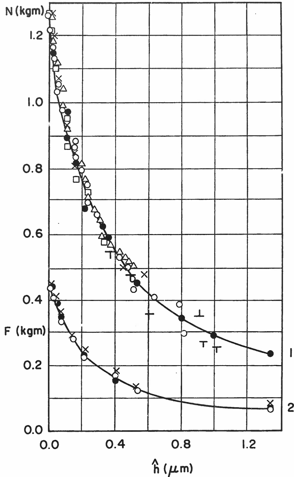
Figure 44. Normal load ( N , curve 1) and static friction force ( F , curve 2) versus the separation \hat{h} (arbitrarily \hat{h} is taken to be zero for the maximum normal load used in the experiments). Dry steel surfaces. (TOLSTOI [1967]).
