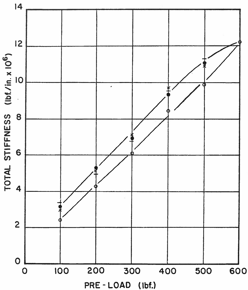
Figure 16. Variation of Dynamic Stiffness with Pre-load.
