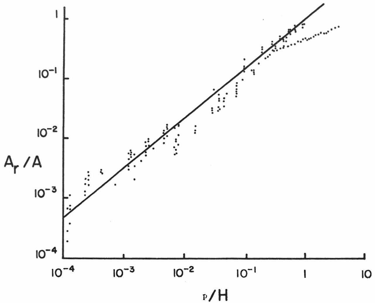
Figure 13. Bearing area ratio vs. dimensionless load.
