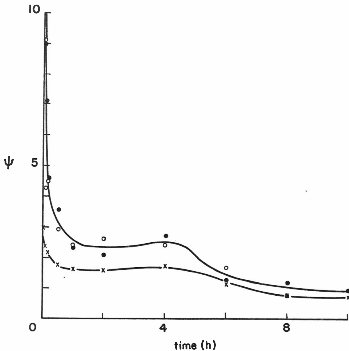
Figure 10. Effect of continued sliding on the plasticity index.
