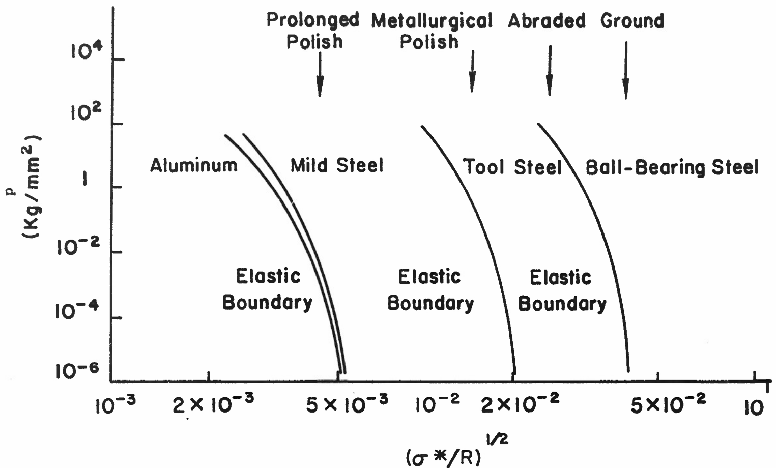
Figure 15. Nominal pressure at which the transition from elastic to plastic deformation occurs for a flat metal of specified roughness pressed on to a flat ideally smooth hard surface.
