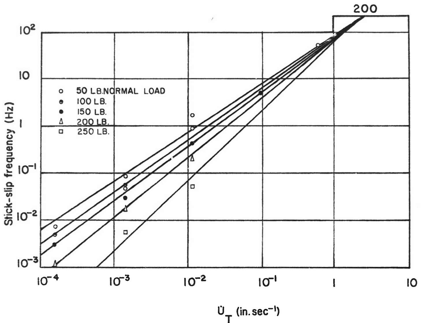
Figure 35. Variation of stick-slip frequency with driving velocity for various normal loads.
