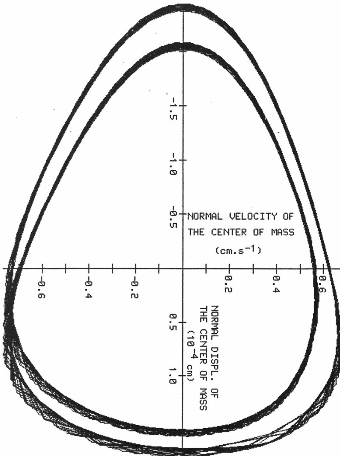
Figure 74. Phase plane plot of the steady normal oscillation obtained during apparently smooth sliding with an apparent coefficient of kinetic friction lower than the coefficient of static friction ( \mu = 1 , \dot{u}_x^C = 0.287 \text{ cm s}^{-1} )
