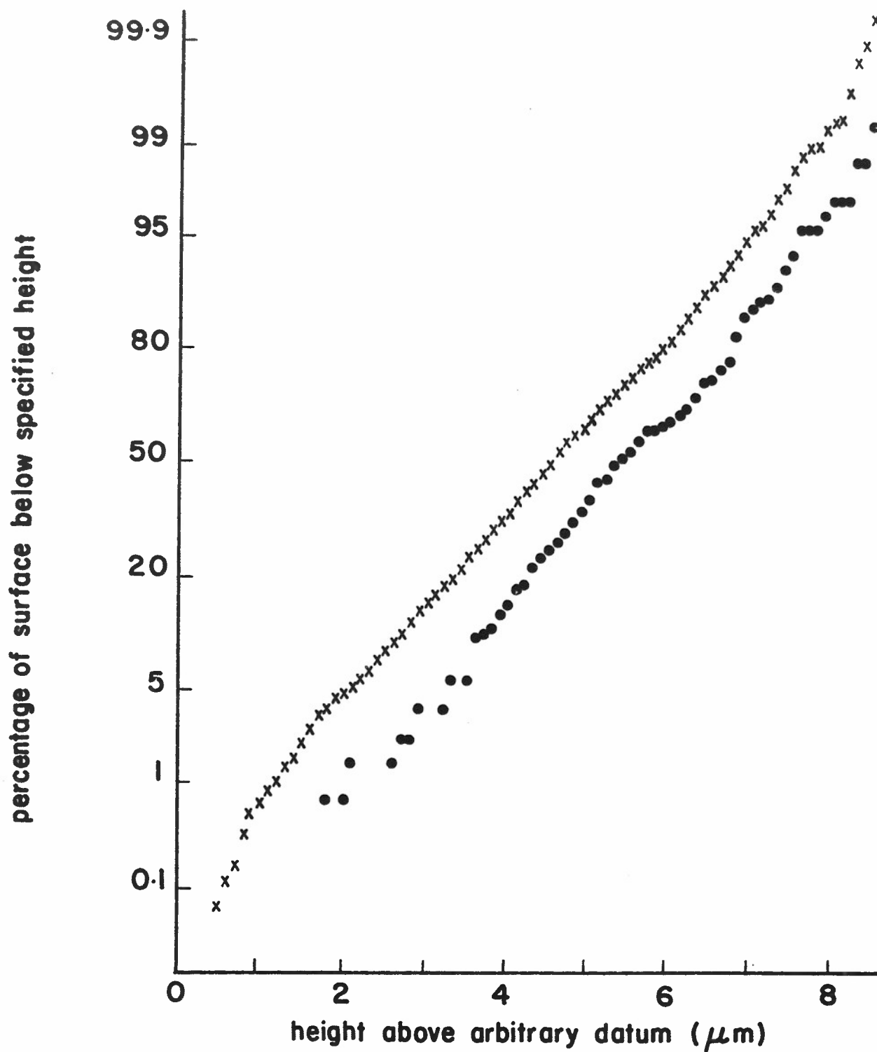
Figure 6. Cumulative height distribution of bead-blasted aluminum. (x) Distribution of all heights (•) Distribution of peak heights A perfect Gaussian distribution would give, with the vertical scale used, a straight line. (GREENWOOD and WILLIAMSON [1966]).
