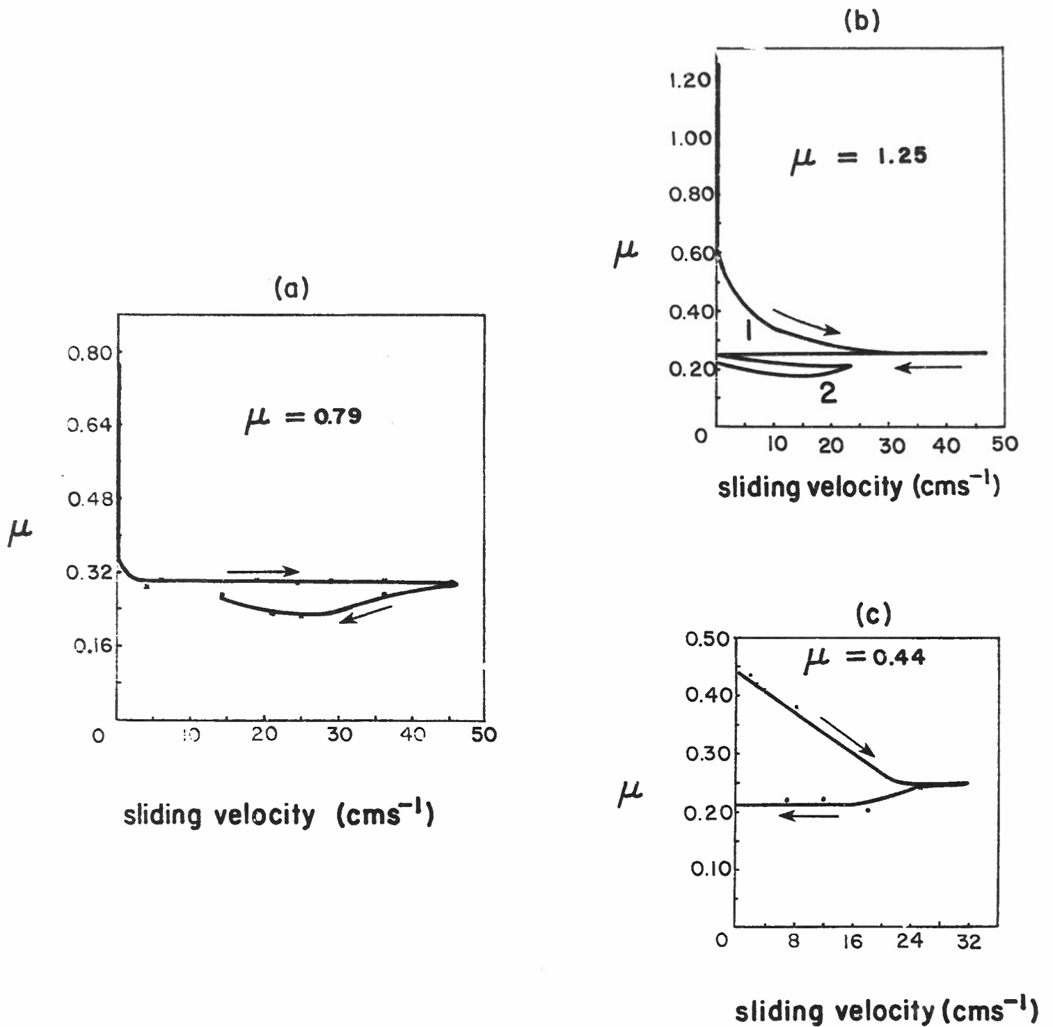
Figure 41. Coefficient of friction vs. sliding velocity.
