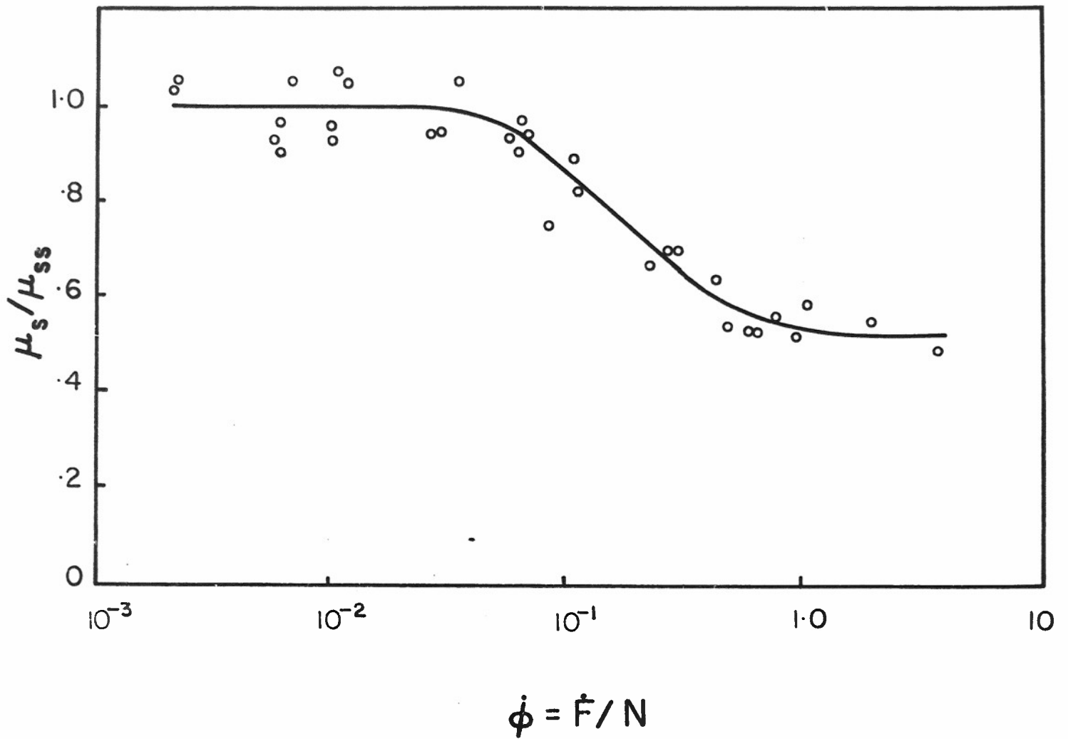
Figure 29. Static friction vs. loading rate. Logarithmic \phi scale and static coefficient of friction normalized by dividing by \mu_{ss} the coefficient of static friction at low loading rates. (RICHARDSON and NOLLE [1976]).
