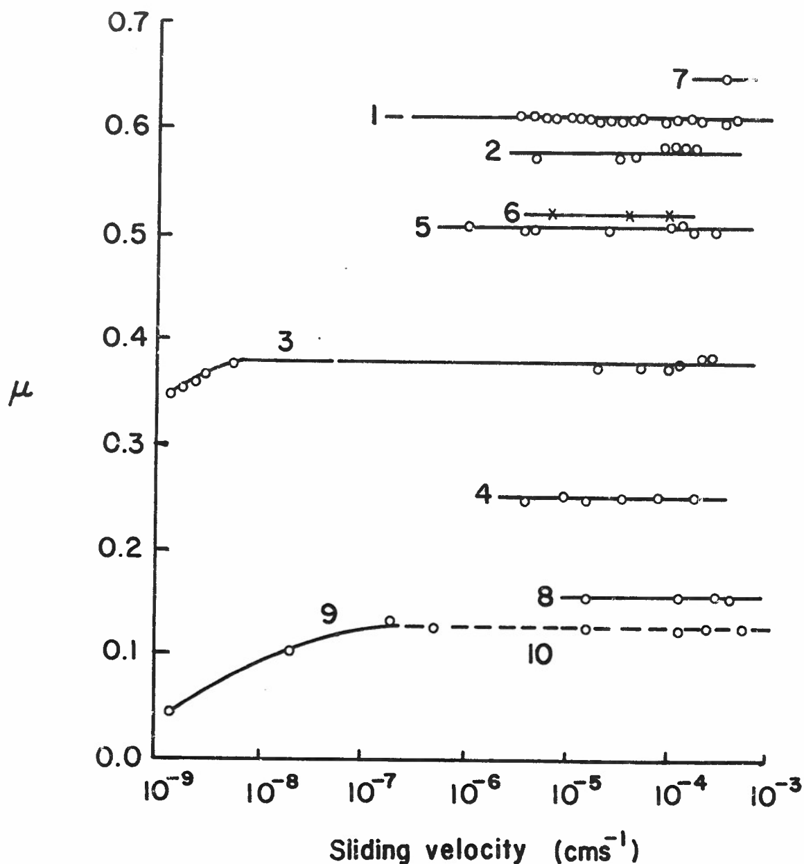
Figure 45. Coefficient of friction as a function of sliding velocity under external normal damping (curves 1-8) or without normal damping (curves 9-10).
