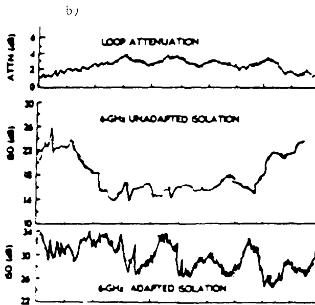
Figure 1-10 Simulated INTELSAT V Dual Frequency Performance in 20mm/hr Rain a) Downlink Results b) Uplink Results
