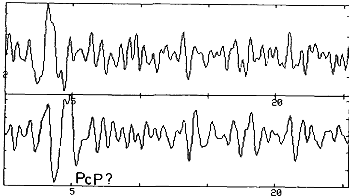
Figure 19. Examples of filtered site terms for the set of Astrakhan data recorded at the RSTN. In each pair, the top trace is the deconvolved site term, which has been filtered in the bottom trace with a von Seggern and Blandford wavelet assuming a yield of 22 kt, t^* = 0.15 sec, and an RSTN instrument response. The predicted location of the PcP arrival is also marked.
