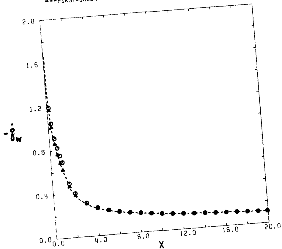
FIG. 29 WALL HEAT-TRANSFER RATE WITH THREE DIFFERENT TYPES OF INITIAL PROFILES. ○ ZERO-ORDER ASYMPTOTIC PROFILES; ▲ EXTENDED WU-TYPE PROFILES; --- FIRST-ORDER ASYMPTOTIC PROFILES.
