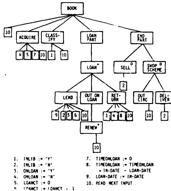
Figure 4-5: Process Tree for Cameron's Book Example
