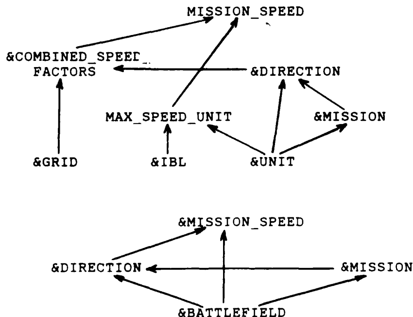
Figure 5-4: Alternative ONEC Genus Graphs
