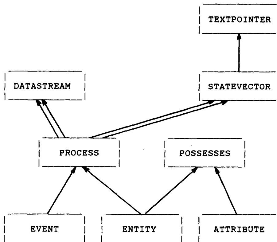
Figure 4-4: SM Generic Structure of JSD Model
