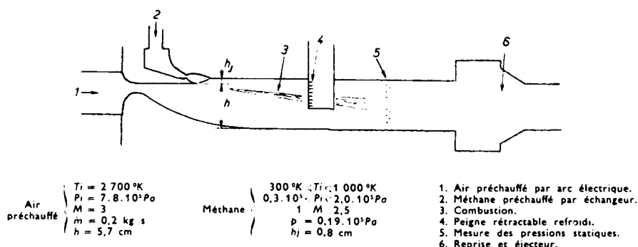
Figure 2. Borghi's arc-preheated combustor.
