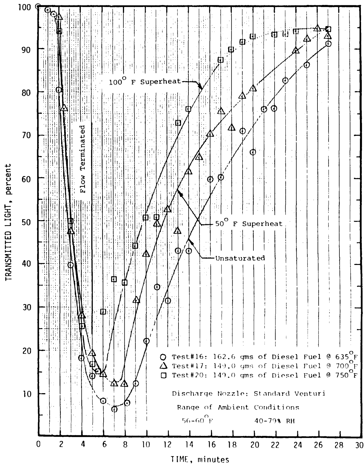
Figure 9. Effect of Superheat on Quality of Moke Produced from Diesel Fuel Discharged from a Venturi Nozzle
