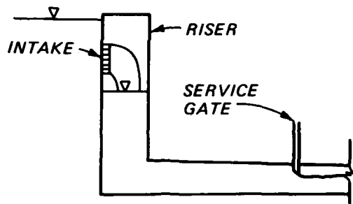
a. DISCHARGE CONTROL AT INTAKE (FREE ORIFICE FLOW-UNDESIRABLE MODE OF OPERATION)
