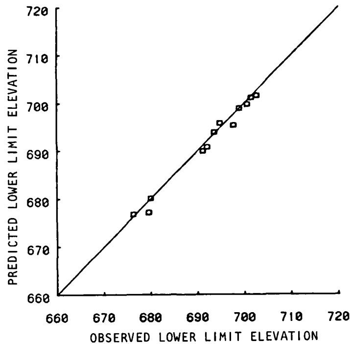
Figure 10. Observed versus predicted lower limit elevation
