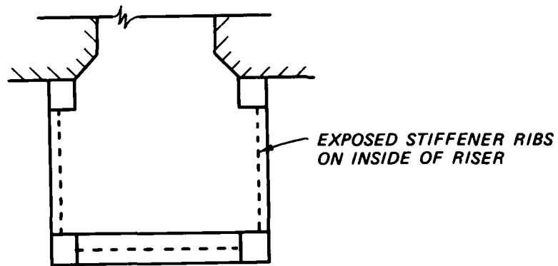
a. Plan view of original design riser
