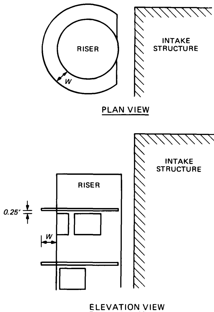
Figure 7. Vortex suppression aprons
