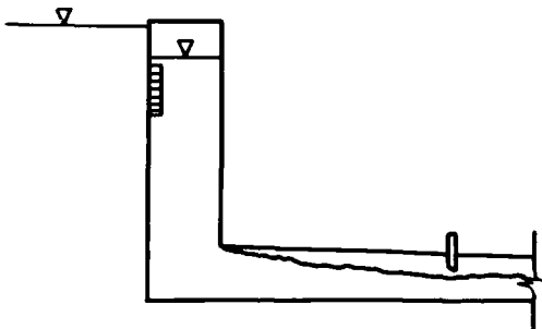
c. DISCHARGE CONTROL IN PASSAGEWAY (SUBMERGED ORIFICE FLOW-UNDESIRABLE MODE OF OPERATION)
