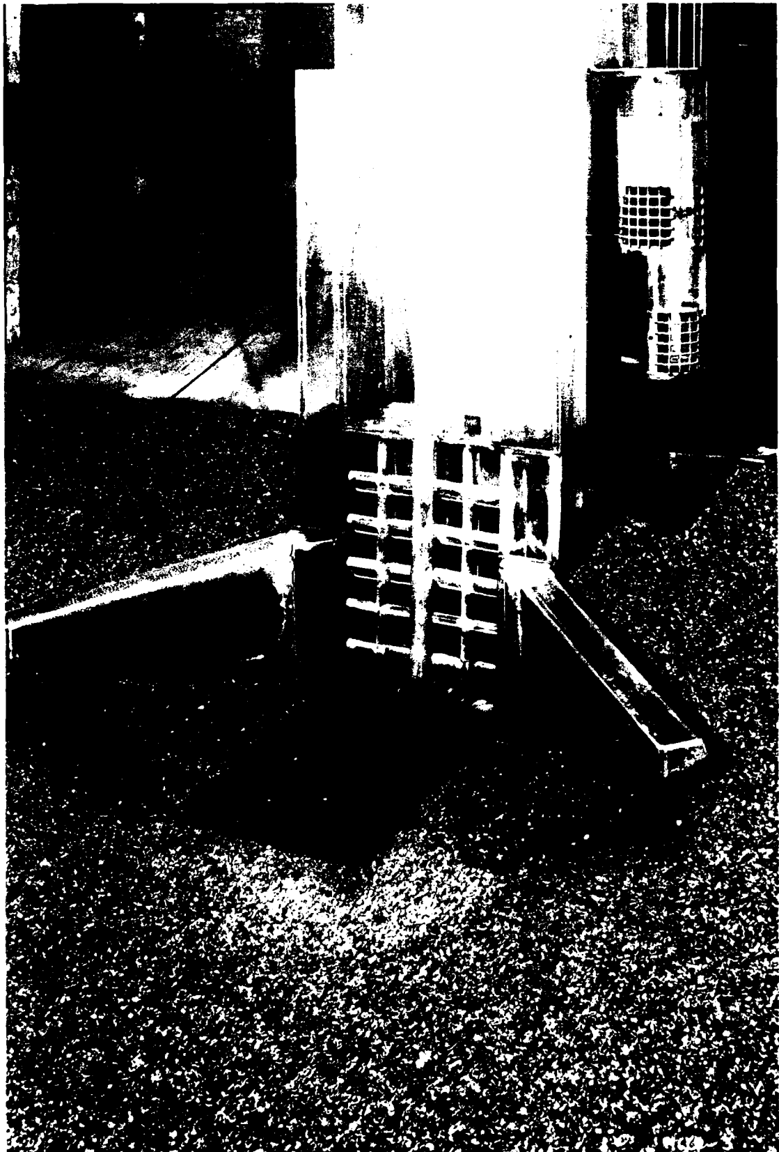
Figure 2. Intake structure with proposed selective withdrawal riser, 1:18-scale hydraulic model
