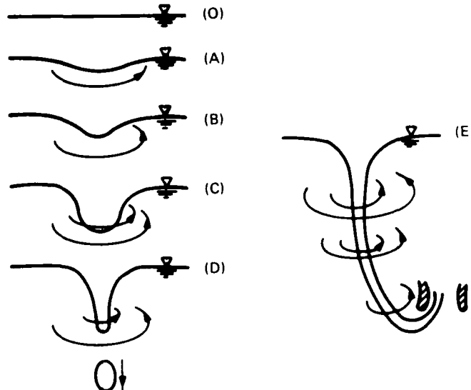
Figure 6. Stages in development of air-entraining vortices
