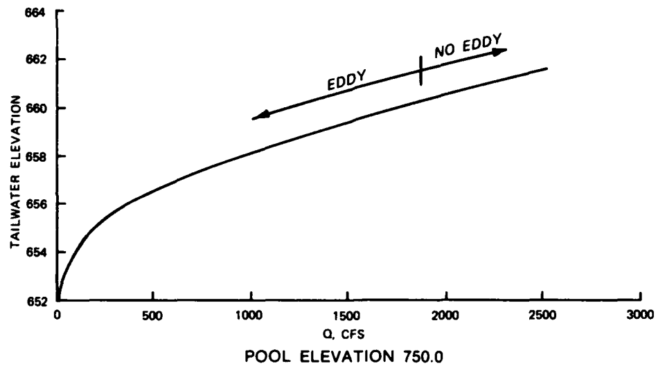
STILLING BASIN PERFORMANCE EQUAL SERVICE GATE OPENING TAILWATER CURVE BASED ON JULY 1971 STUDY
