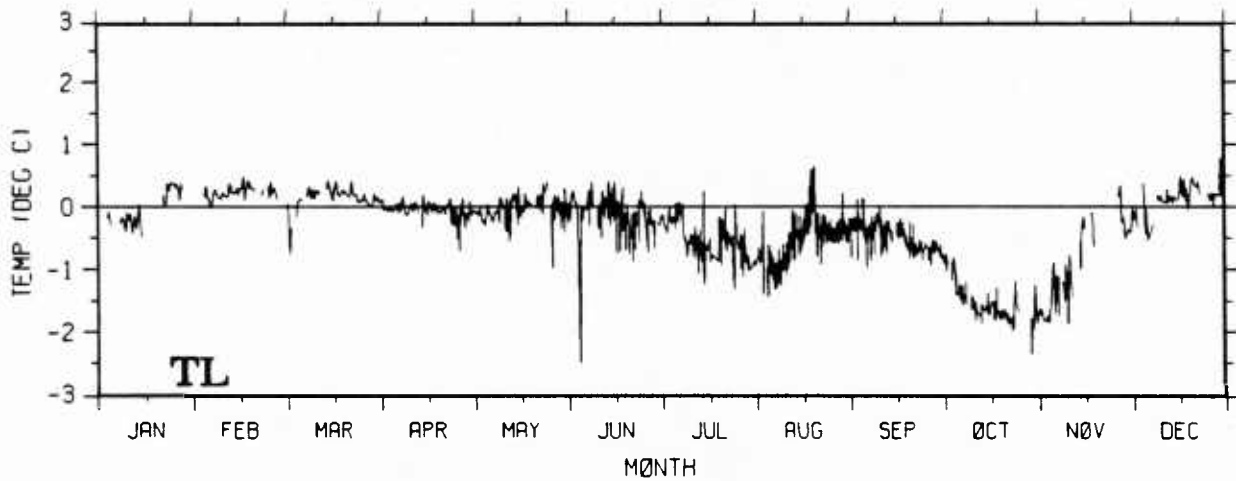
Figure 6b. Difference between predicted and observed SST at Papa with the Garwood, Price, and TL models.
