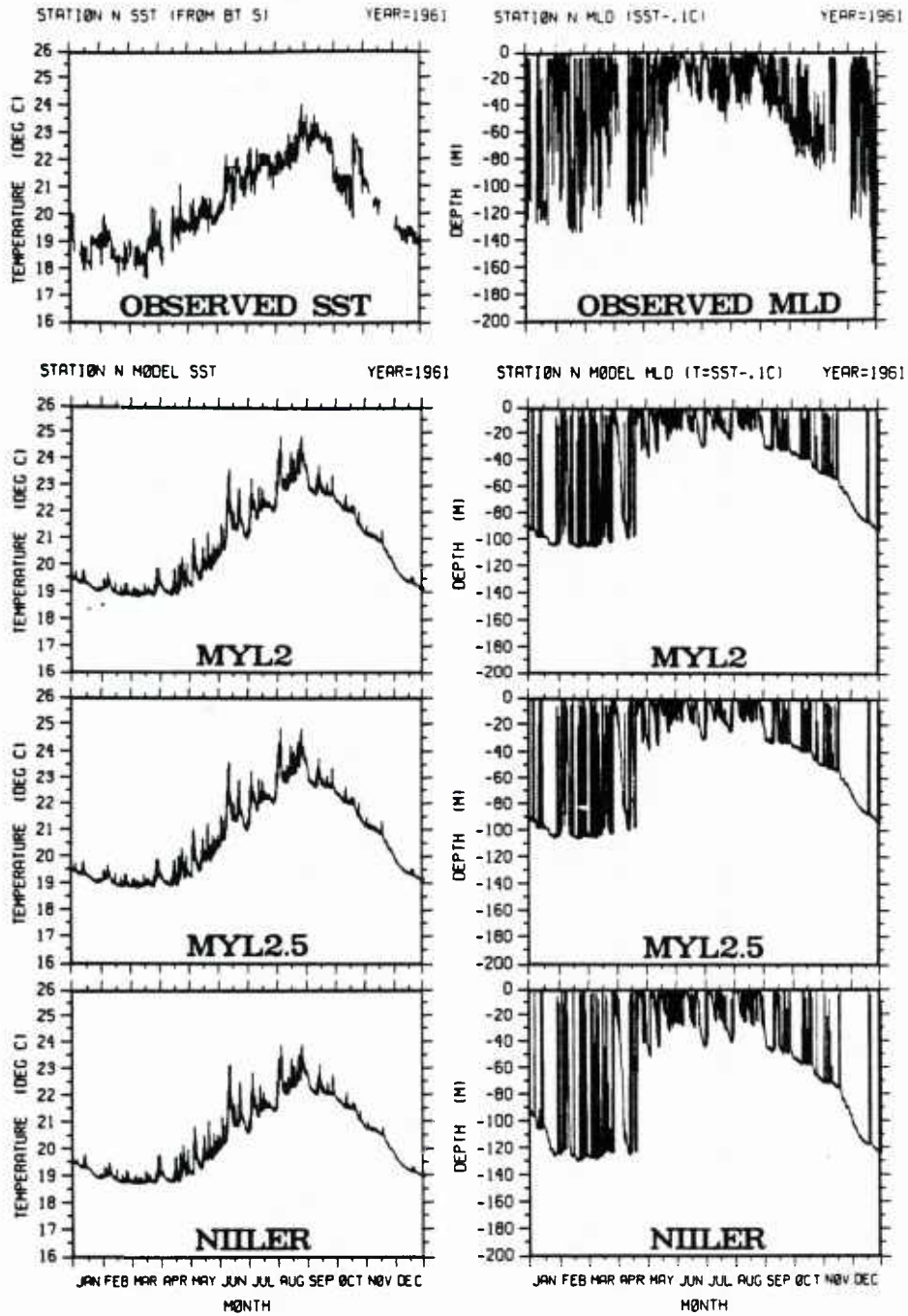
Figure 2a. Observed and predicted SST and MLD at Ocean Station November for the year 1961. Predicted results are for the MYL2, MYL2.5, and Niiler models.
