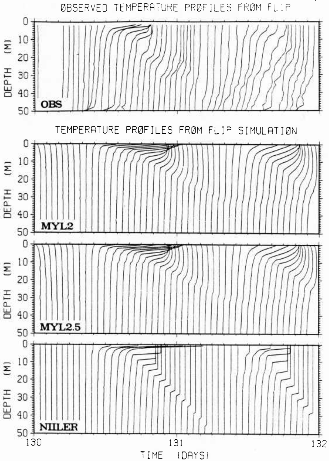
Figure 10a. Observed and predicted temperature profiles for simulation of the data from R/P FLIP for May 9-10, 1980. Predicted profiles are for the MYL2, MYL2.5, and Niler models. The horizontal scale is 1 day = 1.43°C.
