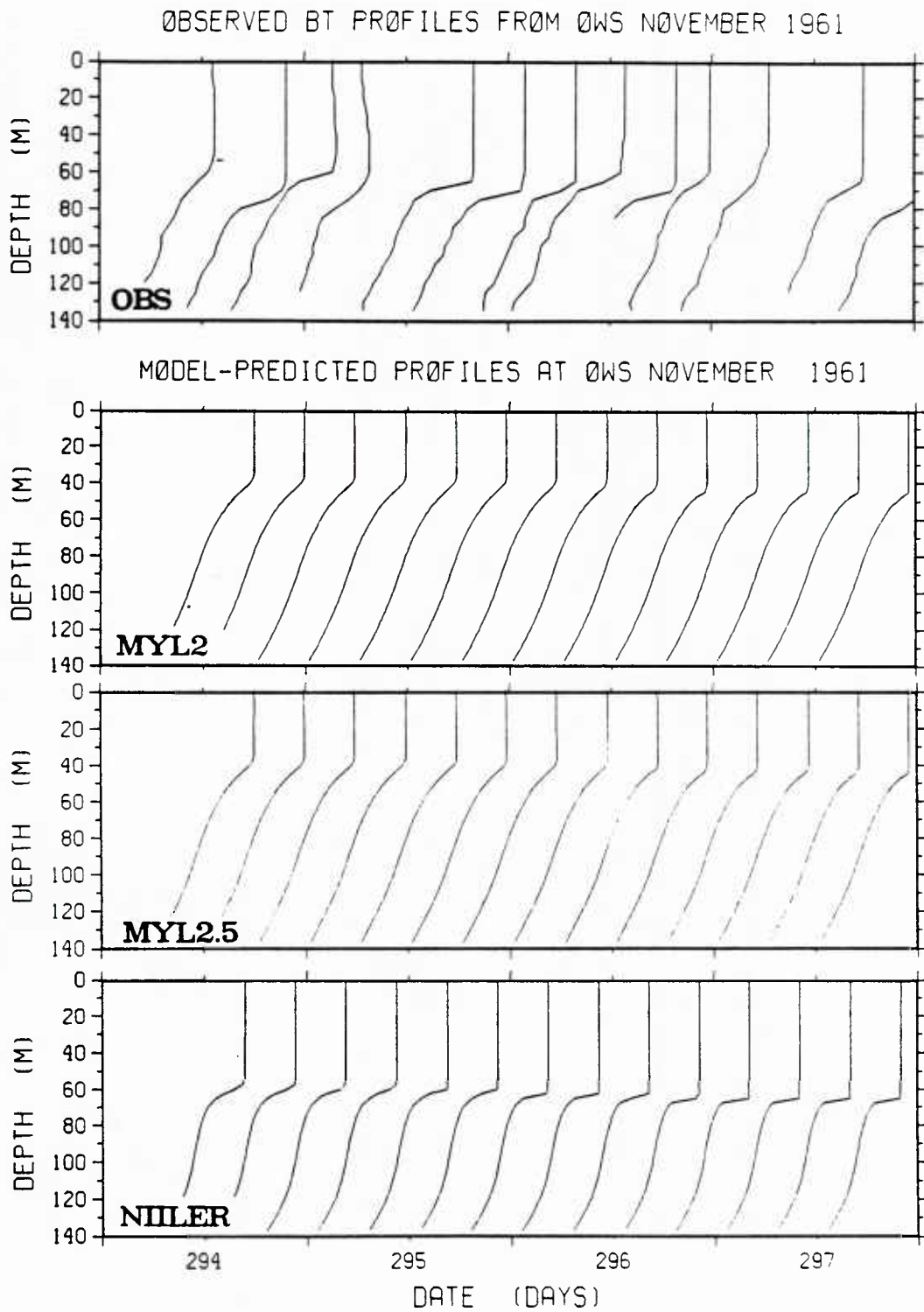
Figure 4a. Observed and predicted profiles at November for a 4-day period near the end of October (October 21-24). Predicted profiles are for the MYL2, MYL2.5, and Niiler models. The horizontal scale is 1 day = 10°C.
