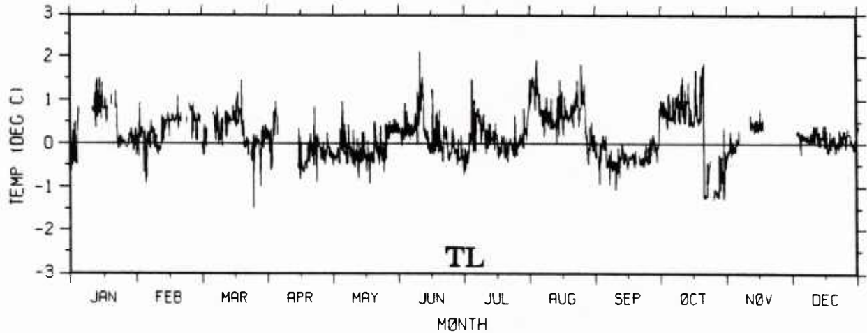
Figure 3b. Difference between predicted and observed SST at November with the Garwood, Price, and TL models.
