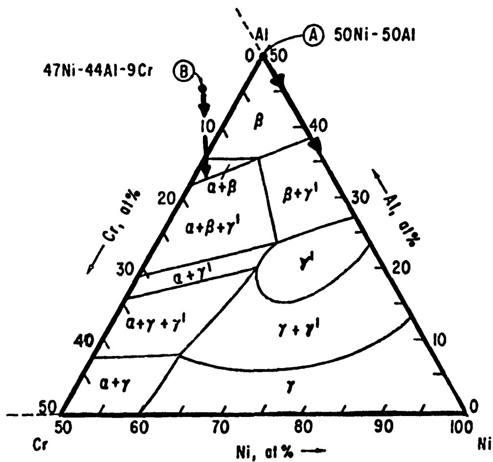
FIG. 7: NICKEL RICH CORNER OF THE Ni-Al-Cr PHASE DIAGRAM AT 1123 K, AND THE IDEALIZED DEGRADATION PATHS FOR a) NiAl (50:50) and b) NiAl + 10 a/o Cr (REF. 83)
