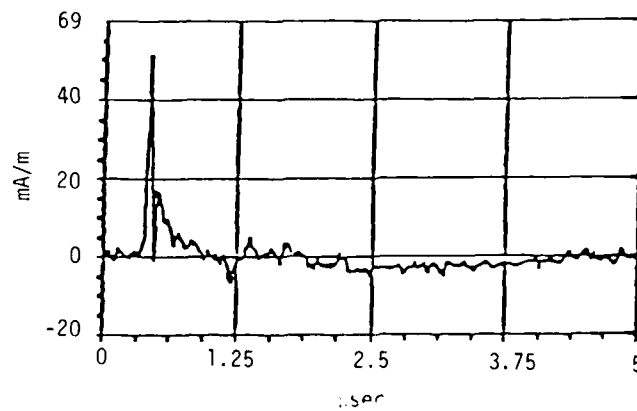
Fig. 7 - Measured electric field for vertically polarized illumination ( E_{\text{inc}} = 123 \text{ kV/m} ).
