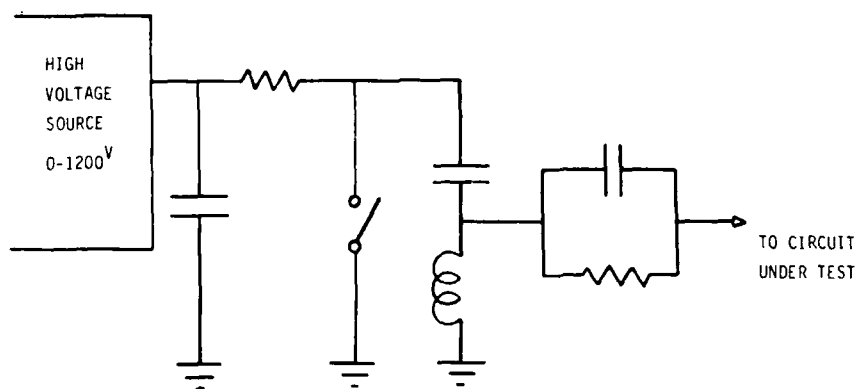
Figure 3. Transient generator circuit.
