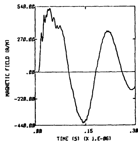
Figure 4. Lateral magnetic field near top of tail boom, NEMP excitation - vertical incidence, longitudinal polarization.
