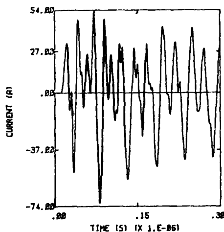
Figure 5. Short circuit current on longitudinal wire, NEMP excitation - vertical incidence, longitudinal polarization.
