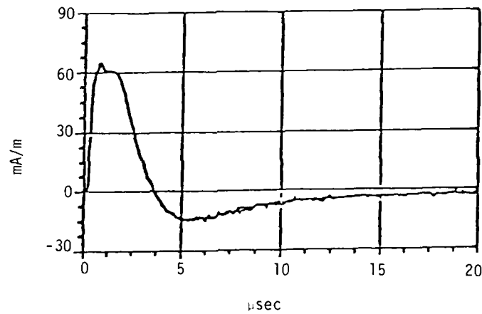
Fig. 6 - Measured internal magnetic field for vertically polarized illumination ( E_{\text{inc}} = 123 \text{ kV/m} ).
