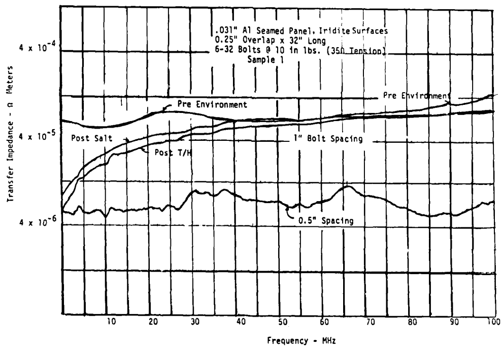
Fig. 2 - Seam impedance for typical bolted seams, showing environment effects (5) T/H - temperature/humidity test.
