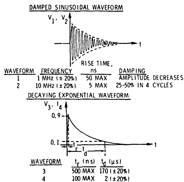
Figure 2. SAE waveforms recommended for lightning-induced testing.
