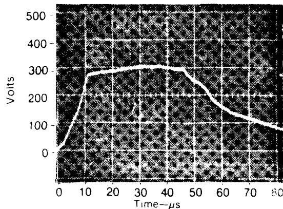
FIGURE 7 Magnified View Of Protector Output
