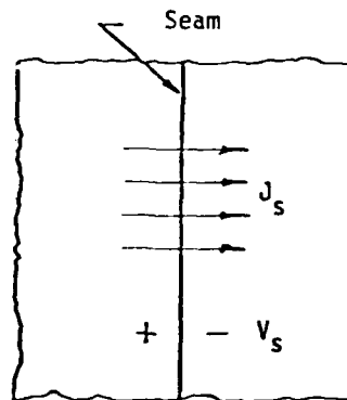
Fig. 1 - Surface current density flowing across a seam.
