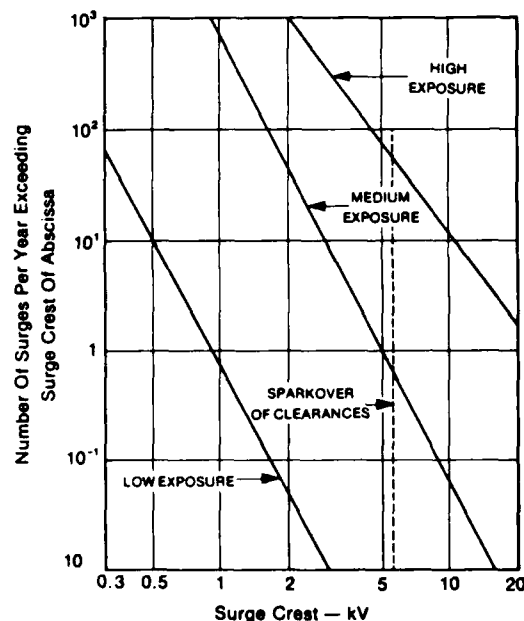
FIGURE 3 Rate Of Surge Occurrences At Unprotected Locations
