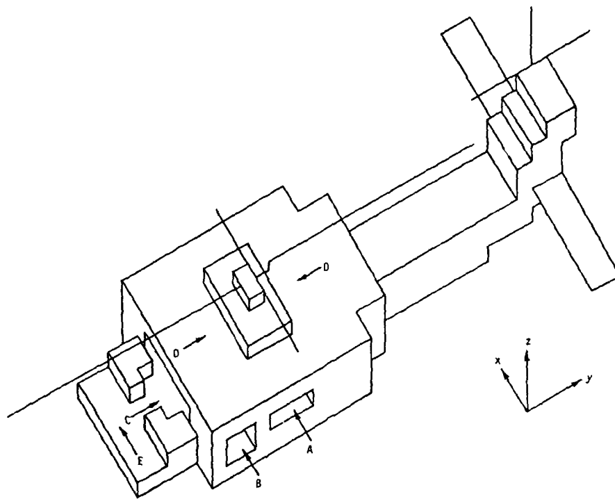
Figure 1. Three-dimensional finite-difference model of UH-60A helicopter.
