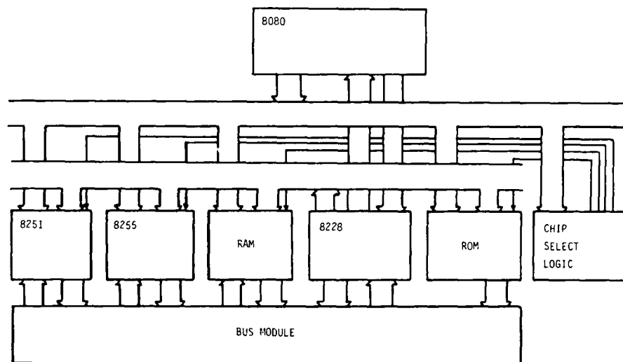
Figure 8. System under test.
