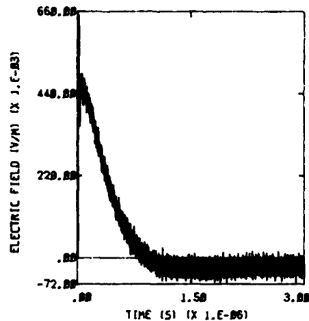
Fig. 9 - Calculated value of E_y .
