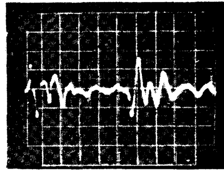
FIGURE 9—Protector Output With EMP Input (6kV, 120A) 20V Div., 50μs Div.
