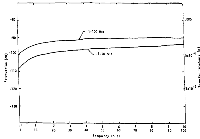
Fig. 5 - The (experimental) values of attenuation and surface transfer impedance Z_{\text{meas}} for metallic honeycomb (1/8" x 1/2" steel, 10" x 10" frame, Tecknit #64-90055; steel shield plate) (5, 11).
