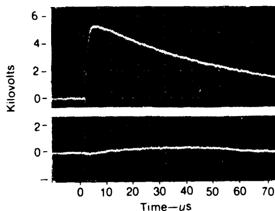
FIGURE 6—Transient Reduction
