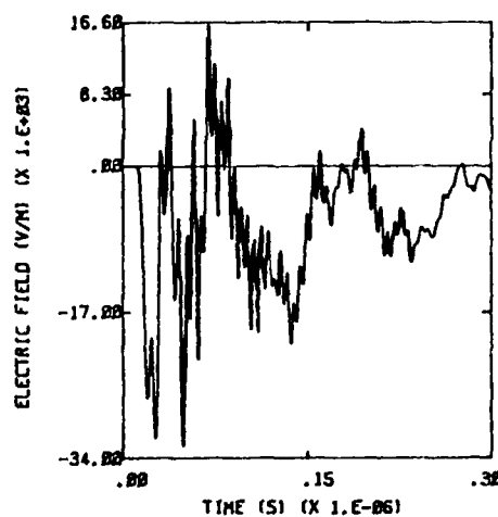
Figure 3. Normal electric field at test point 1, NEMP excitation - vertical incidence, longitudinal polarization.
