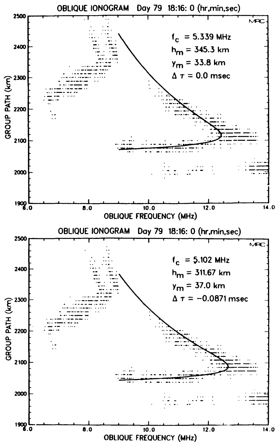
Figure 13. Comparison of ionogram fits for no delay shift \Delta\tau = 0 (a) and \Delta\tau fitted (b).
