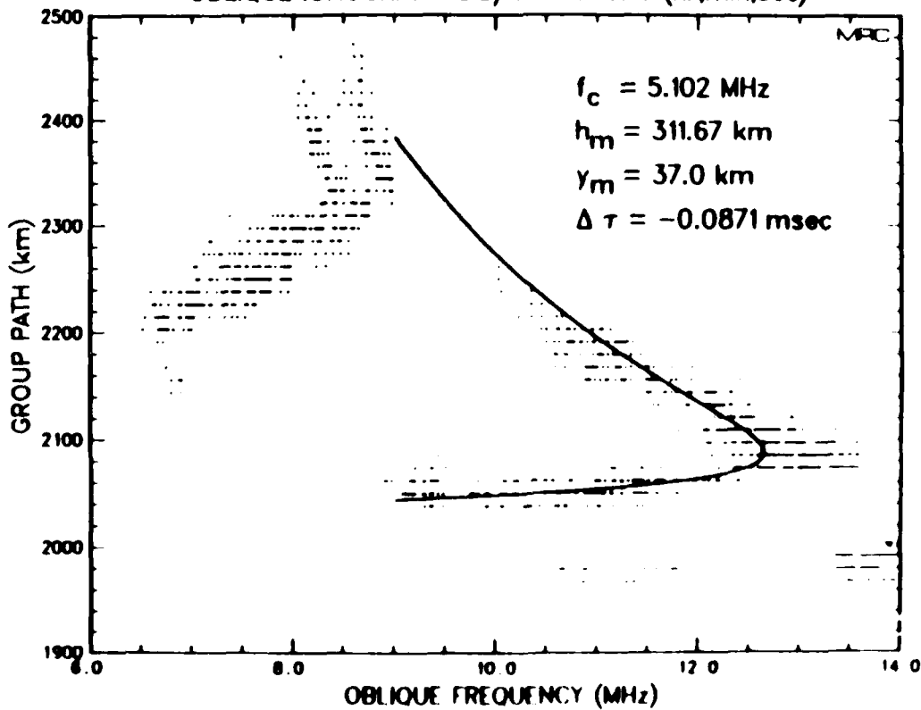
Figure 34. HF Channel Probe scattering function measurement, May 1995, 12:19 GMT, and a corresponding oblique ionogram including best fit parameters for a two-layer model.
