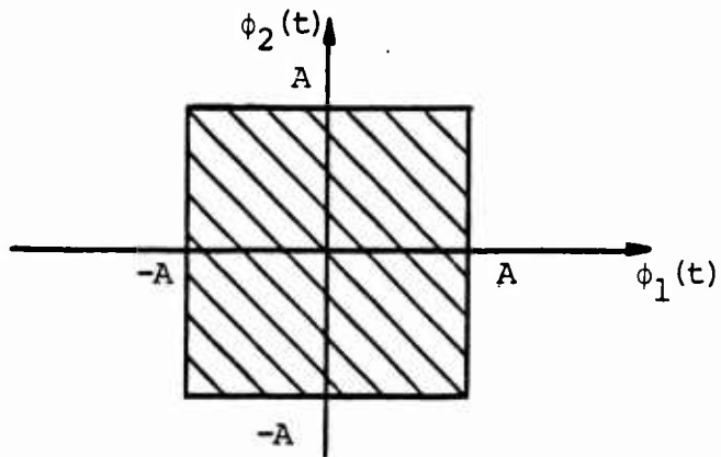
(b) Translated Type II Decision Region
