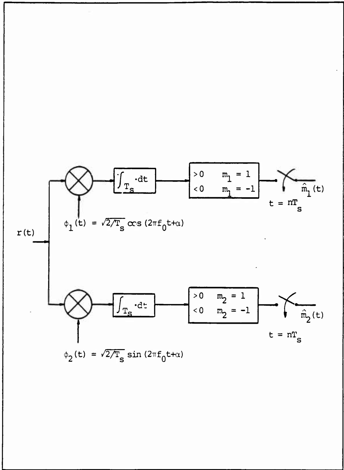
Figure 3.1 Optimum QPSK Receiver Structure
