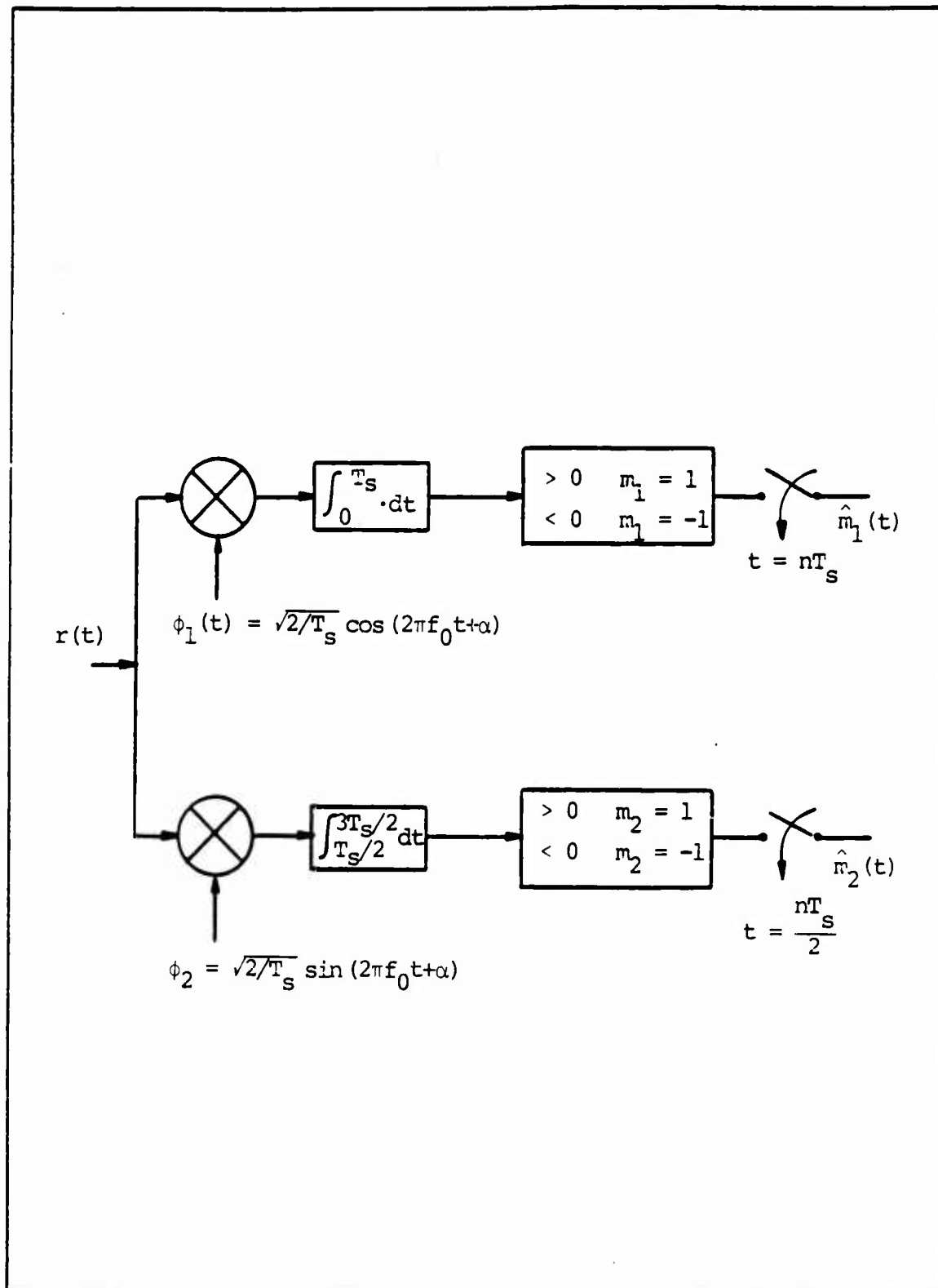
Figure 3.4 Optimum Offset QPSK Receiver Structure
