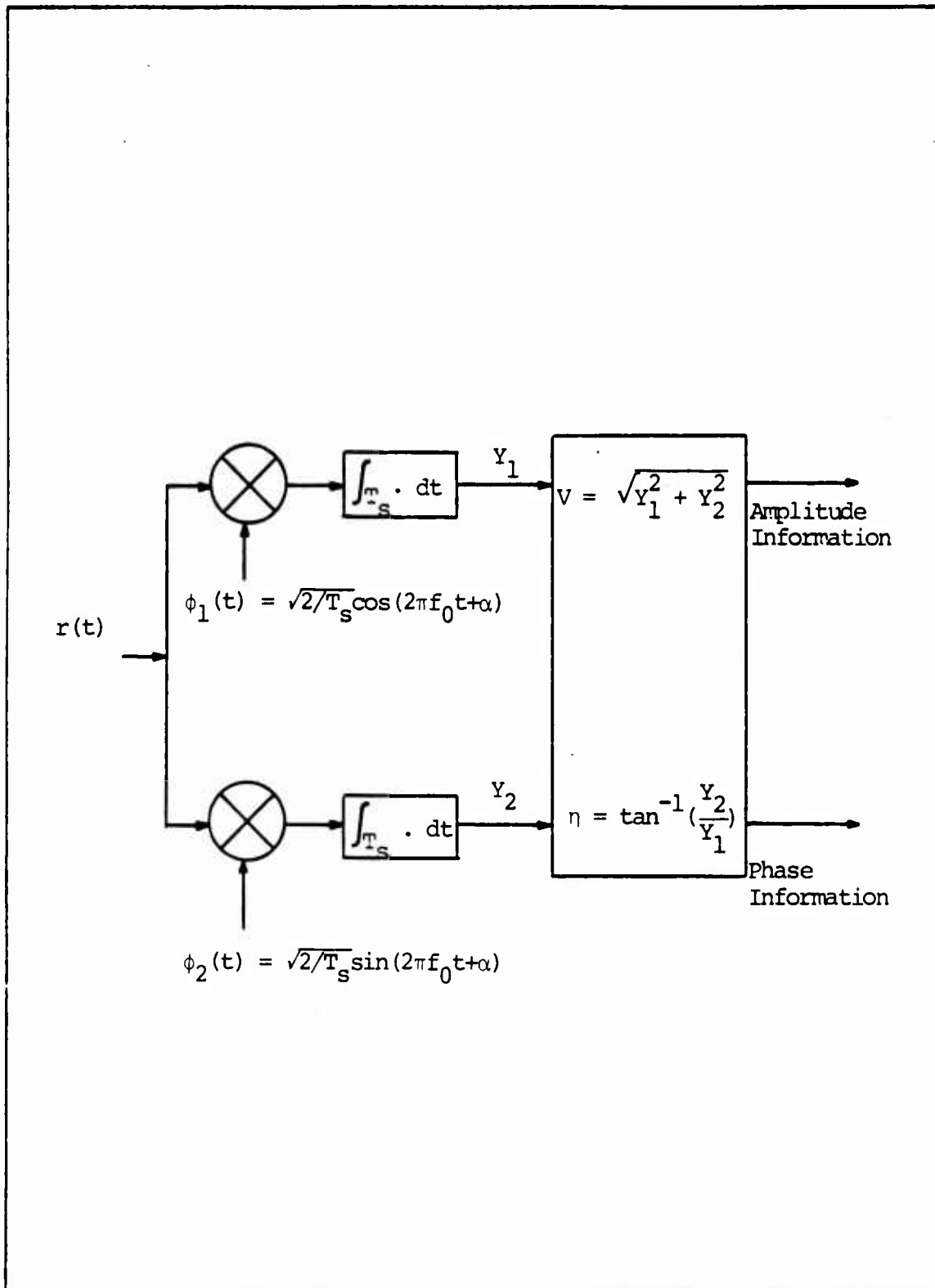
Figure 6.4 Receiver Structure for Suboptimum 16-State AM/PM Signaling
