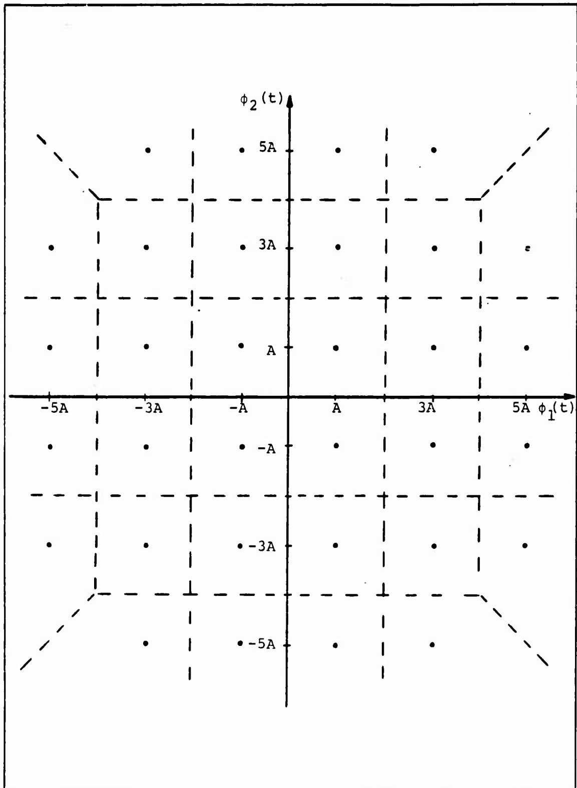
Figure 5.8 Signal Space Diagram for 32 QAM Signaling
