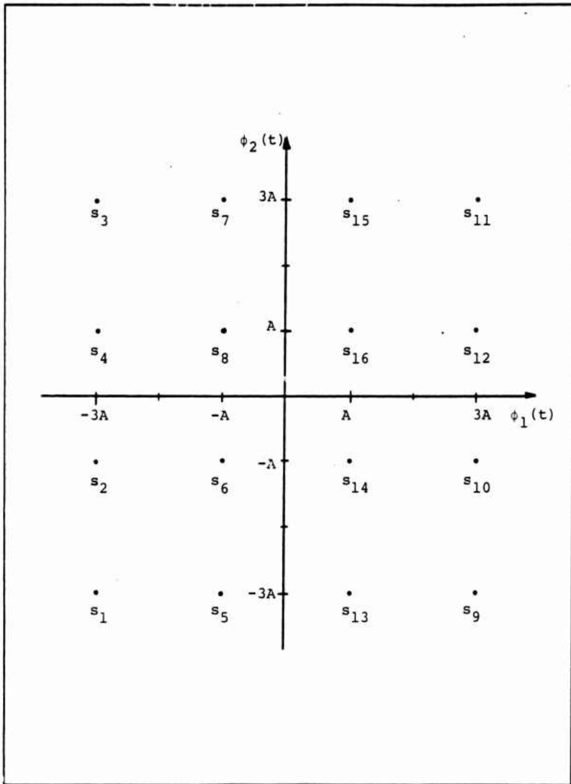
Figure 5.1 Signal Space Diagram for 16 QAM Signaling
