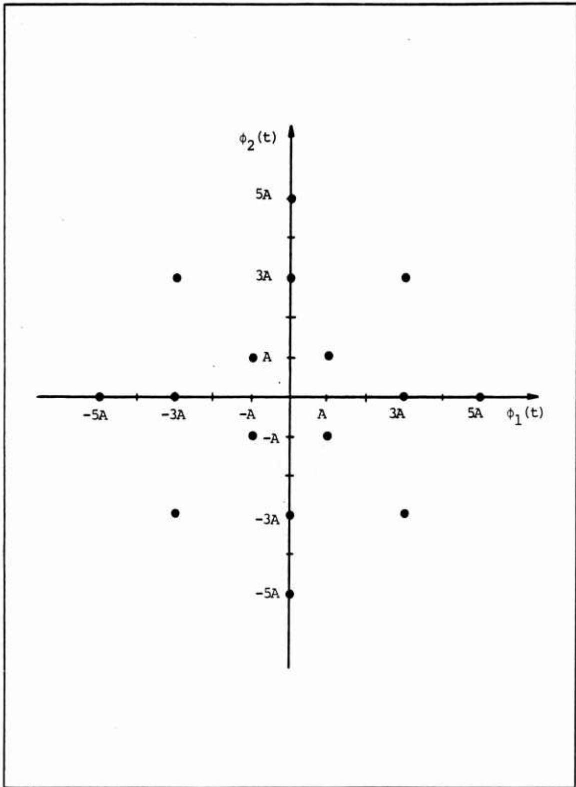
Figure 6.1 Signal Space Diagram for 16-State AM/PM Signaling
