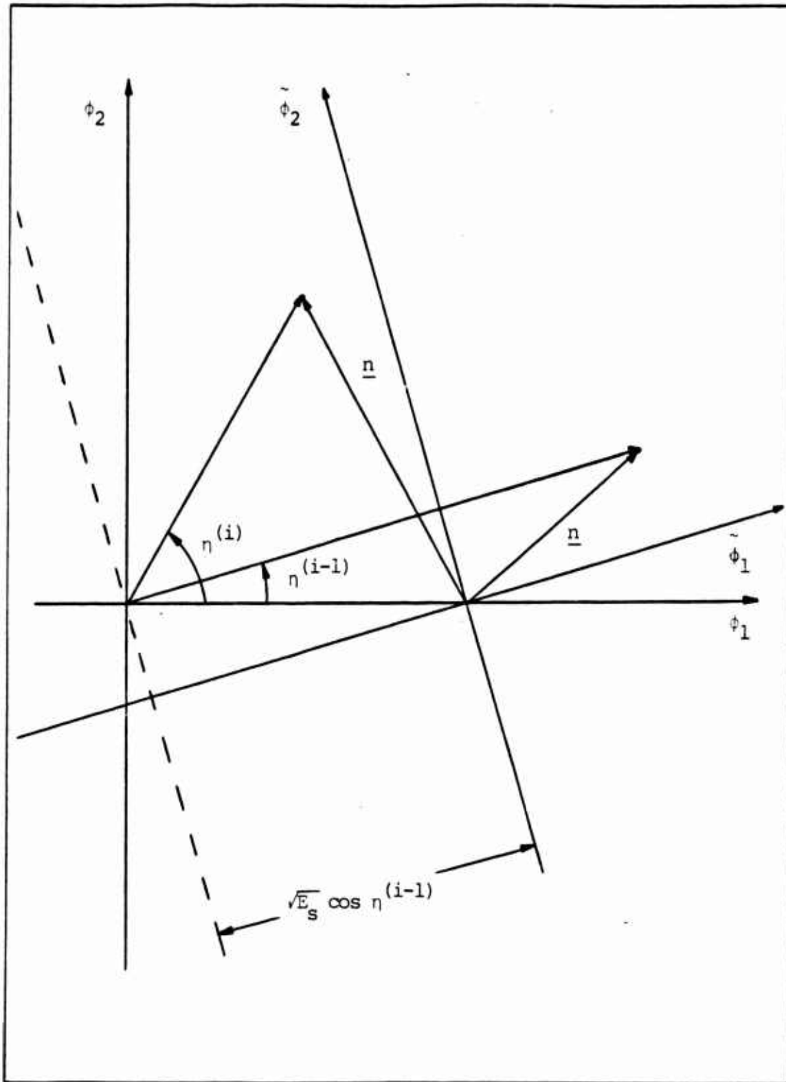
Figure 4.2 Signal Space Representation of Received DPSK Signals
