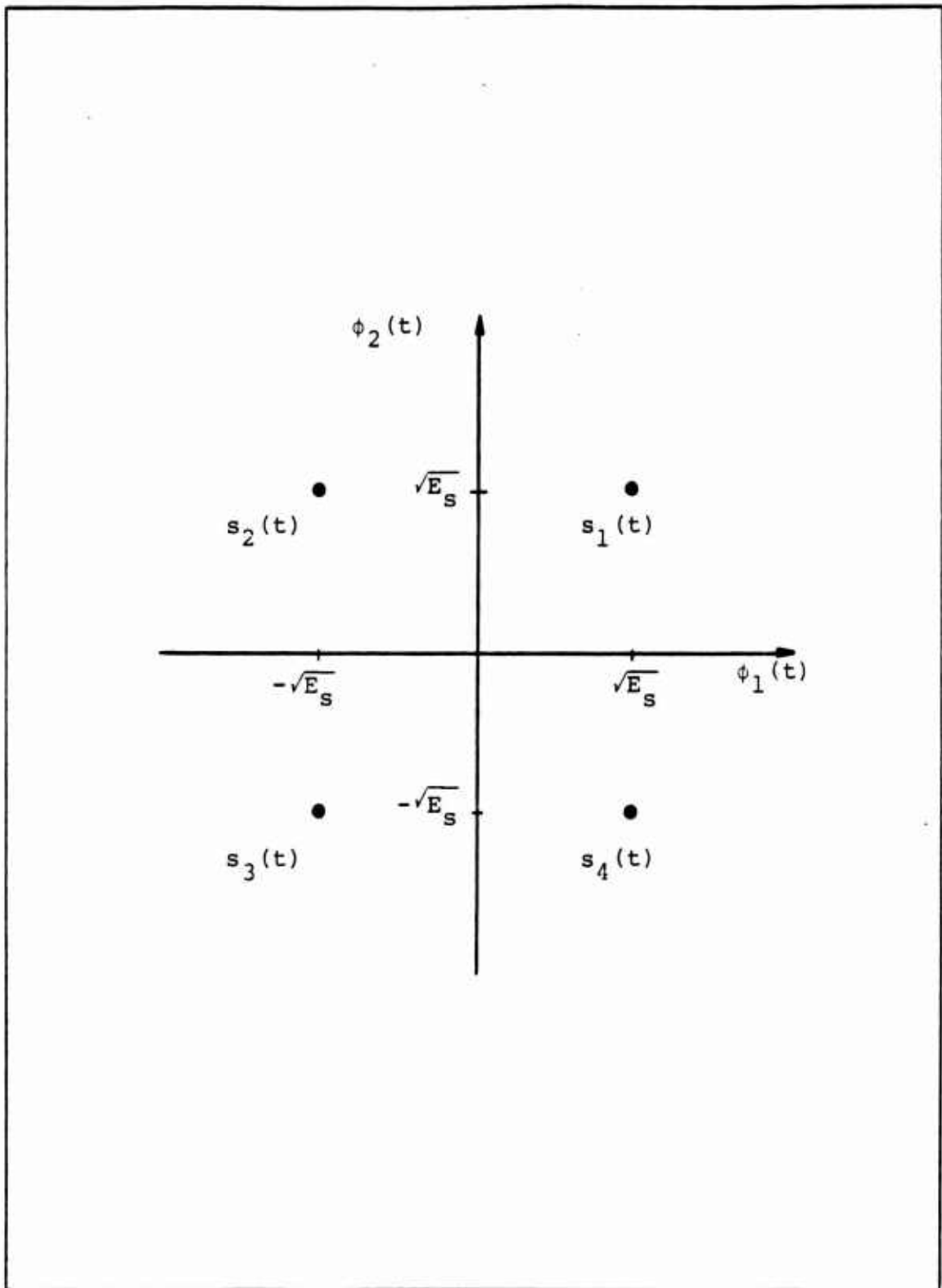
Figure 3.2 Signal Space Diagram for QPSK Signaling
