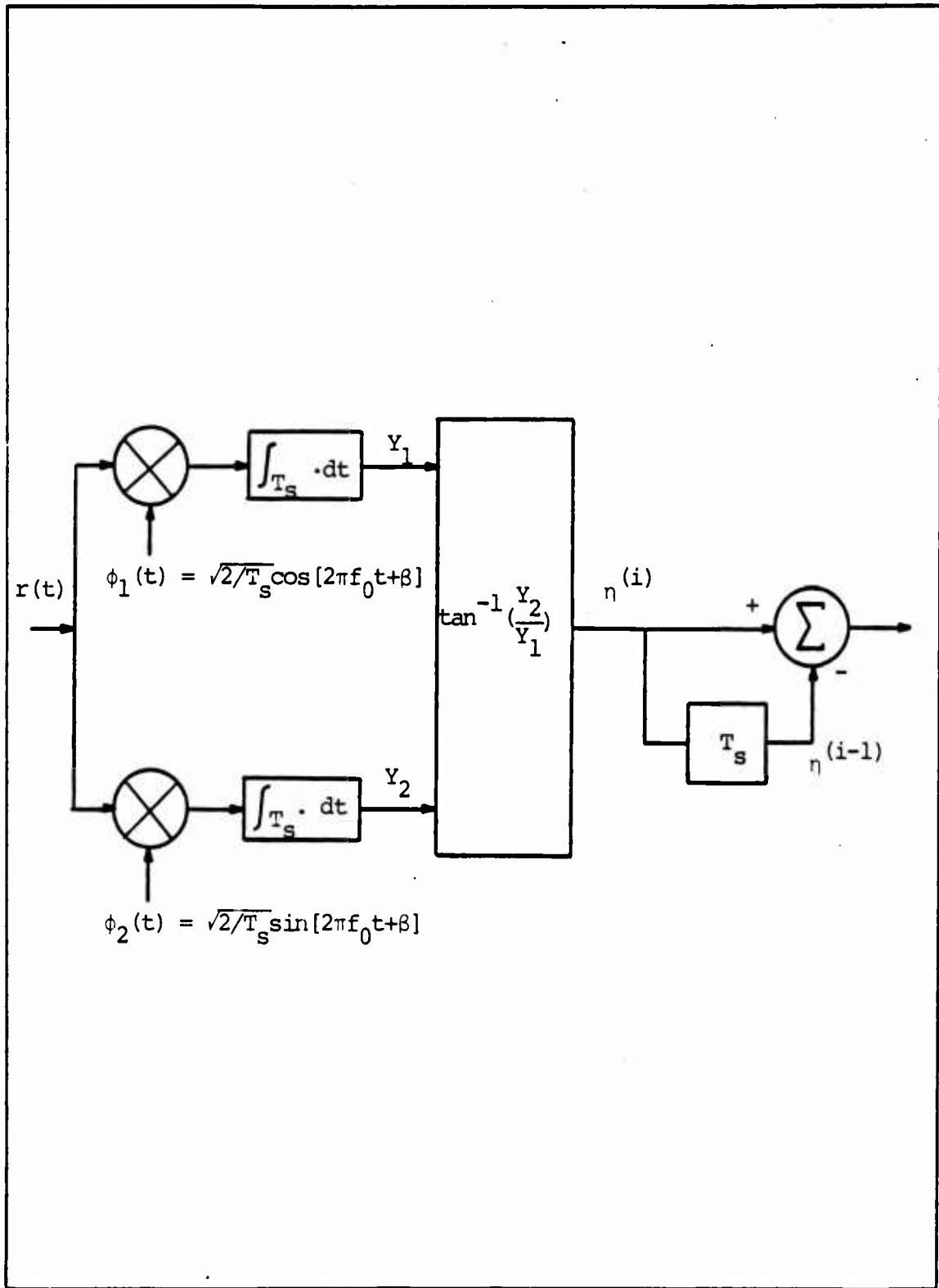
Figure 4.1 Optimum DPSK Receiver Structure
