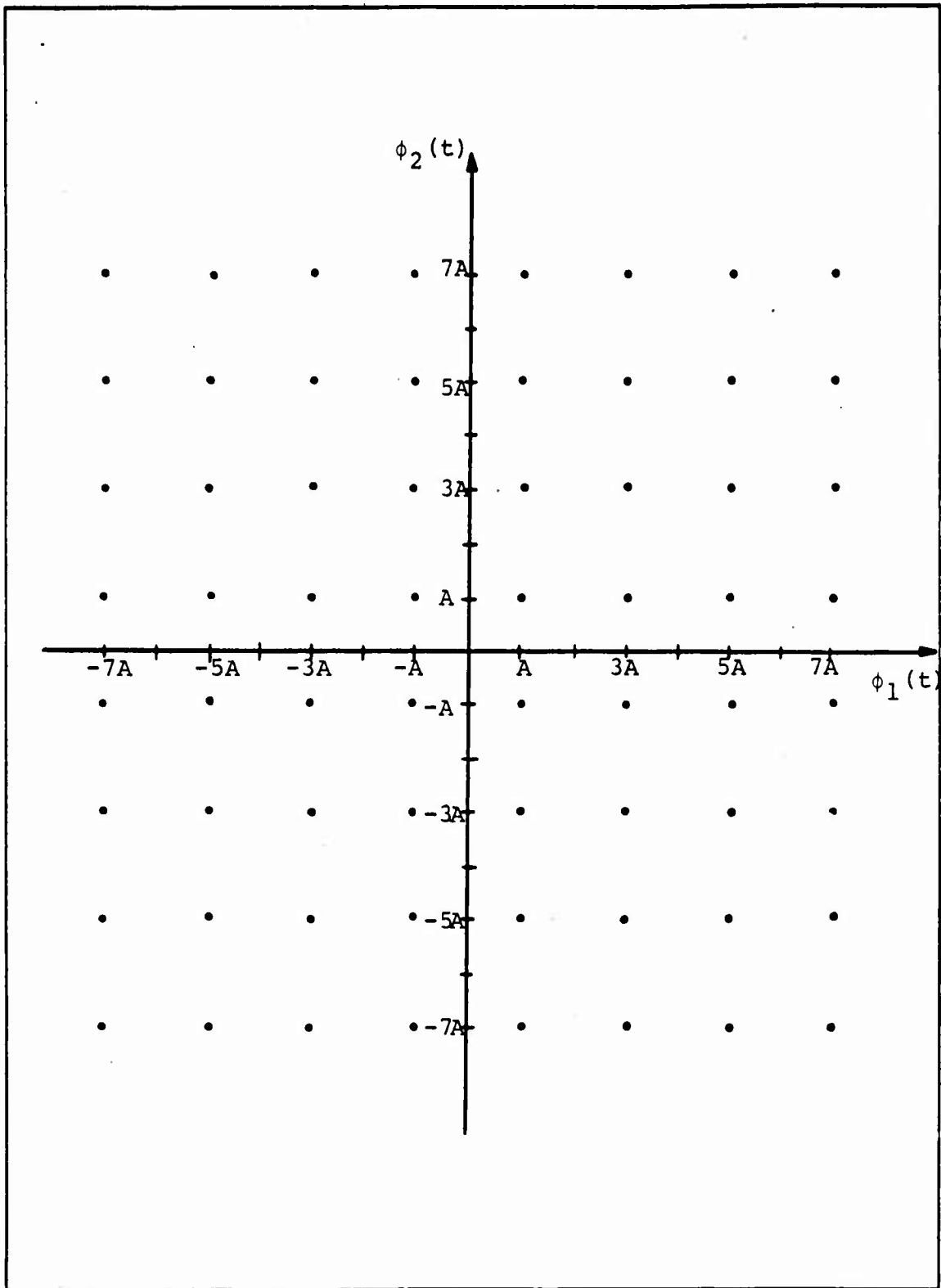
Figure 5.5 Signal Space Diagram for 64 QAM Signaling
