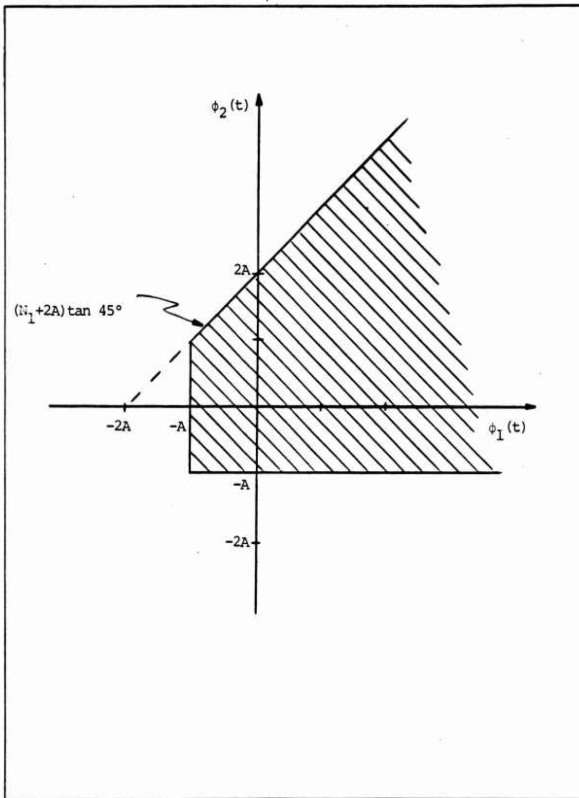
Figure 5.9 Translated Type I Decision Region for 32 QAM
