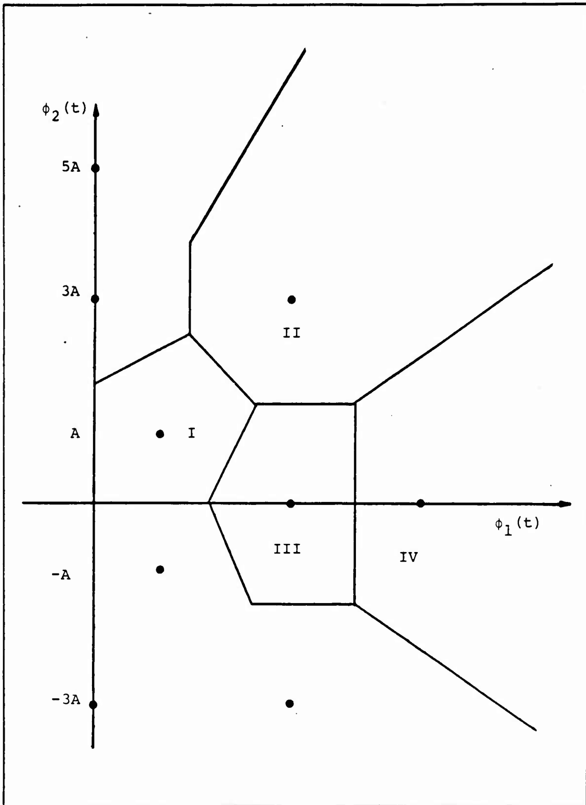
Figure 6.2 Optimum Decision Regions for 16-State AM/PM Signaling
