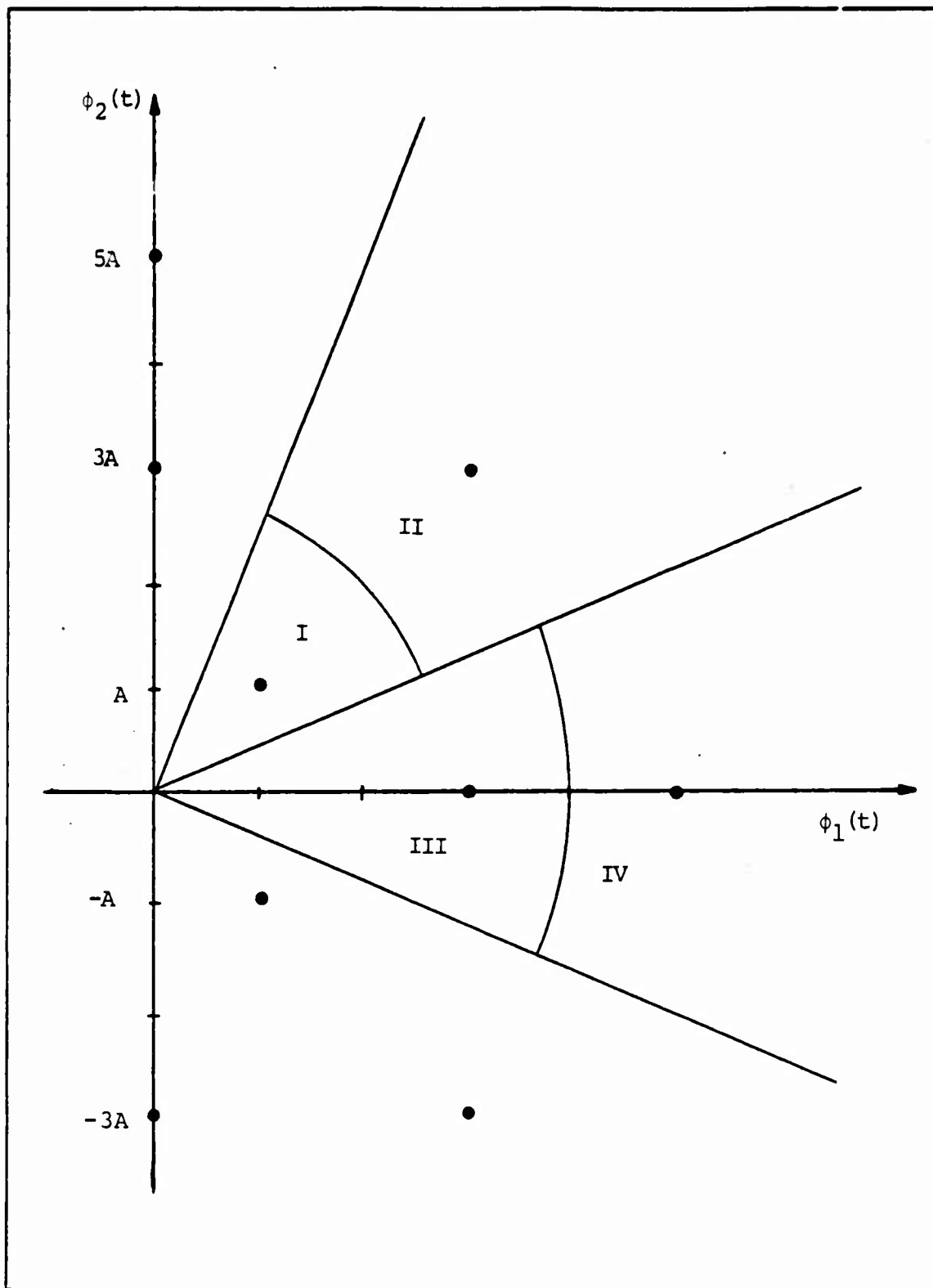
Figure 6.3 Suboptimum Decision Regions for 16-State AM/PM Signaling
