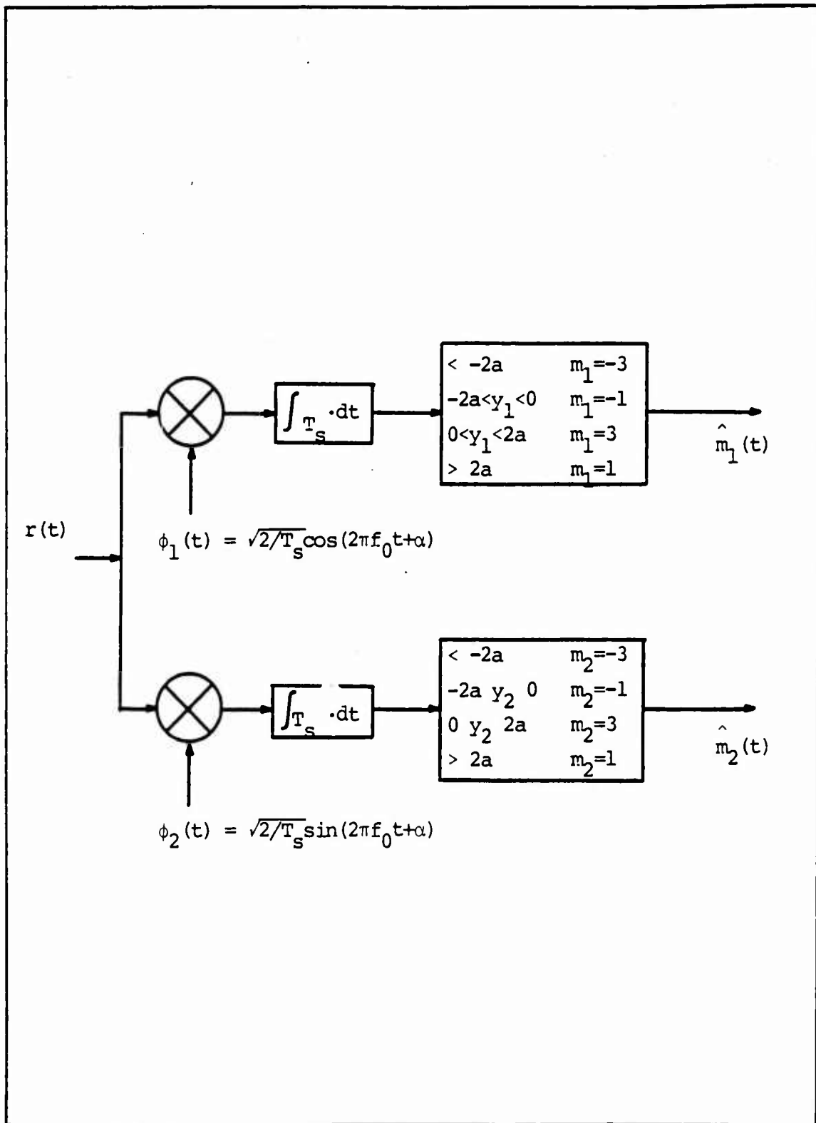
Figure 5.2 Optimum 16 QAM Receiver Structure
