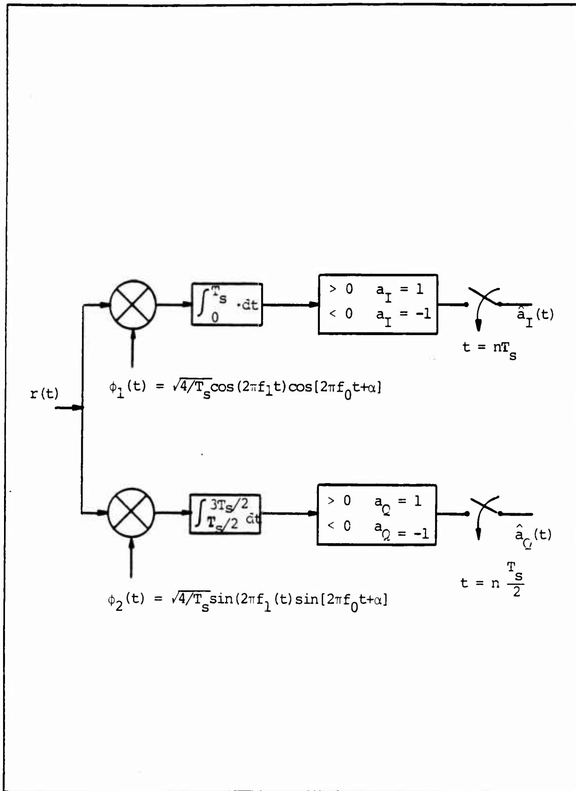
Figure 3.5 Optimum MSK Receiver Structure
