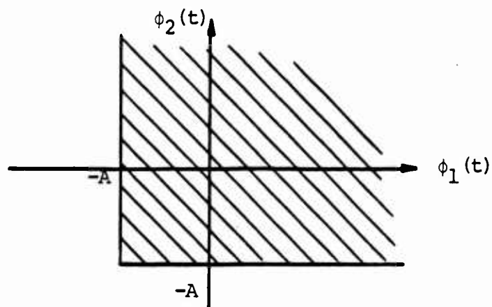
(a) Translated Type I Decision Region
