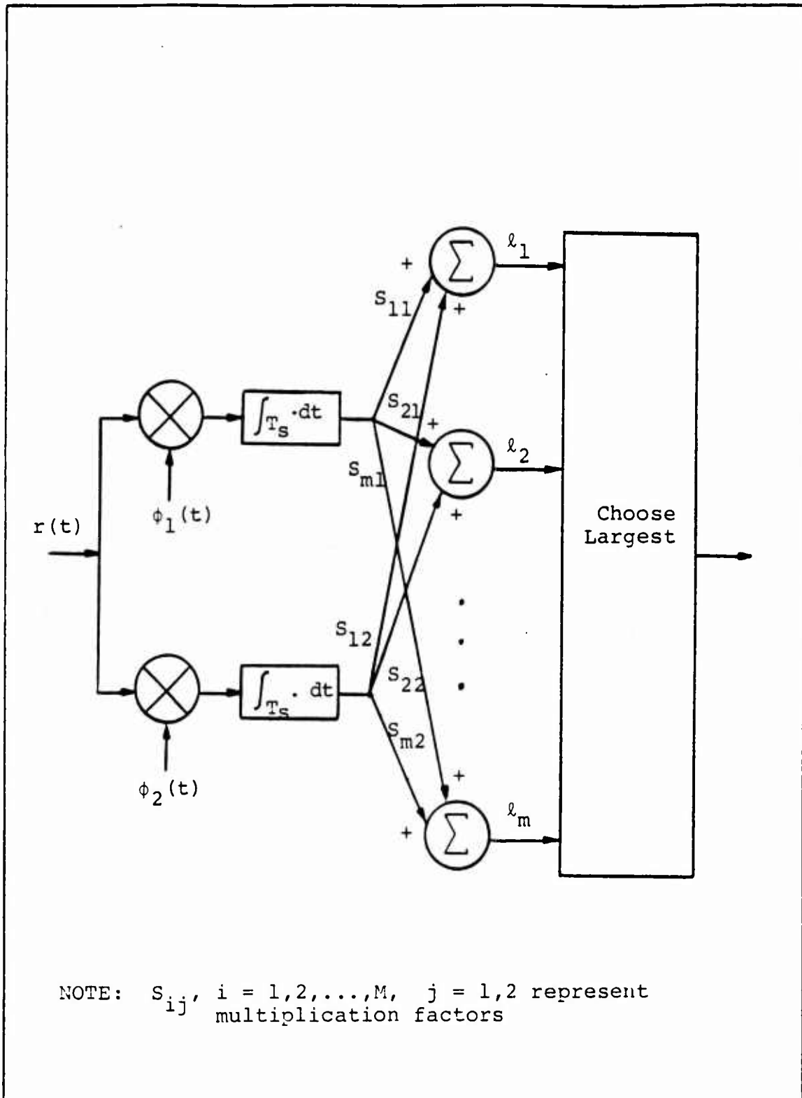
Figure 2.1 Optimum MPSK Receiver for AWGN Channel
