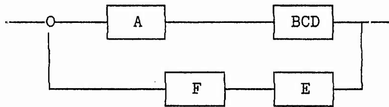
Figure 3-11b. Reduced BCD Loop
