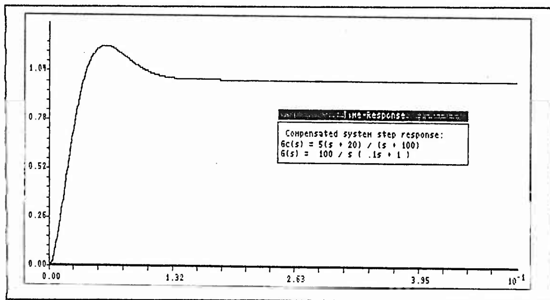
Figure 2-20. Compensated System Time Response
