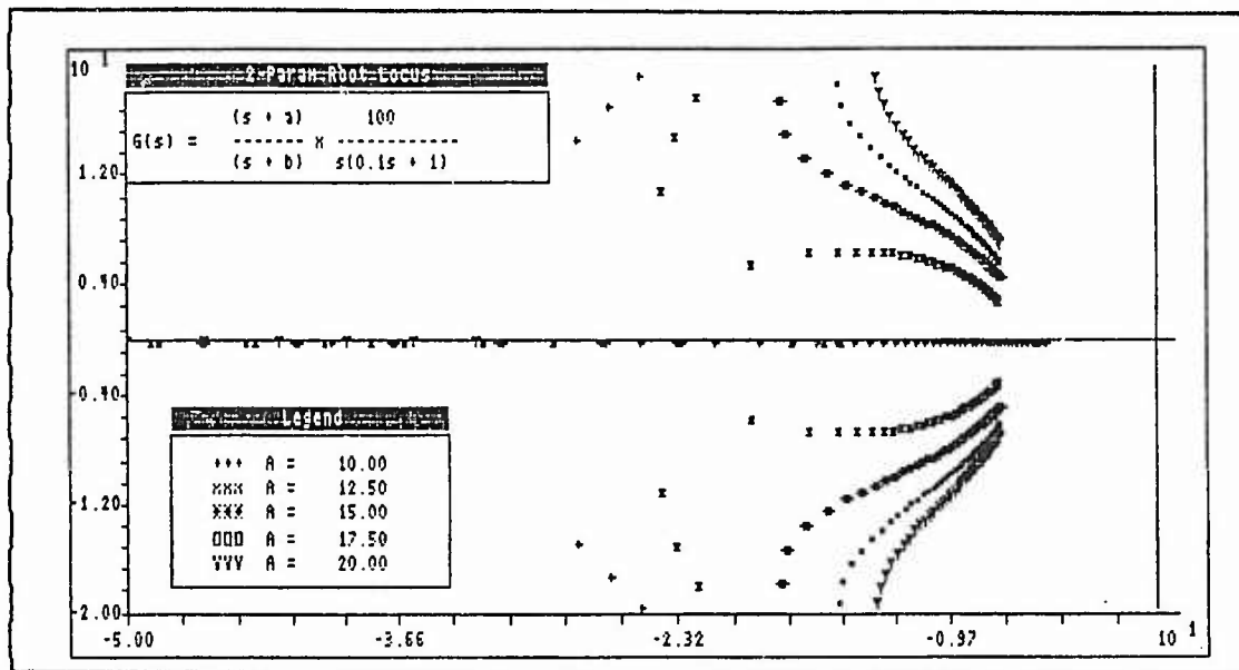
Figure 3-22. Two-parameter Root Locus Family of Curves
