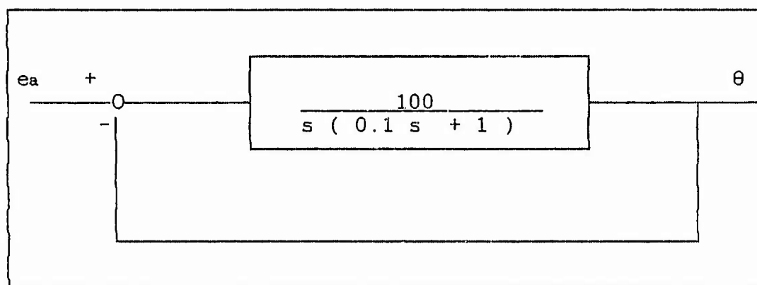
Figure 2-2. DC Motor Equivalent Block Diagram
