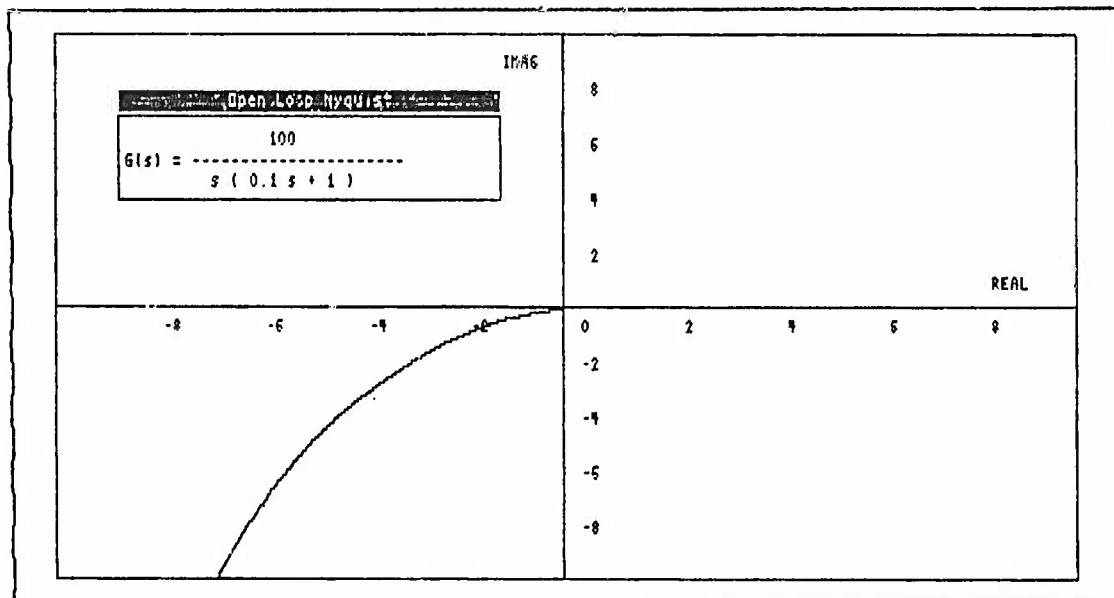
Figure 2-11. DC Motor Nyquist Plot
