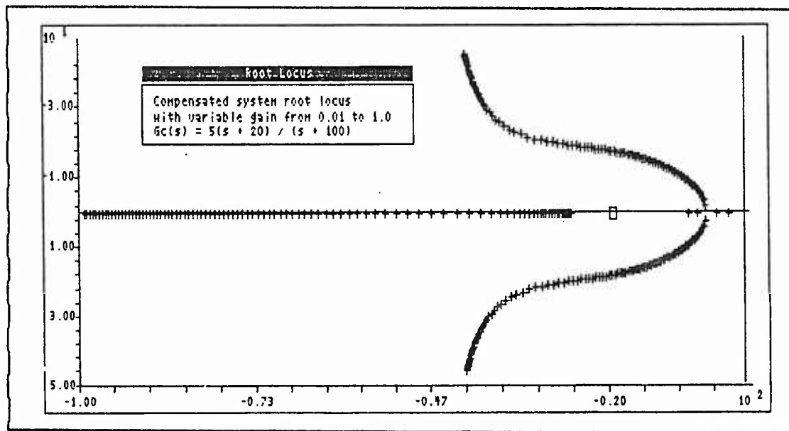
Figure 2-19. Compensated System Root Locus
