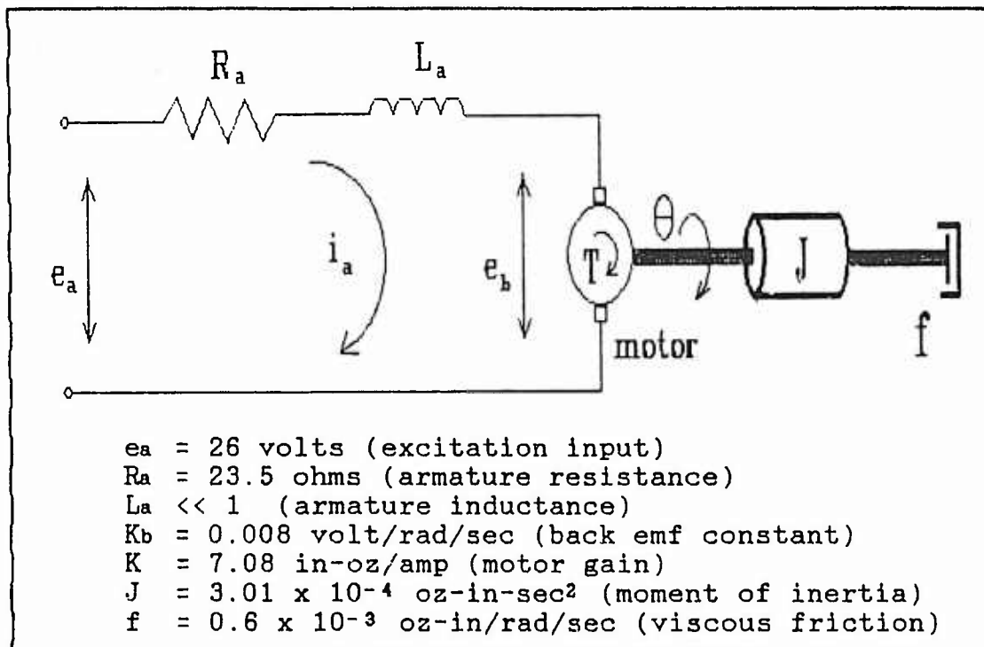
Figure 2-1. Schematic Diagram of the Armature Controlled DC Motor
