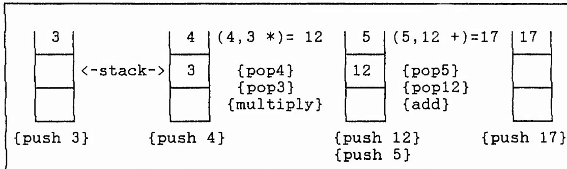
Figure 3-20. Stack Operation Example
