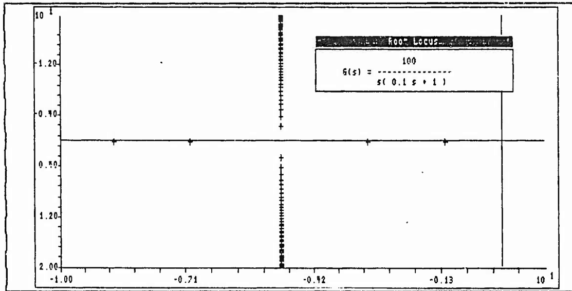
Figure 2-14. DC Motor Root Locus Diagram
