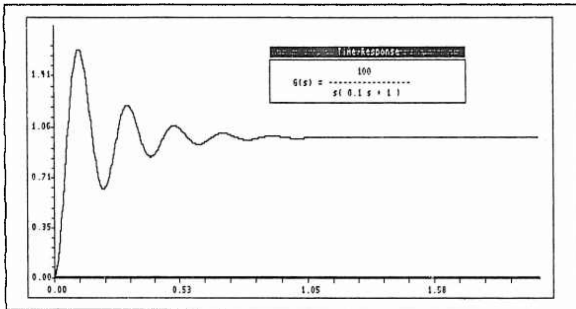
Figure 2-16. DC Motor Step Response
