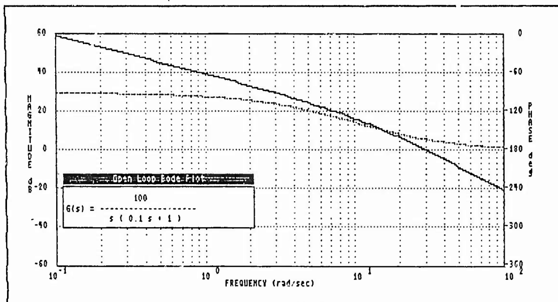
Figure 2-12. DC Motor Open-Loop Bode Diagram
