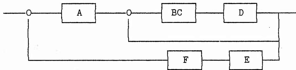
Figure 3-11b. Reduced BC Loop
