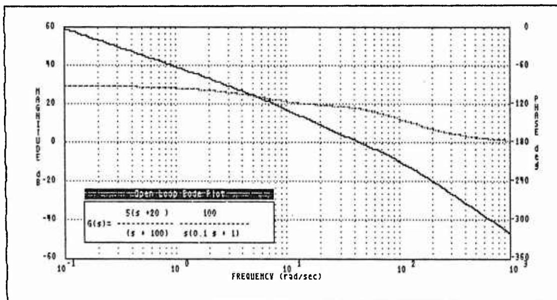
Figure 2-18. Compensated Open-Loop Bode Plot
