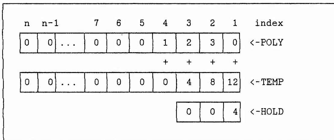
Figure 3-7. Array Contents After Third-Factor Operation
