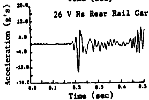
Figure 24. Vertical accelerations along road side of rail car.
