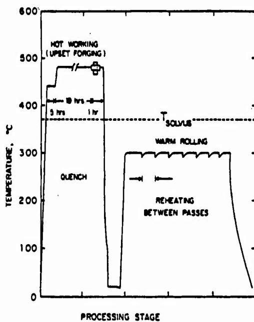
Figure 2.2 Schematic of the thermomechanical processing technique.
