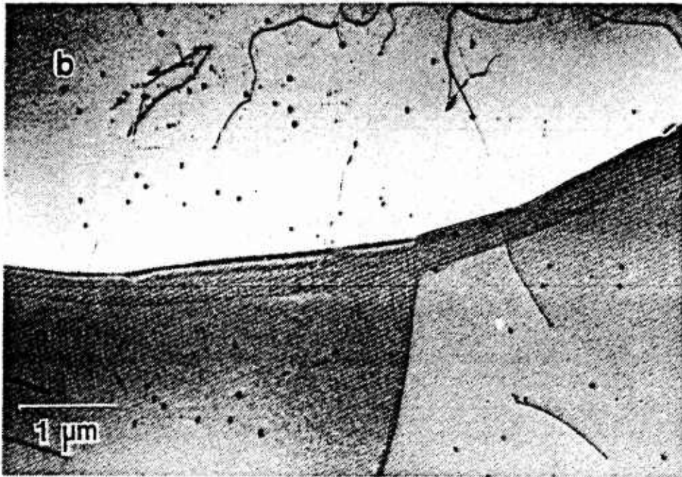
Figure 4.3 TEM micrograph of Al-10Mg-0.1Zr heated to 733K: (a) Heavy reduction material, (b) Light reduction material.
