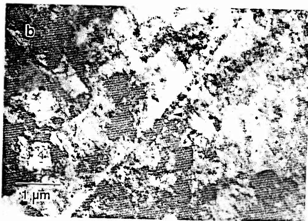
Figure 4.9 TEM micrograph of Al-10Mg-0.1Zr in as rolled condition: (a) Light reduction, (b) Heavy reduction. Arrows indicate \beta on prior grain boundary.
