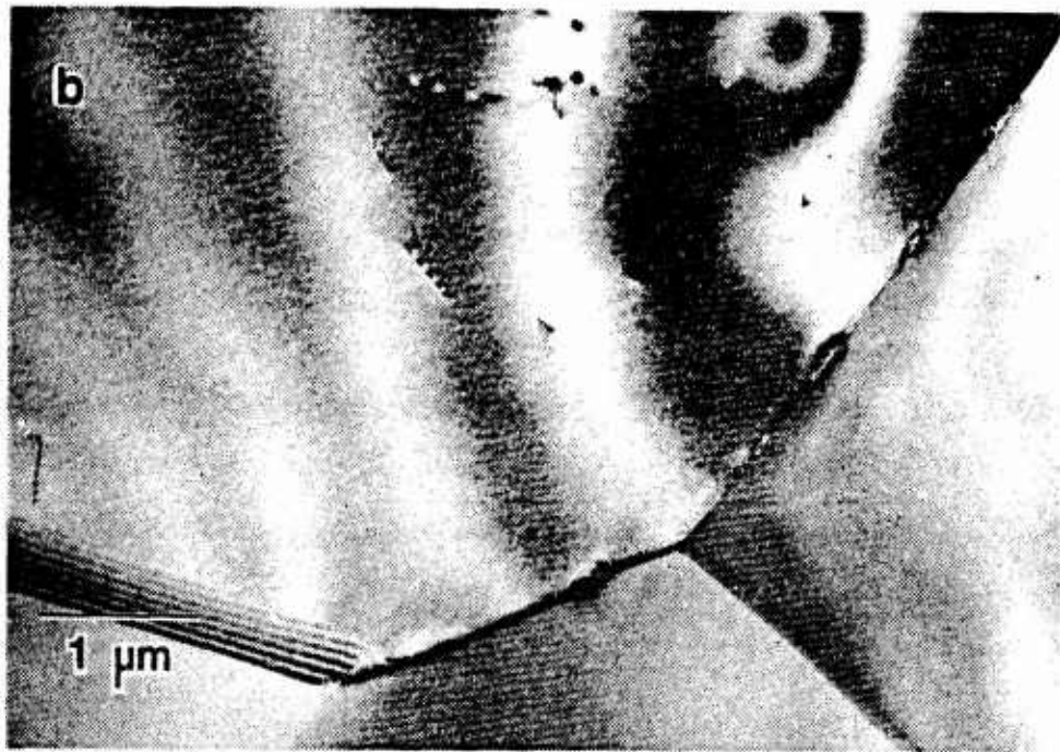
Figure 4.19 TEM micrographs of lightly reduced and annealed for 1.5 hrs at 573K: (a) Heated to 633K and cooled to 295K (b) Heated to 723K and cooled to 295K.
