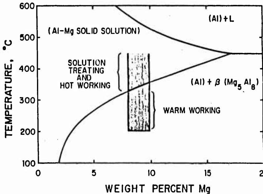
Figure 2.1 Aluminum-Magnesium phase diagram with TMP region indicated.
