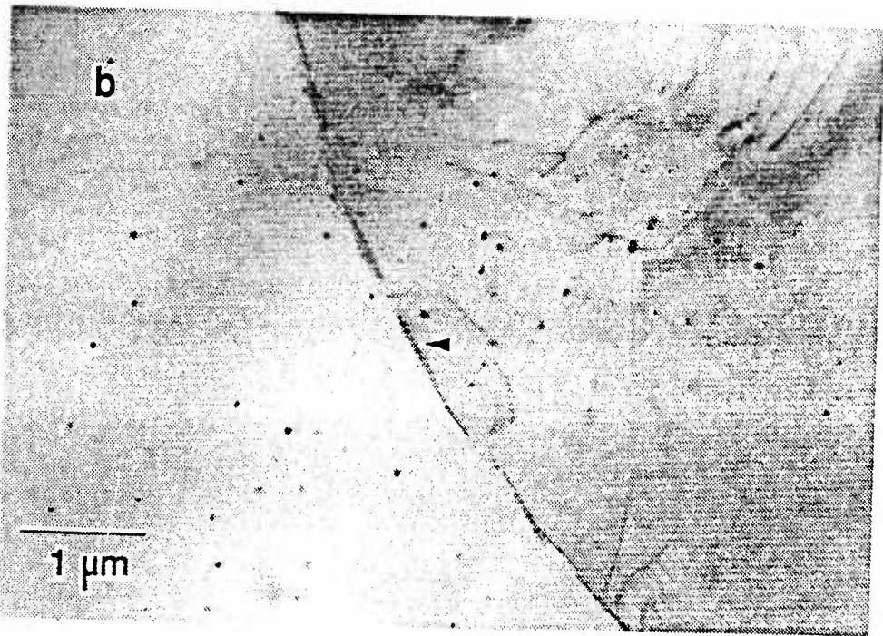
Figure 4.15 TEM micrograph of Al-10Mg-0.1Zr 723K scan: (a) Heavy reduction - recrystallized grain interior (b) Light reduction - \beta remnants from prior grain boundary.
